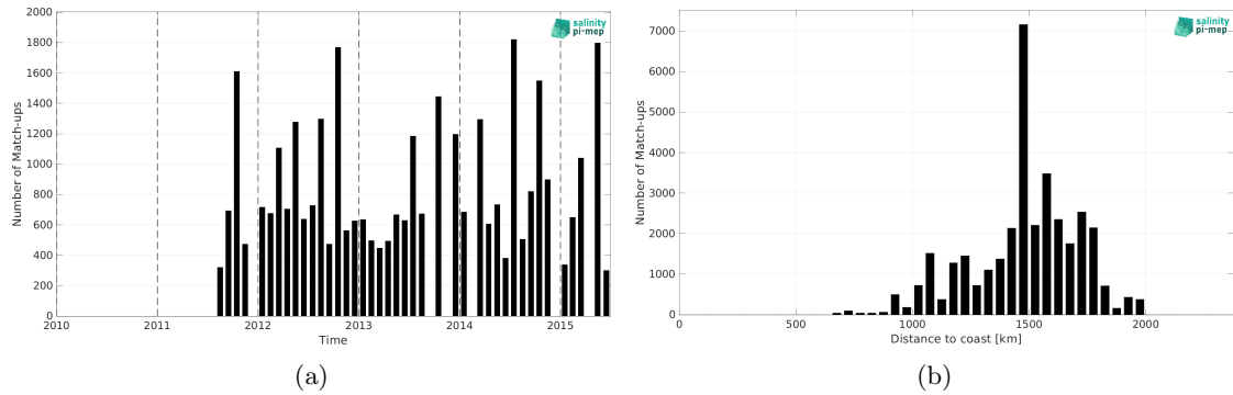
Figure 2: Number of match-ups between TSG (LEGOS-DM) and Aquarius SSS L3 CAP v5 - 7-Day running (JPL) SSS as a function of time (a) and as function of the distance to coast (b) over the SPURS 1 Pi-MEP region and for the full satellite product period.
