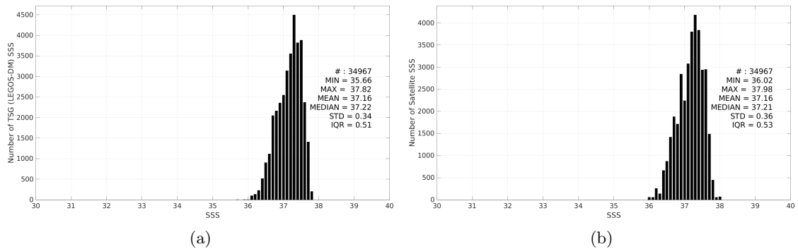
Figure 3: Histograms of SSS from TSG (LEGOS-DM) (a) and Aquarius SSS L3 CAP v5 - 7-Day running (JPL) (b) considering all match-up pairs per bins of 0.1 over the SPURS 1 Pi-MEP region and for the full satellite product period.
