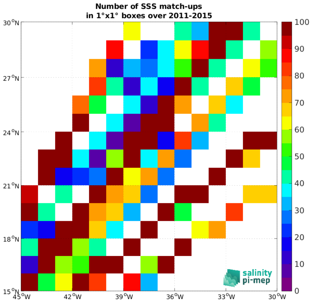
Figure 5: Number of SSS match-ups between TSG (LEGOS-DM) SSS and the Aquarius SSS L3 CAP v5 - 7-Day running (JPL) SSS product for the SPURS 1 Pi-MEP region over 1^\circ \times 1^\circ boxes and for the full satellite product period.
