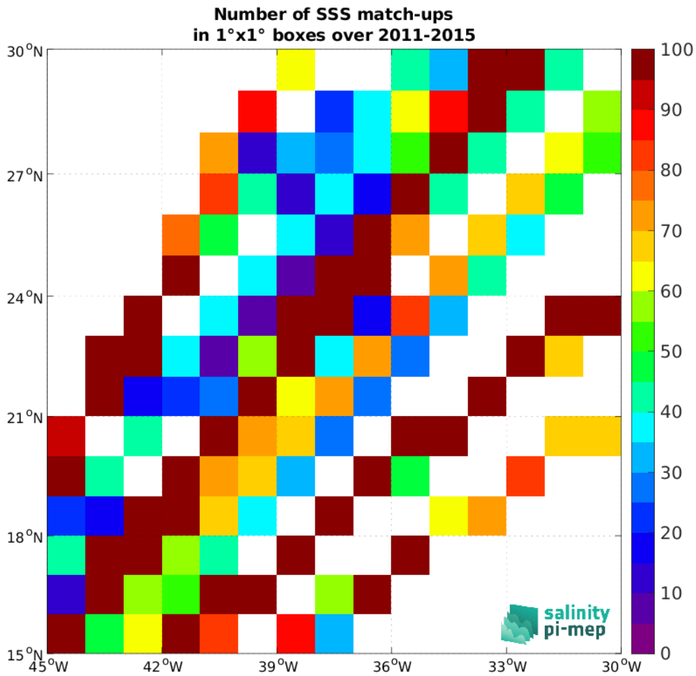
Figure 5: Number of SSS match-ups between TSG (LEGOS-DM) SSS and the Aquarius SSS L3 CAP v5 - 7-Day running (JPL) SSS product for the SPURS 1 Pi-MEP region over 1°x1° boxes and for the full satellite product period.
