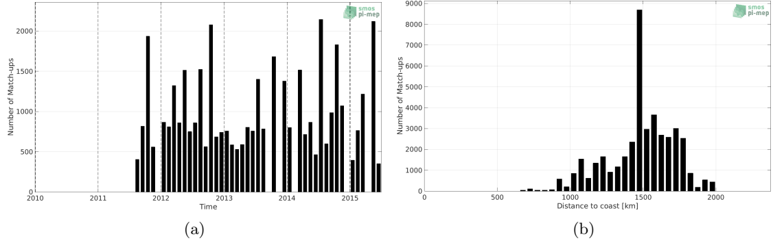
Figure 1: Number of match-ups between TSG (LEGOS-DM) and Aquarius SSS L3 CAP v5 - 7-Day running (JPL) SSS as a function of time (a) and as function of the distance to coast (b) over the SPURS 1 Pi-MEP region and for the full satellite product period.
