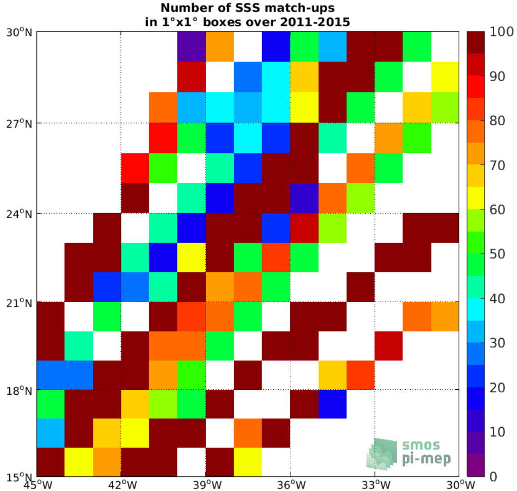
Figure 4: Number of SSS match-ups between TSG (LEGOS-DM) SSS and the Aquarius SSS L3 CAP v5 - 7-Day running (JPL) SSS product for the SPURS 1 Pi-MEP region over 1°x1° boxes and for the full satellite product period.
