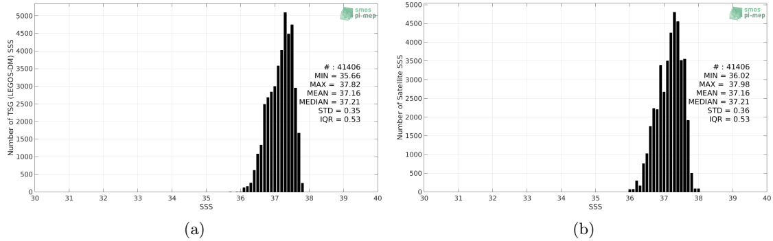
Figure 2: Histograms of SSS from TSG (LEGOS-DM) (a) and Aquarius SSS L3 CAP v5 - 7-Day running (JPL) (b) considering all match-up pairs per bins of 0.1 over the SPURS 1 Pi-MEP region and for the full satellite product period.
