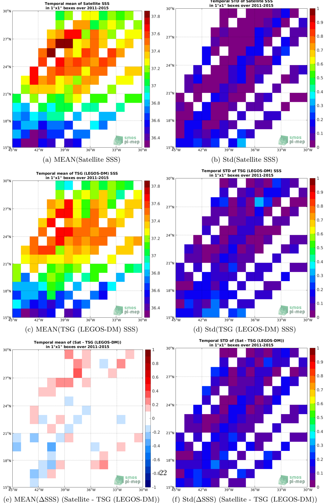
Figure 6: Temporal mean (left) and Std (right) of SSS from Aquarius SSS L3 CAP v5 - 7-Day running (JPL) (top), TSG (LEGOS-DM) (middle), and of \Delta SSS (Satellite - TSG (LEGOS-DM)). Only match-up pairs are used to generate these maps.
