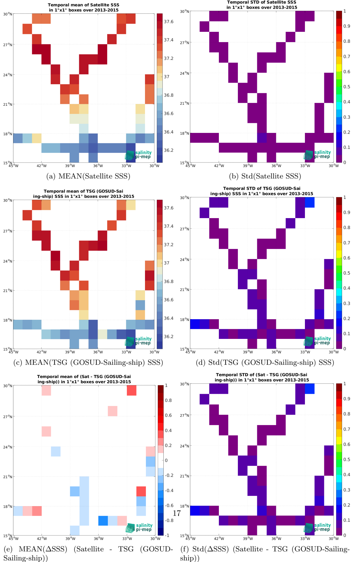
Figure 7: Temporal mean (left) and Std (right) of SSS from Aquarius SSS L3 CAP v5 - 7-Day running (JPL) (top), TSG (GOSUD-Sailing-ship) (middle), and of \Delta SSS (Satellite - TSG (GOSUD-Sailing-ship)). Only match-up pairs are used to generate these maps.
