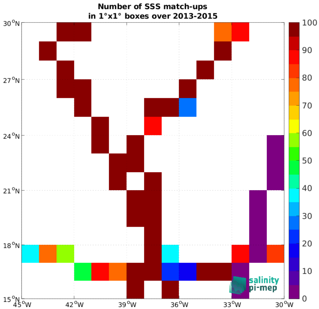
Figure 5: Number of SSS match-ups between TSG (GOSUD-Sailing-ship) SSS and the Aquarius SSS L3 CAP v5 - 7-Day running (JPL) SSS product for the SPURS 1 Pi-MEP region over 1^\circ \times 1^\circ boxes and for the full satellite product period.
