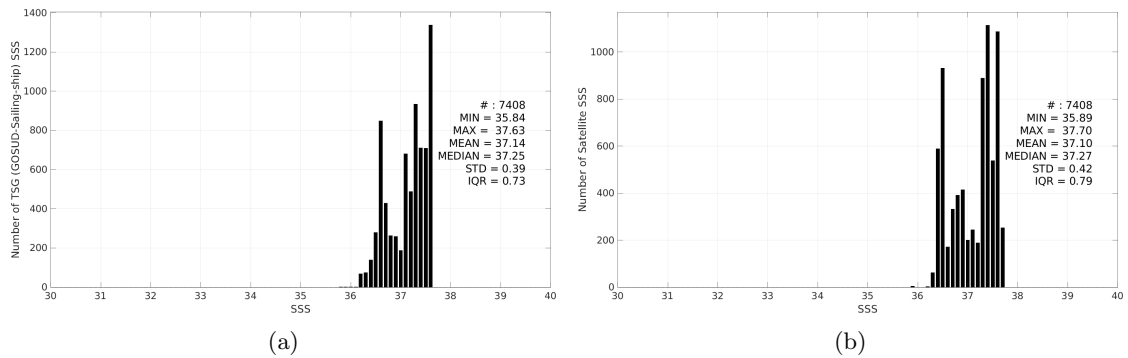
Figure 3: Histograms of SSS from TSG (GOSUD-Sailing-ship) (a) and Aquarius SSS L3 CAP v5 - 7-Day running (JPL) (b) considering all match-up pairs per bins of 0.1 over the SPURS 1 Pi-MEP region and for the full satellite product period.
