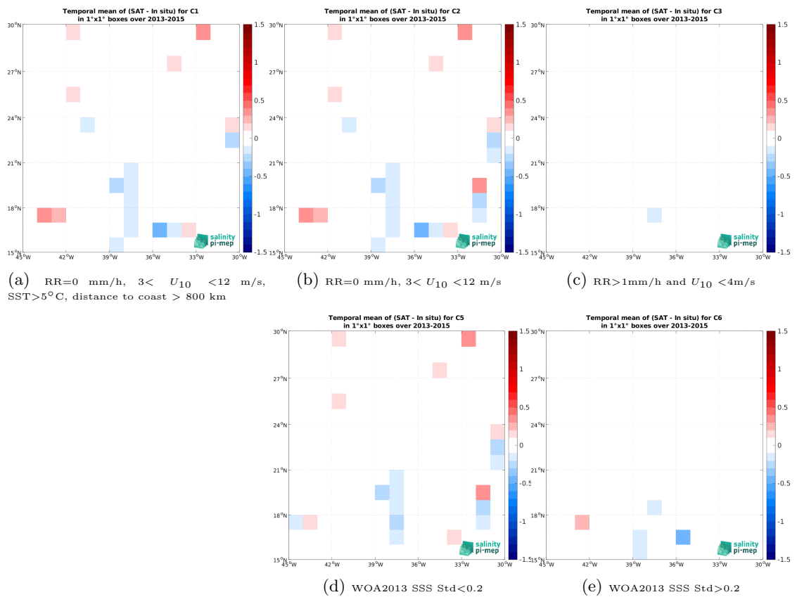
Figure 14: Temporal mean gridded over spatial boxes of size 1^\circ \times 1^\circ of \Delta SSS (Aquarius SSS L3 CAP v5 - 7-Day running (JPL) - TSG (GOSUD-Sailing-ship)) for 5 different subdatasets corresponding to:RR=0 mm/h, 3 < U_{10} < 12 m/s, SST >5^\circ C, distance to coast > 800 km (a), RR=0 mm/h, 3 < U_{10} < 12 m/s (b), RR >1 mm/h and U_{10} < 4 m/s (c), WOA2013 SSS Std <0.2 (d), WOA2013 SSS Std >0.2 (e).
