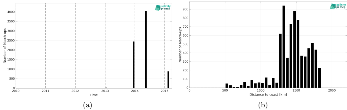
Figure 2: Number of match-ups between TSG (GOSUD-Sailing-ship) and Aquarius SSS L3 CAP v5 - 7-Day running (JPL) SSS as a function of time (a) and as function of the distance to coast (b) over the SPURS 1 Pi-MEP region and for the full satellite product period.
