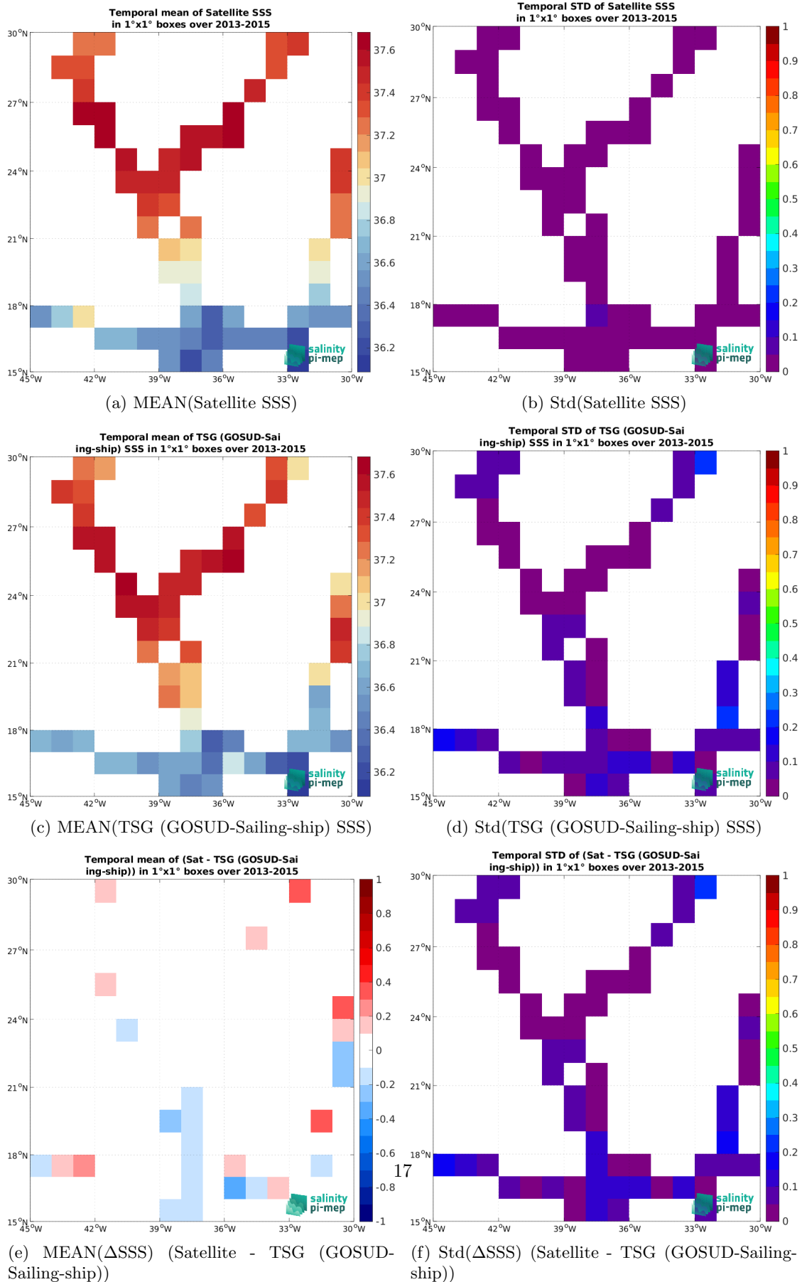
Figure 6: Temporal mean (left) and Std (right) of SSS from Aquarius SSS L3 CAP v5 - 7-Day running (JPL) (top), TSG (GOSUD-Sailing-ship) (middle), and of \Delta SSS (Satellite - TSG (GOSUD-Sailing-ship)). Only match-up pairs are used to generate these maps.
