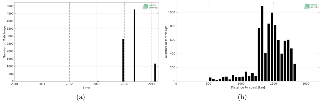
Figure 1: Number of match-ups between TSG (GOSUD-Sailing-ship) and Aquarius SSS L3 CAP v5 - 7-Day running (JPL) SSS as a function of time (a) and as function of the distance to coast (b) over the SPURS 1 Pi-MEP region and for the full satellite product period.
