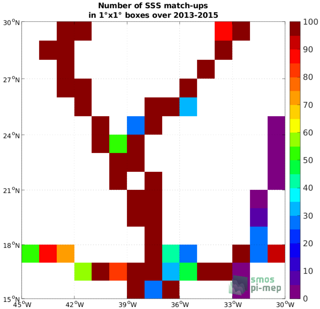
Figure 4: Number of SSS match-ups between TSG (GOSUD-Sailing-ship) SSS and the Aquarius SSS L3 CAP v5 - 7-Day running (JPL) SSS product for the SPURS 1 Pi-MEP region over 1°x1° boxes and for the full satellite product period.
