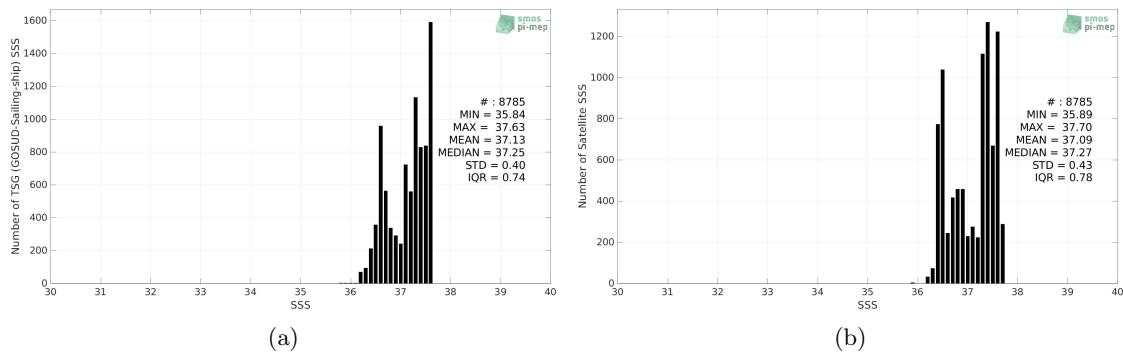
Figure 2: Histograms of SSS from TSG (GOSUD-Sailing-ship) (a) and Aquarius SSS L3 CAP v5 - 7-Day running (JPL) (b) considering all match-up pairs per bins of 0.1 over the SPURS 1 Pi-MEP region and for the full satellite product period.
