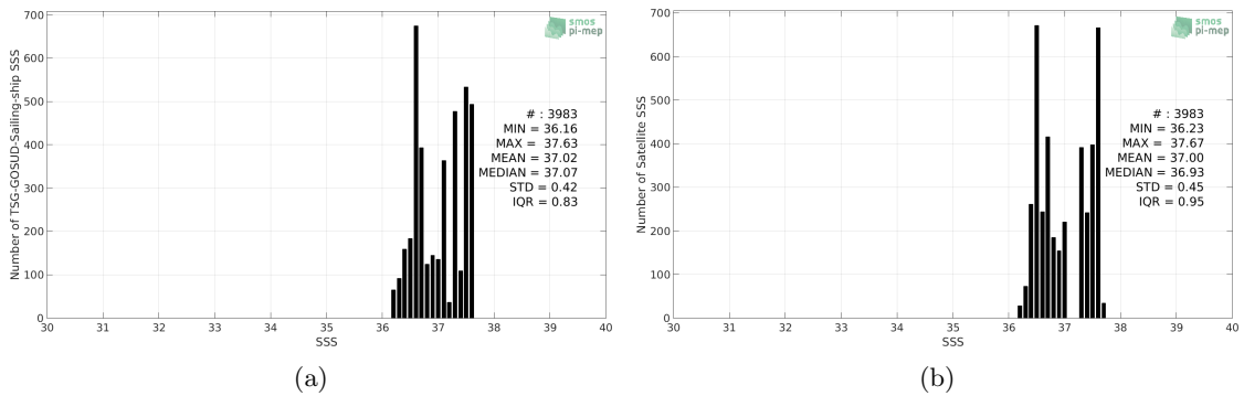
Figure 2: Histograms of SSS from TSG-GOSUD-Sailing-ship (a) and Aquarius-L3-JPL-V5-7DAY-RUNNING (b) considering all match-up pairs per bins of 0.1 over the SPURS 1 Pi-MEP region and for the full satellite product period.
