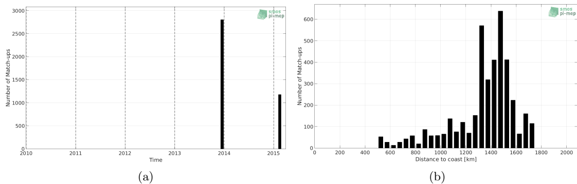
Figure 1: Number of match-ups between TSG-GOSUD-Sailing-ship and Aquarius-L3-JPL-V5-7DAY-RUNNING SSS as a function of time (a) and as function of the distance to coast (b) over the SPURS 1 Pi-MEP region and for the full satellite product period.
