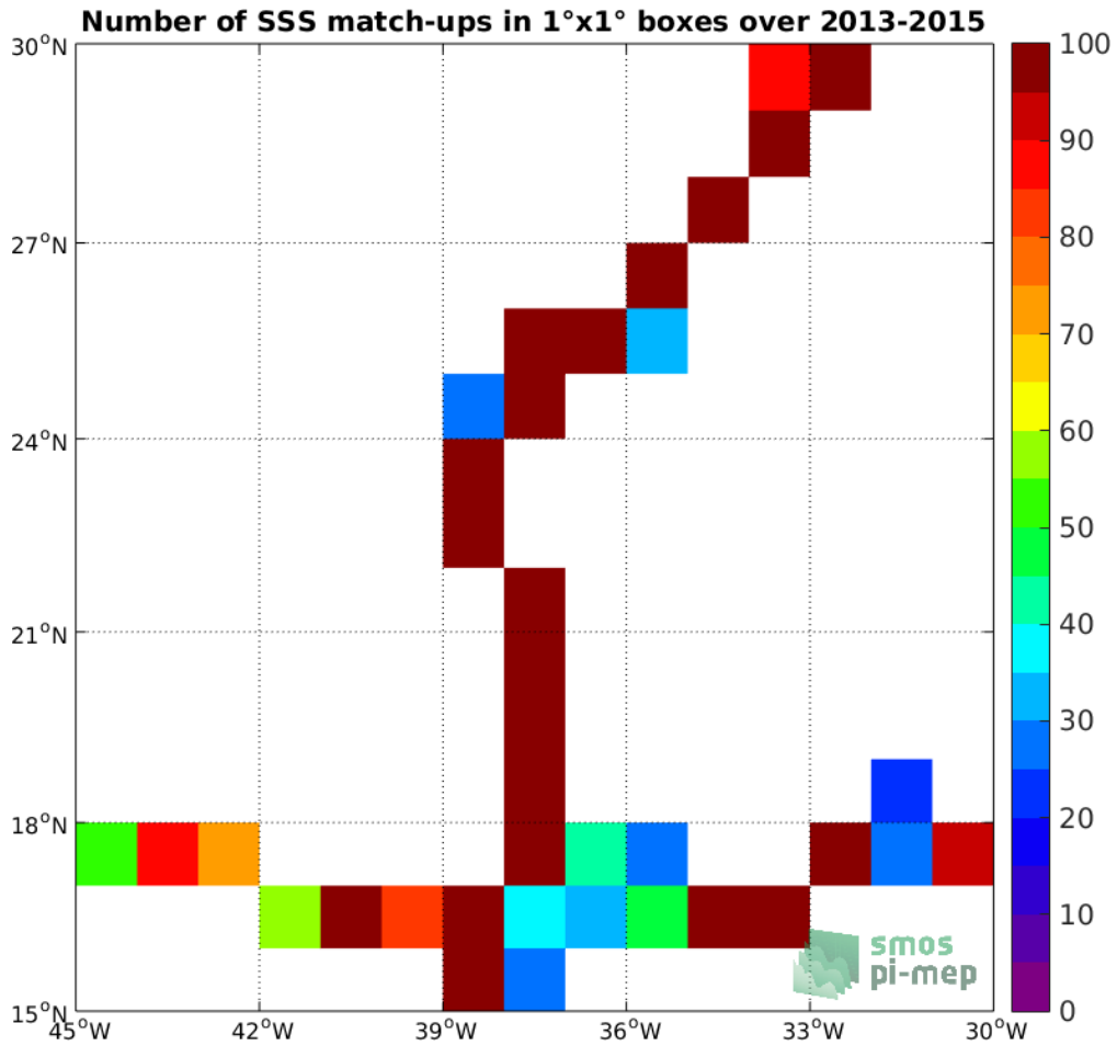
Figure 4: Number of SSS match-ups between TSG-GOSUD-Sailing-ship SSS and the Aquarius-L3-JPL-V5-7DAY-RUNNING SSS product for the SPURS 1 Pi-MEP region over 1°x1° boxes and for the full satellite product period.
