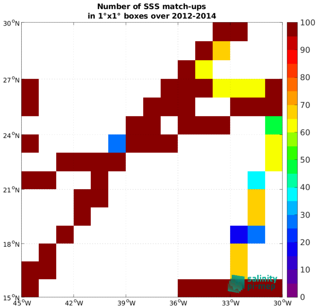
Figure 4: Number of SSS match-ups between TSG (GOSUD-Research-vessel) SSS and the Aquarius SSS L3 CAP v5 - 7-Day running (JPL) SSS product for the SPURS 1 Pi-MEP region over 1^\circ \times 1^\circ boxes and for the full satellite product period.
