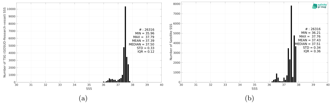
Figure 2: Histograms of SSS from TSG (GOSUD-Research-vessel) (a) and Aquarius SSS L3 CAP v5 - 7-Day running (JPL) (b) considering all match-up pairs per bins of 0.1 over the SPURS 1 Pi-MEP region and for the full satellite product period.
