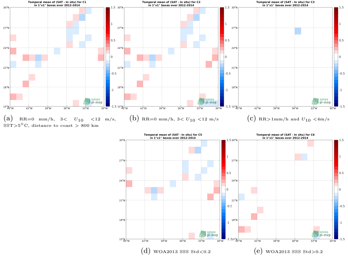
Figure 12: Temporal mean gridded over spatial boxes of size 1^\circ \times 1^\circ of \Delta\text{SSS} (Aquarius SSS L3 CAP v5 - 7-Day running (JPL) - TSG (GOSUD-Research-vessel)) for 5 different subdatasets corresponding to: RR=0 mm/h, 3 < U_{10} < 12 m/s, SST > 5^\circ\text{C} , distance to coast > 800 km (a), RR=0 mm/h, 3 < U_{10} < 12 m/s (b), RR > 1\text{mm/h} and U_{10} < 4\text{m/s} (c), WOA2013 SSS Std < 0.2 (d), WOA2013 SSS Std > 0.2 (e).
