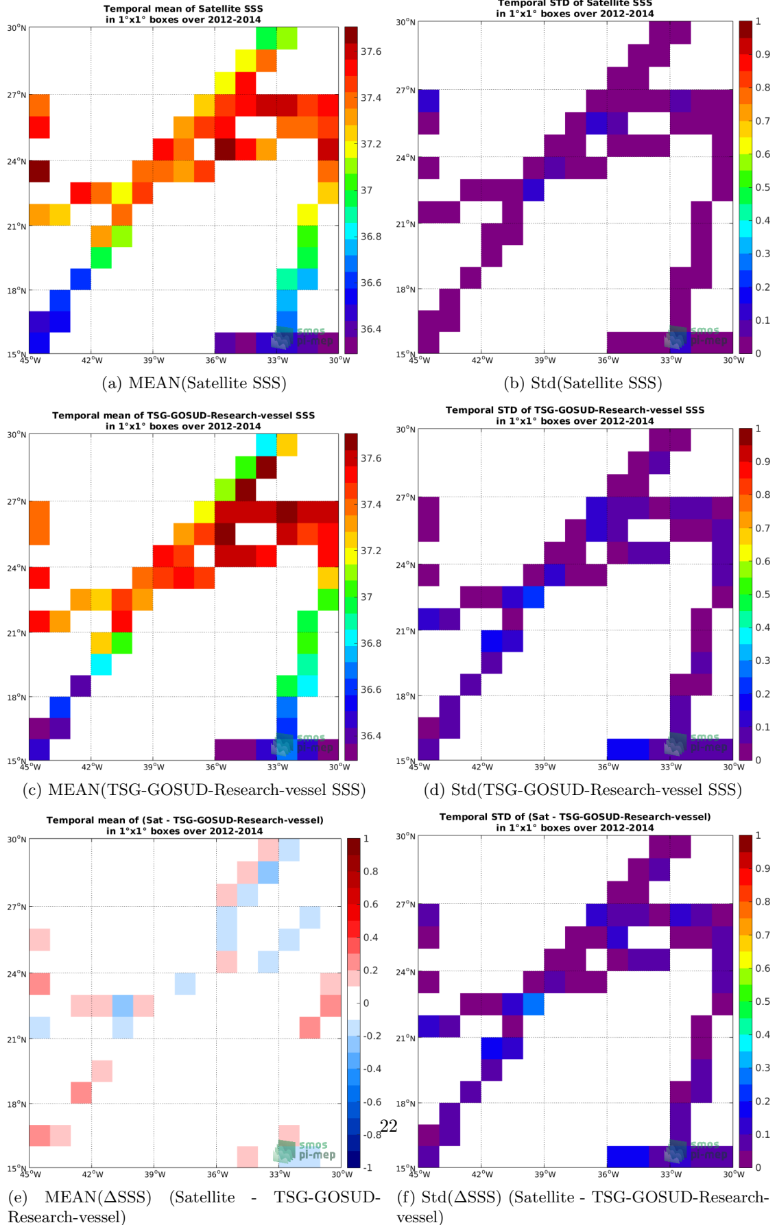
Figure 6: Temporal mean (left) and Std (right) of SSS from Aquarius-L3-JPL-V5-7DAY-RUNNING (top), TSG-GOSUD-Research-vessel (middle), and of \Delta SSS (Satellite - TSG-GOSUD-Research-vessel). Only match-up pairs are used to generate these maps.
