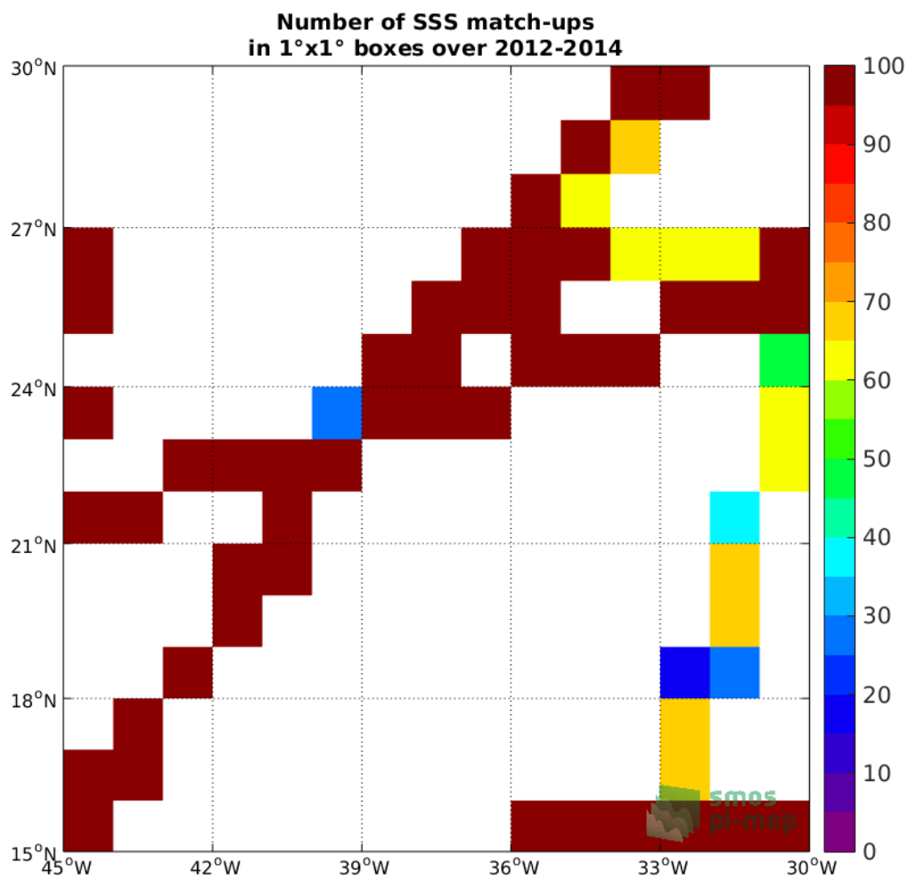
Figure 4: Number of SSS match-ups between TSG-GOSUD-Research-vessel SSS and the Aquarius-L3-JPL-V5-7DAY-RUNNING SSS product for the SPURS 1 Pi-MEP region over 1°x1° boxes and for the full satellite product period.
