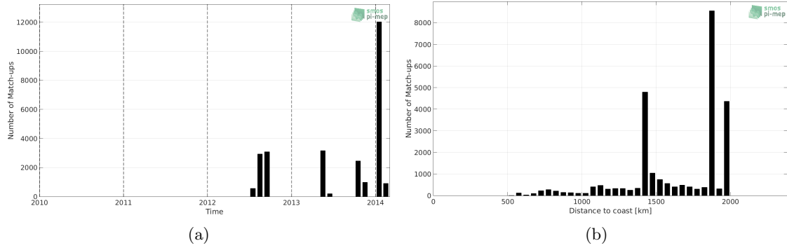
Figure 1: Number of match-ups between TSG-GOSUD-Research-vessel and Aquarius-L3-JPL-V5-7DAY-RUNNING SSS as a function of time (a) and as function of the distance to coast (b) over the SPURS 1 Pi-MEP region and for the full satellite product period.
