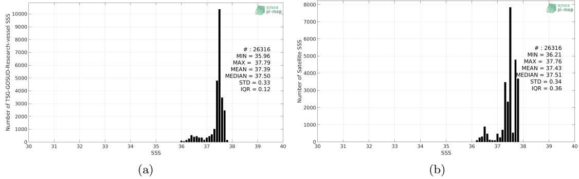
Figure 2: Histograms of SSS from TSG-GOSUD-Research-vessel (a) and Aquarius-L3-JPL-V5-7DAY-RUNNING (b) considering all match-up pairs per bins of 0.1 over the SPURS 1 Pi-MEP region and for the full satellite product period.
