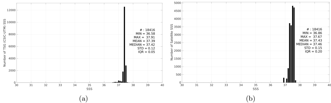
Figure 3: Histograms of SSS from TSG (CSIC-UTM) (a) and Aquarius SSS L3 CAP v5 - 7-Day running (JPL) (b) considering all match-up pairs per bins of 0.1 over the SPURS 1 Pi-MEP region and for the full satellite product period.
