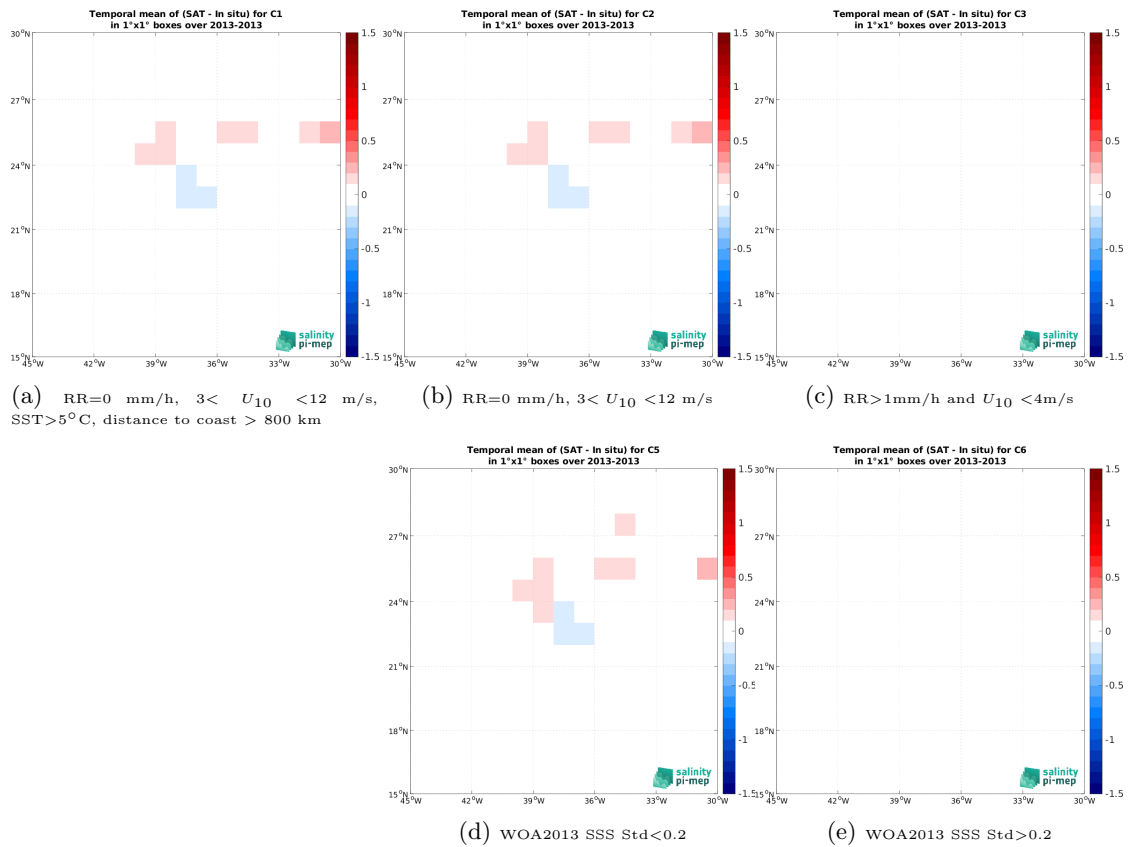
Figure 14: Temporal mean gridded over spatial boxes of size 1^\circ \times 1^\circ of \Delta SSS (Aquarius SSS L3 CAP v5 - 7-Day running (JPL) - TSG (CSIC-UTM)) for 5 different subdatasets corresponding to:RR=0 mm/h, 3 < U_{10} < 12 m/s, SST >5^\circ C, distance to coast > 800 km (a), RR=0 mm/h, 3 < U_{10} < 12 m/s (b), RR >1 mm/h and U_{10} < 4 m/s (c), WOA2013 SSS Std <0.2 (d), WOA2013 SSS Std >0.2 (e).
