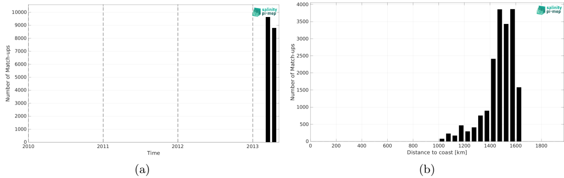
Figure 2: Number of match-ups between TSG (CSIC-UTM) and Aquarius SSS L3 CAP v5 - 7-Day running (JPL) SSS as a function of time (a) and as function of the distance to coast (b) over the SPURS 1 Pi-MEP region and for the full satellite product period.
