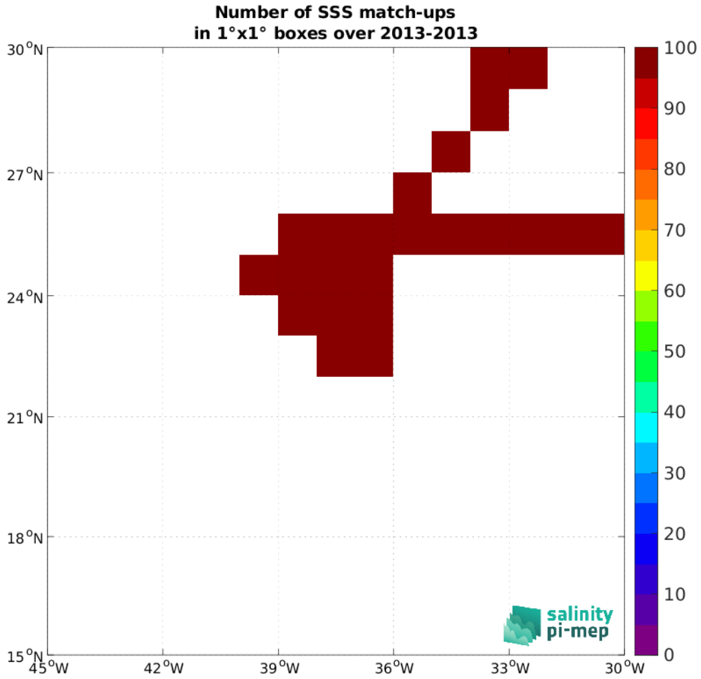
Figure 4: Number of SSS match-ups between TSG (CSIC-UTM) SSS and the Aquarius SSS L3 CAP v5 - 7-Day running (JPL) SSS product for the SPURS 1 Pi-MEP region over 1°x1° boxes and for the full satellite product period.
