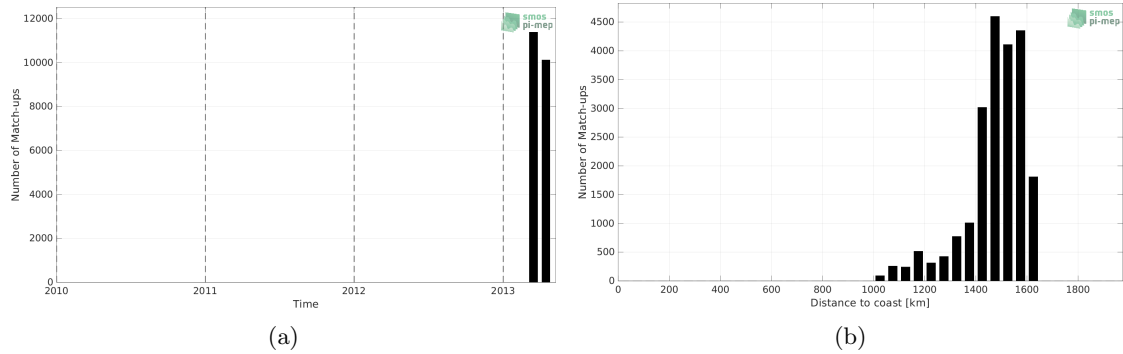
Figure 1: Number of match-ups between TSG (CSIC-UTM) and Aquarius SSS L3 CAP v5 - 7-Day running (JPL) SSS as a function of time (a) and as function of the distance to coast (b) over the SPURS 1 Pi-MEP region and for the full satellite product period.
