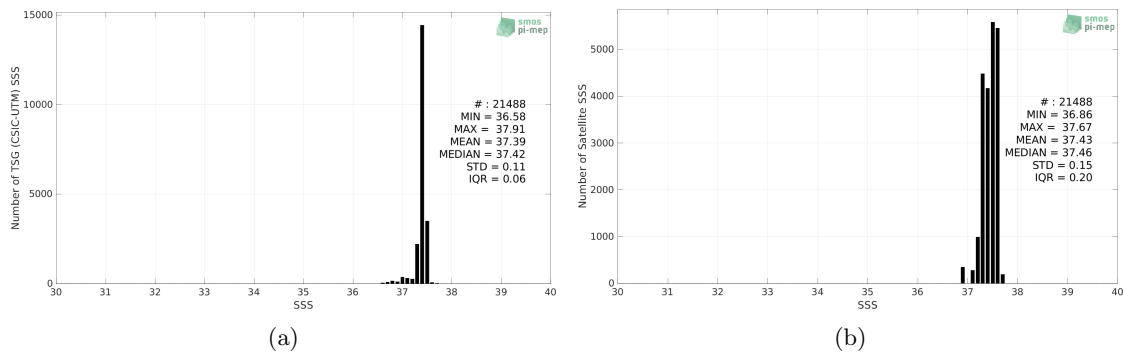
Figure 2: Histograms of SSS from TSG (CSIC-UTM) (a) and Aquarius SSS L3 CAP v5 - 7-Day running (JPL) (b) considering all match-up pairs per bins of 0.1 over the SPURS 1 Pi-MEP region and for the full satellite product period.
