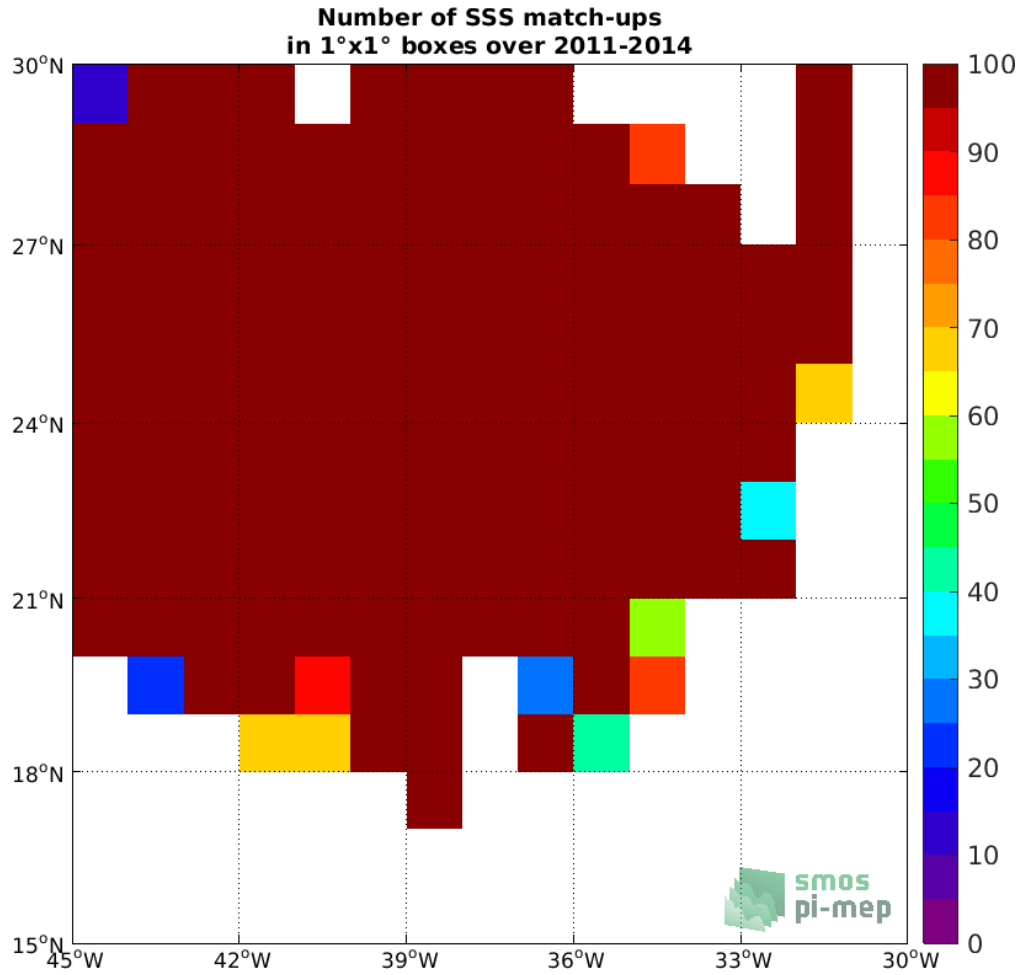
Figure 3: Number of SSS match-ups between Surface drifters SSS and the Aquarius SSS L3 CAP v5 - 7-Day running (JPL) SSS product for the SPURS 1 Pi-MEP region over 1°x1° boxes and for the full satellite product period.
