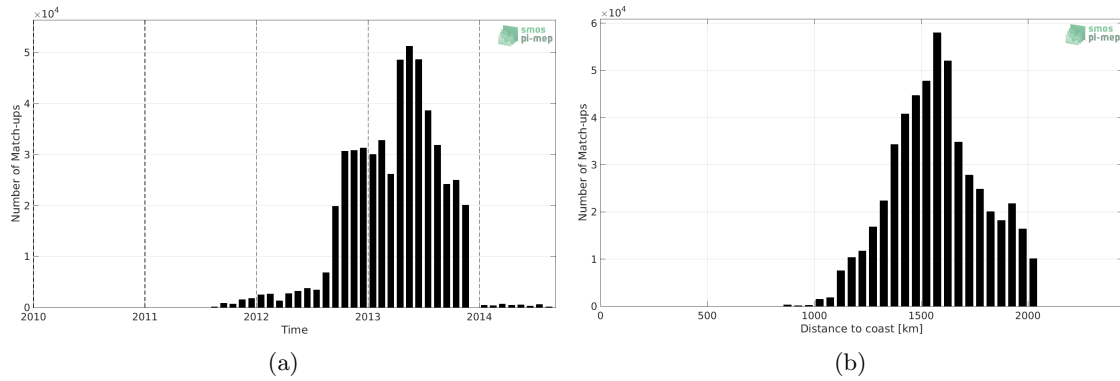
Figure 1: Number of match-ups between Surface drifters and Aquarius SSS L3 CAP v5 - 7-Day running (JPL) SSS as a function of time (a) and as function of the distance to coast (b) over the SPURS 1 Pi-MEP region and for the full satellite product period.
