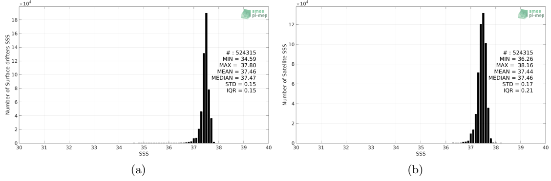
Figure 2: Histograms of SSS from Surface drifters (a) and Aquarius SSS L3 CAP v5 - 7-Day running (JPL) (b) considering all match-up pairs per bins of 0.1 over the SPURS 1 Pi-MEP region and for the full satellite product period.
