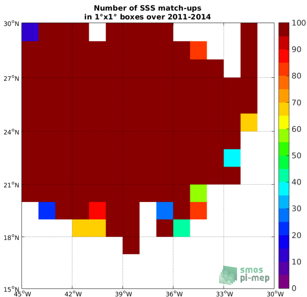
Figure 3: Number of SSS match-ups between Surface drifters SSS and the Aquarius-L3-JPL-V5-7DAY-RUNNING SSS product for the SPURS 1 Pi-MEP region over 1°x1° boxes and for the full satellite product period.
