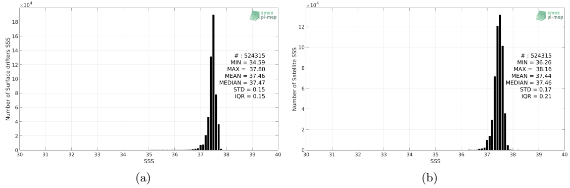
Figure 2: Histograms of SSS from Surface drifters (a) and Aquarius-L3-JPL-V5-7DAY-RUNNING (b) considering all match-up pairs per bins of 0.1 over the SPURS 1 Pi-MEP region and for the full satellite product period.
