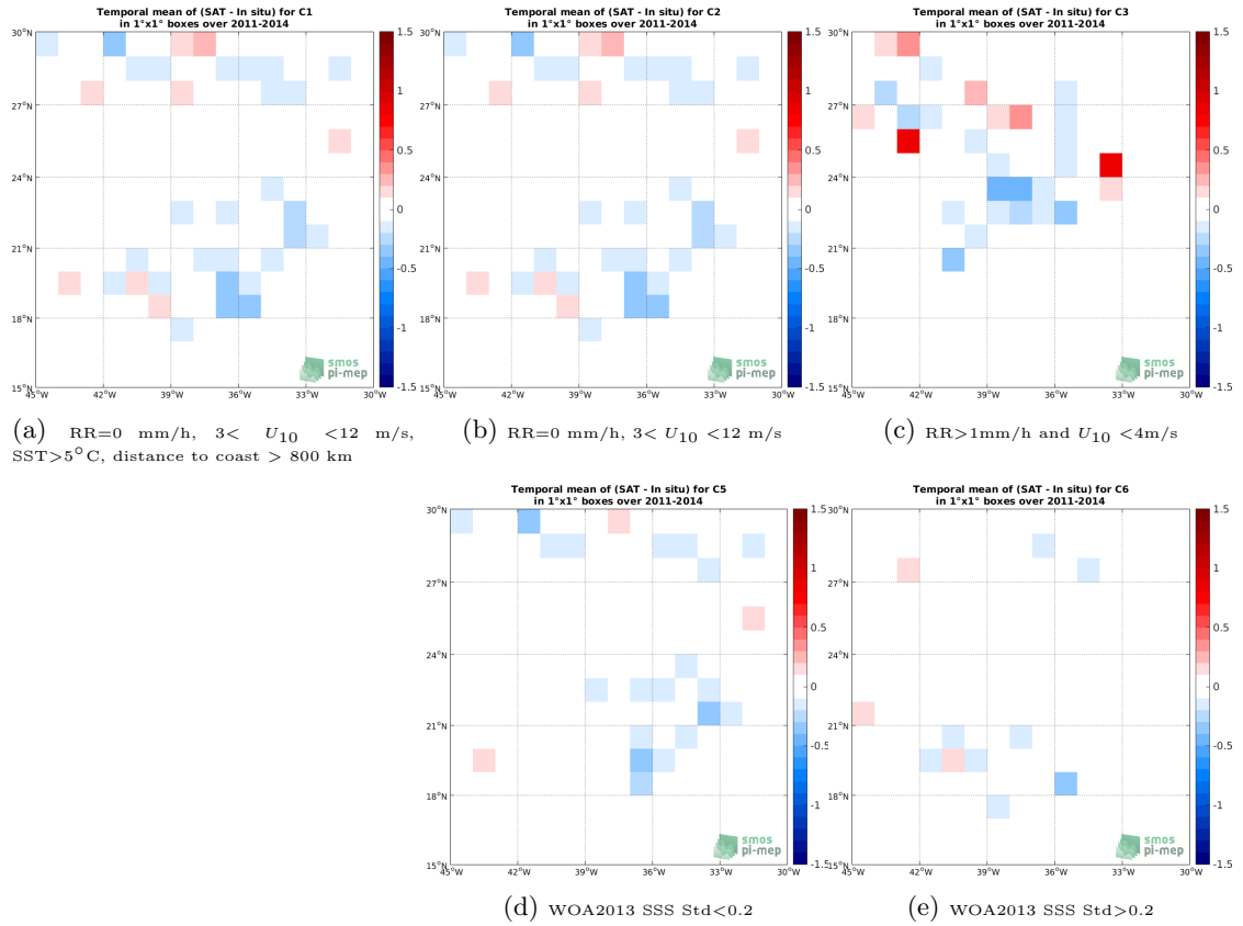
Figure 11: Temporal mean gridded over spatial boxes of size 1^\circ \times 1^\circ of \Delta SSS (Aquarius-L3-JPL-V5-7DAY-RUNNING - Surface drifters) for 5 different subdatasets corresponding to:RR=0 mm/h, 3 < U_{10} < 12 m/s, SST >5^\circ C, distance to coast > 800 km (a), RR=0 mm/h, 3 < U_{10} < 12 m/s (b), RR >1 mm/h and U_{10} < 4 m/s (c), WOA2013 SSS Std <0.2 (d), WOA2013 SSS Std >0.2 (e).
