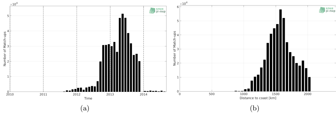
Figure 1: Number of match-ups between Surface drifters and Aquarius-L3-JPL-V5-7DAY-RUNNING SSS as a function of time (a) and as function of the distance to coast (b) over the SPURS 1 Pi-MEP region and for the full satellite product period.
