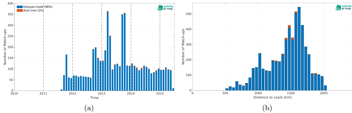
Figure 2: Number of match-ups between Argo and Aquarius SSS L3 CAP v5 - 7-Day running (JPL) SSS as a function of time (a) and as function of the distance to coast (b) over the SPURS 1 Pi-MEP region and for the full satellite product period.
