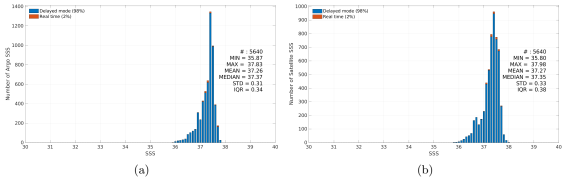
Figure 3: Histograms of SSS from Argo (a) and Aquarius SSS L3 CAP v5 - 7-Day running (JPL) (b) considering all match-up pairs per bins of 0.1 over the SPURS 1 Pi-MEP region and for the full satellite product period.
