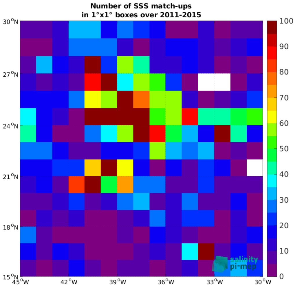
Figure 5: Number of SSS match-ups between Argo SSS and the Aquarius SSS L3 CAP v5 - 7-Day running (JPL) SSS product for the SPURS 1 Pi-MEP region over 1^{\circ}\times 1^{\circ} boxes and for the full satellite product period.
