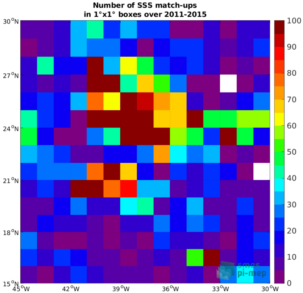
Figure 4: Number of SSS match-ups between Argo SSS and the Aquarius SSS L3 CAP v5 - 7-Day running (JPL) SSS product for the SPURS 1 Pi-MEP region over 1°x1° boxes and for the full satellite product period.
