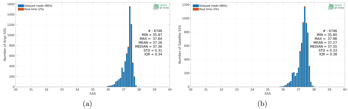
Figure 2: Histograms of SSS from Argo (a) and Aquarius SSS L3 CAP v5 - 7-Day running (JPL) (b) considering all match-up pairs per bins of 0.1 over the SPURS 1 Pi-MEP region and for the full satellite product period.
