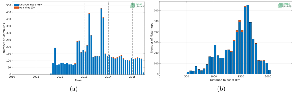
Figure 1: Number of match-ups between Argo and Aquarius SSS L3 CAP v5 - 7-Day running (JPL) SSS as a function of time (a) and as function of the distance to coast (b) over the SPURS 1 Pi-MEP region and for the full satellite product period.
