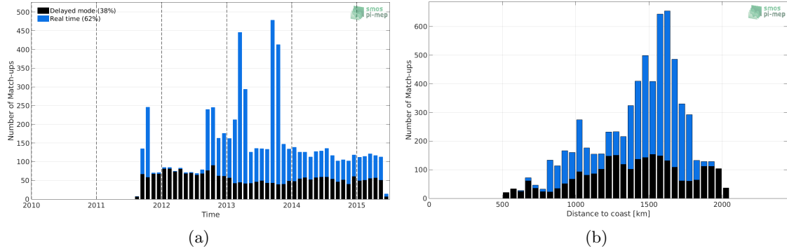
Figure 1: Number of match-ups between Argo and Aquarius-L3-JPL-V5-7DAY-RUNNING SSS as a function of time (a) and as function of the distance to coast (b) over the SPURS 1 Pi-MEP region and for the full satellite product period.
