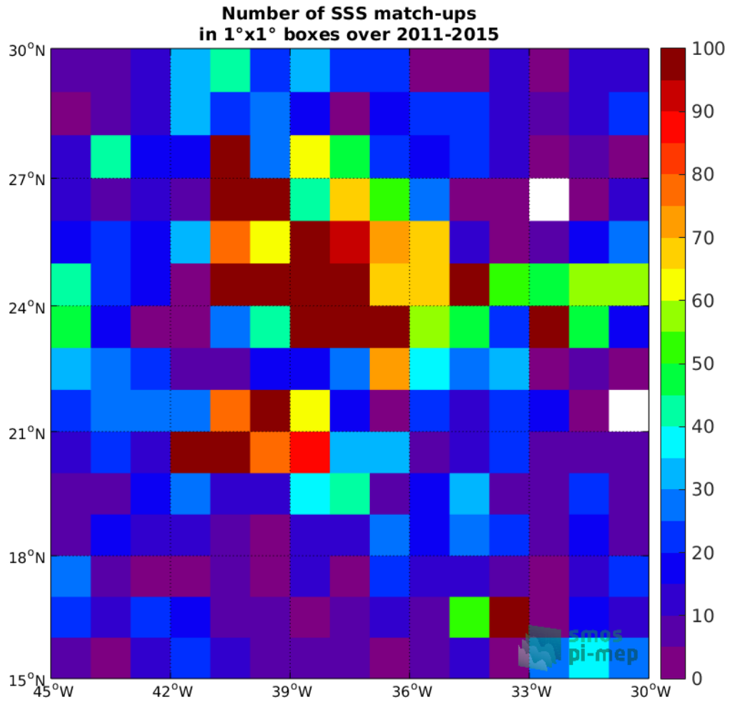
Figure 4: Number of SSS match-ups between Argo SSS and the Aquarius-L3-JPL-V5-7DAY-RUNNING SSS product for the SPURS 1 Pi-MEP region over 1°x1° boxes and for the full satellite product period.
