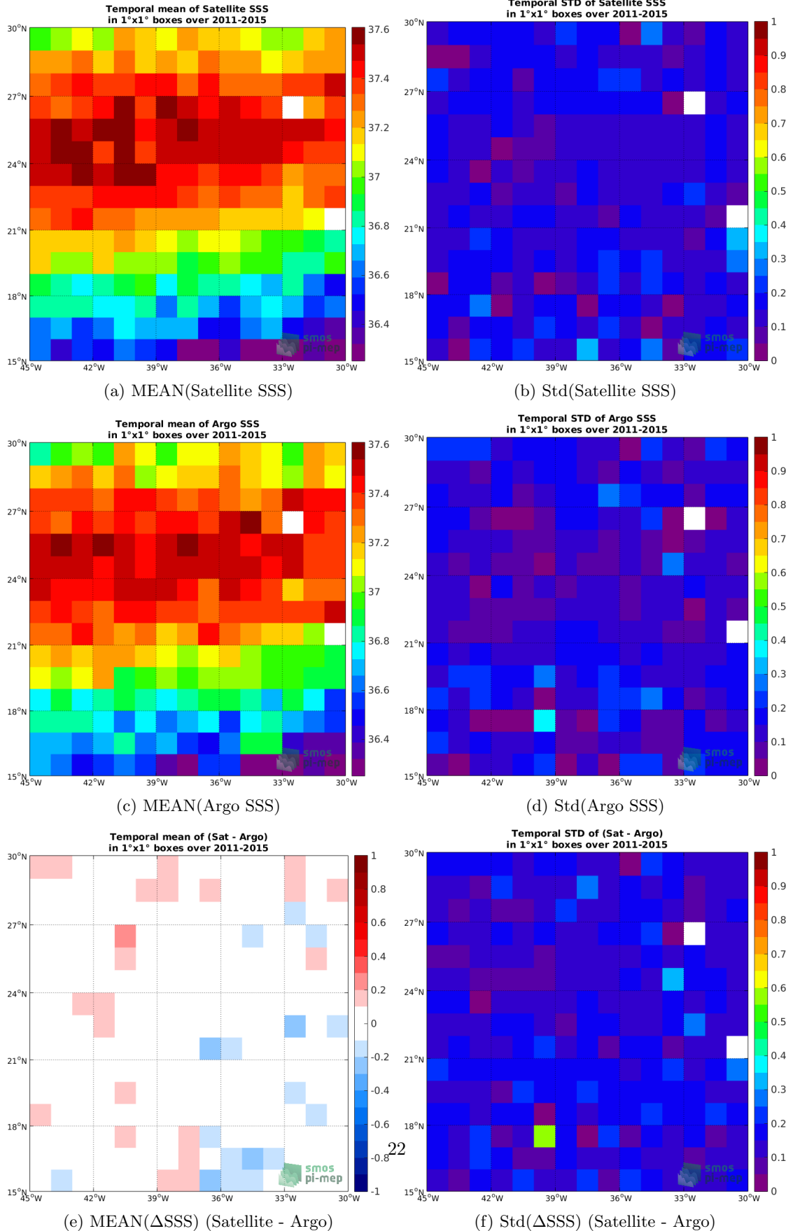
Figure 6: Temporal mean (left) and Std (right) of SSS from Aquarius-L3-JPL-V5-7DAY-RUNNING (top), Argo (middle), and of \Delta SSS (Satellite - Argo). Only match-up pairs are used to generate these maps.
