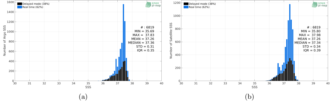
Figure 2: Histograms of SSS from Argo (a) and Aquarius-L3-JPL-V5-7DAY-RUNNING (b) considering all match-up pairs per bins of 0.1 over the SPURS 1 Pi-MEP region and for the full satellite product period.
