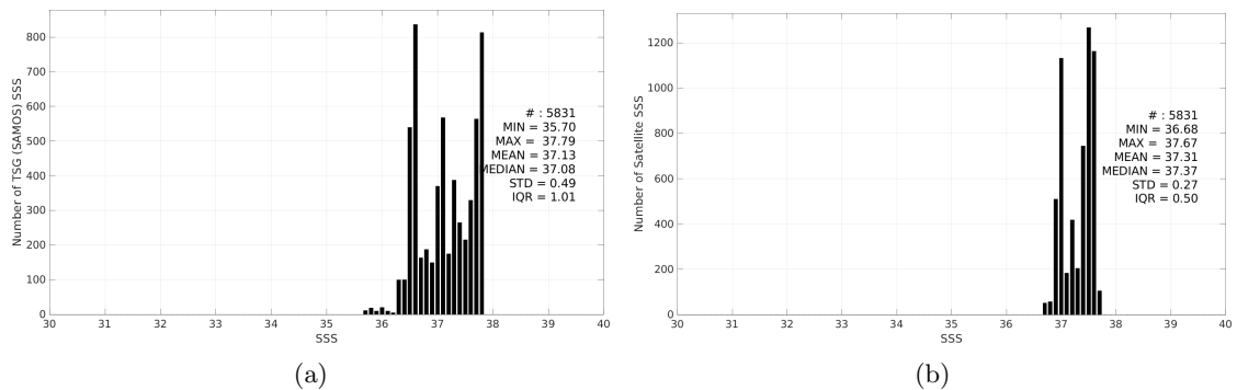
Figure 3: Histograms of SSS from TSG (SAMOS) (a) and Aquarius SSS L3 CAP v5 - Monthly (JPL) (b) considering all match-up pairs per bins of 0.1 over the SPURS 1 Pi-MEP region and for the full satellite product period.
