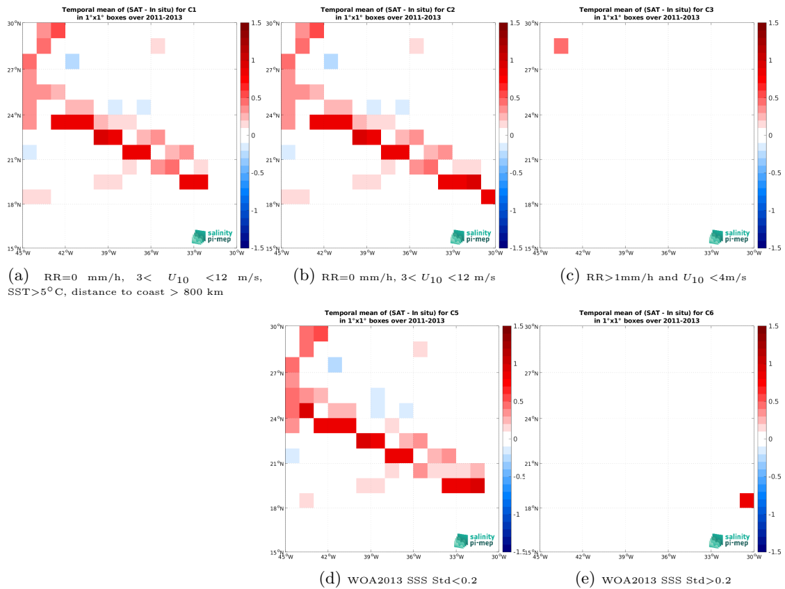
Figure 14: Temporal mean gridded over spatial boxes of size 1^\circ \times 1^\circ of \Delta SSS (Aquarius SSS L3 CAP v5 - Monthly (JPL) - TSG (SAMOS)) for 5 different subdatasets corresponding to:RR=0 mm/h, 3 < U_{10} < 12 m/s, SST>5°C, distance to coast > 800 km (a), RR=0 mm/h, 3 < U_{10} < 12 m/s (b), RR>1mm/h and U_{10} < 4 m/s (c), WOA2013 SSS Std<0.2 (d), WOA2013 SSS Std>0.2 (e).
