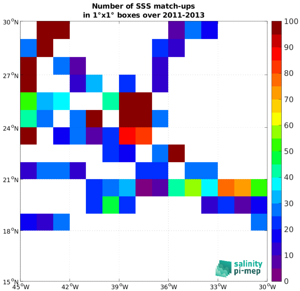
Figure 5: Number of SSS match-ups between TSG (SAMOS) SSS and the Aquarius SSS L3 CAP v5 - Monthly (JPL) SSS product for the SPURS 1 Pi-MEP region over 1^\circ \times 1^\circ boxes and for the full satellite product period.
