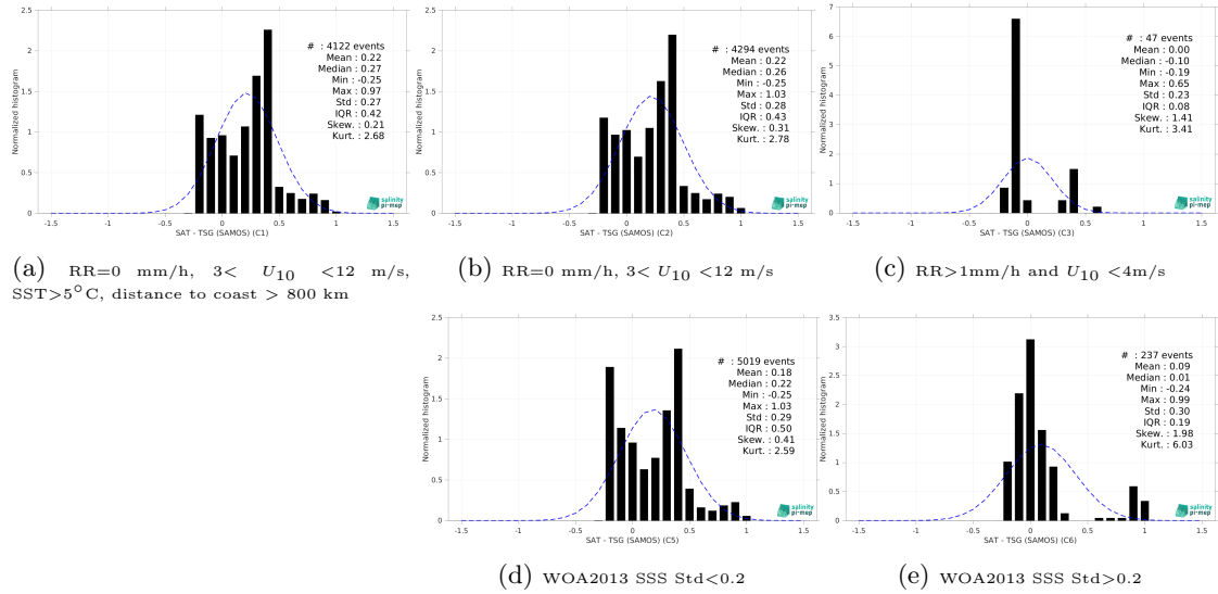
Figure 15: Normalized histogram of \Delta\text{SSS} (Aquarius SSS L3 CAP v5 - Monthly (JPL) - TSG (SAMOS)) for 5 different subdatasets corresponding to: RR=0 mm/h, 3 < U_{10} < 12 m/s, SST>5°C, distance to coast > 800 km (a), RR=0 mm/h, 3 < U_{10} < 12 m/s (b), RR>1mm/h and U_{10} < 4 m/s (c), WOA2013 SSS Std<0.2 (d), WOA2013 SSS Std>0.2 (e).
