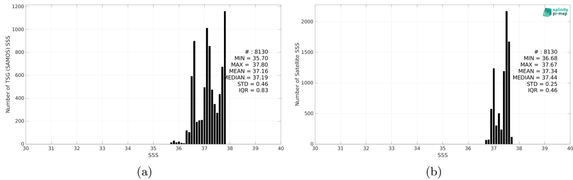
Figure 2: Histograms of SSS from TSG (SAMOS) (a) and Aquarius SSS L3 CAP v5 - Monthly (JPL) (b) considering all match-up pairs per bins of 0.1 over the SPURS 1 Pi-MEP region and for the full satellite product period.
