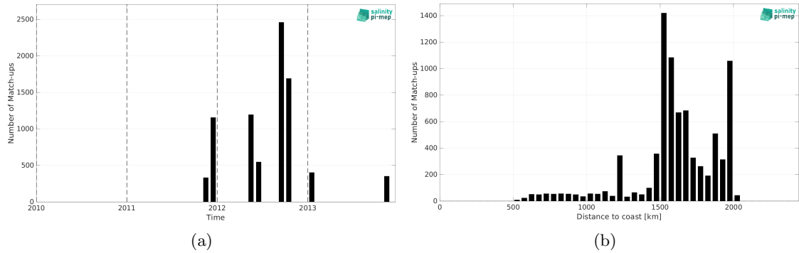
Figure 1: Number of match-ups between TSG (SAMOS) and Aquarius SSS L3 CAP v5 - Monthly (JPL) SSS as a function of time (a) and as function of the distance to coast (b) over the SPURS 1 Pi-MEP region and for the full satellite product period.
