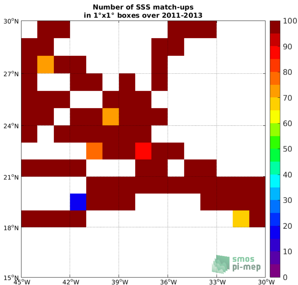
Figure 4: Number of SSS match-ups between TSG (SAMOS) SSS and the Aquarius SSS L3 CAP v5 - Monthly (JPL) SSS product for the SPURS 1 Pi-MEP region over 1°x1° boxes and for the full satellite product period.
