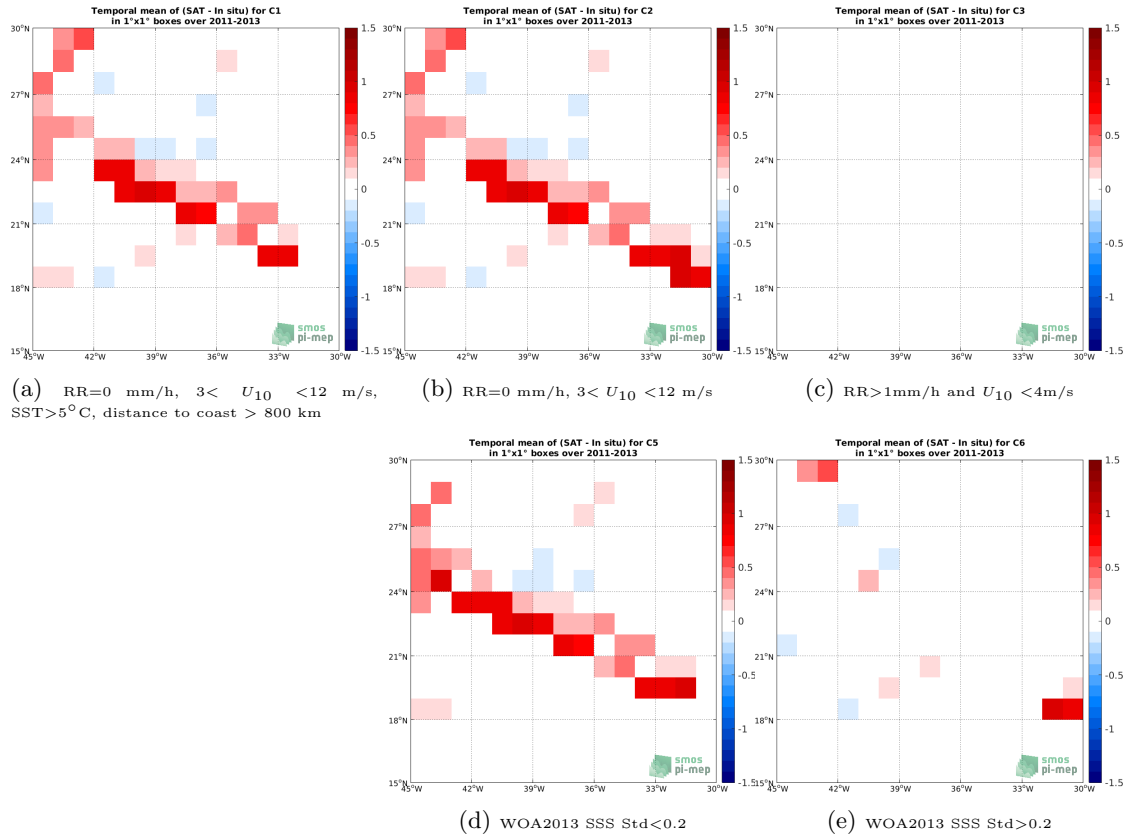
Figure 12: Temporal mean gridded over spatial boxes of size 1^\circ \times 1^\circ of \Delta SSS (Aquarius SSS L3 CAP v5 - Monthly (JPL) - TSG (SAMOS)) for 5 different subdatasets corresponding to: RR=0 mm/h, 3 < U_{10} < 12 m/s, SST > 5^\circ\text{C} , distance to coast > 800 km (a), RR=0 mm/h, 3 < U_{10} < 12 m/s (b), RR > 1 mm/h and U_{10} < 4 m/s (c), WOA2013 SSS Std < 0.2 (d), WOA2013 SSS Std > 0.2 (e).
