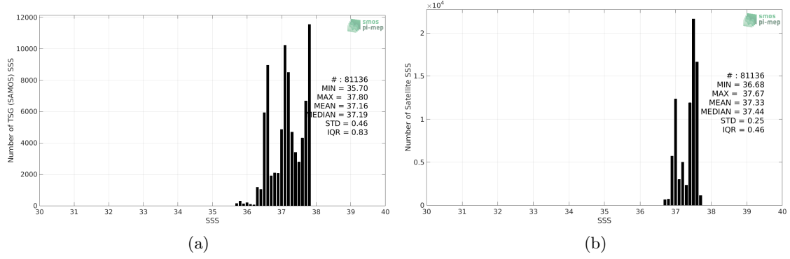
Figure 2: Histograms of SSS from TSG (SAMOS) (a) and Aquarius SSS L3 CAP v5 - Monthly (JPL) (b) considering all match-up pairs per bins of 0.1 over the SPURS 1 Pi-MEP region and for the full satellite product period.
