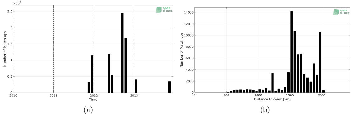
Figure 1: Number of match-ups between TSG (SAMOS) and Aquarius SSS L3 CAP v5 - Monthly (JPL) SSS as a function of time (a) and as function of the distance to coast (b) over the SPURS 1 Pi-MEP region and for the full satellite product period.
