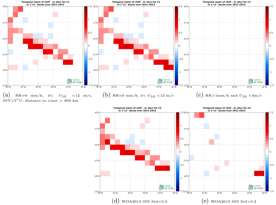
Figure 12: Temporal mean gridded over spatial boxes of size 1^\circ \times 1^\circ of \Delta SSS (Aquarius-L3-JPL-V5-MONTHLY - TSG-SAMOS) for 5 different subdatasets corresponding to: RR=0 mm/h, 3 < U_{10} < 12 m/s, SST >5^\circ C, distance to coast > 800 km (a), RR=0 mm/h, 3 < U_{10} < 12 m/s (b), RR >1 mm/h and U_{10} < 4 m/s (c), WOA2013 SSS Std <0.2 (d), WOA2013 SSS Std >0.2 (e).
