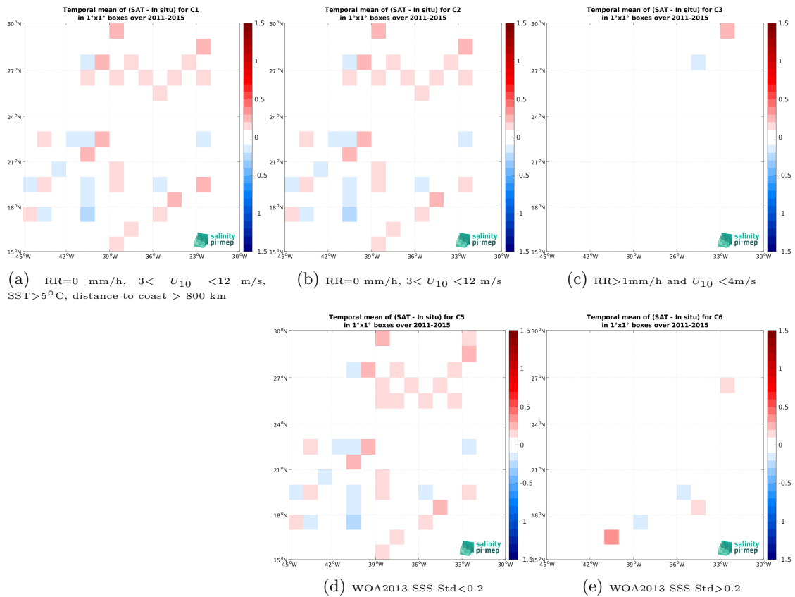
Figure 14: Temporal mean gridded over spatial boxes of size 1^\circ \times 1^\circ of \Delta SSS (Aquarius SSS L3 CAP v5 - Monthly (JPL) - TSG (LEGOS-DM)) for 5 different subdatasets corresponding to:RR=0 mm/h, 3 < U_{10} < 12 m/s, SST>5°C, distance to coast > 800 km (a), RR=0 mm/h, 3 < U_{10} < 12 m/s (b), RR>1mm/h and U_{10} < 4 m/s (c), WOA2013 SSS Std<0.2 (d), WOA2013 SSS Std>0.2 (e).
