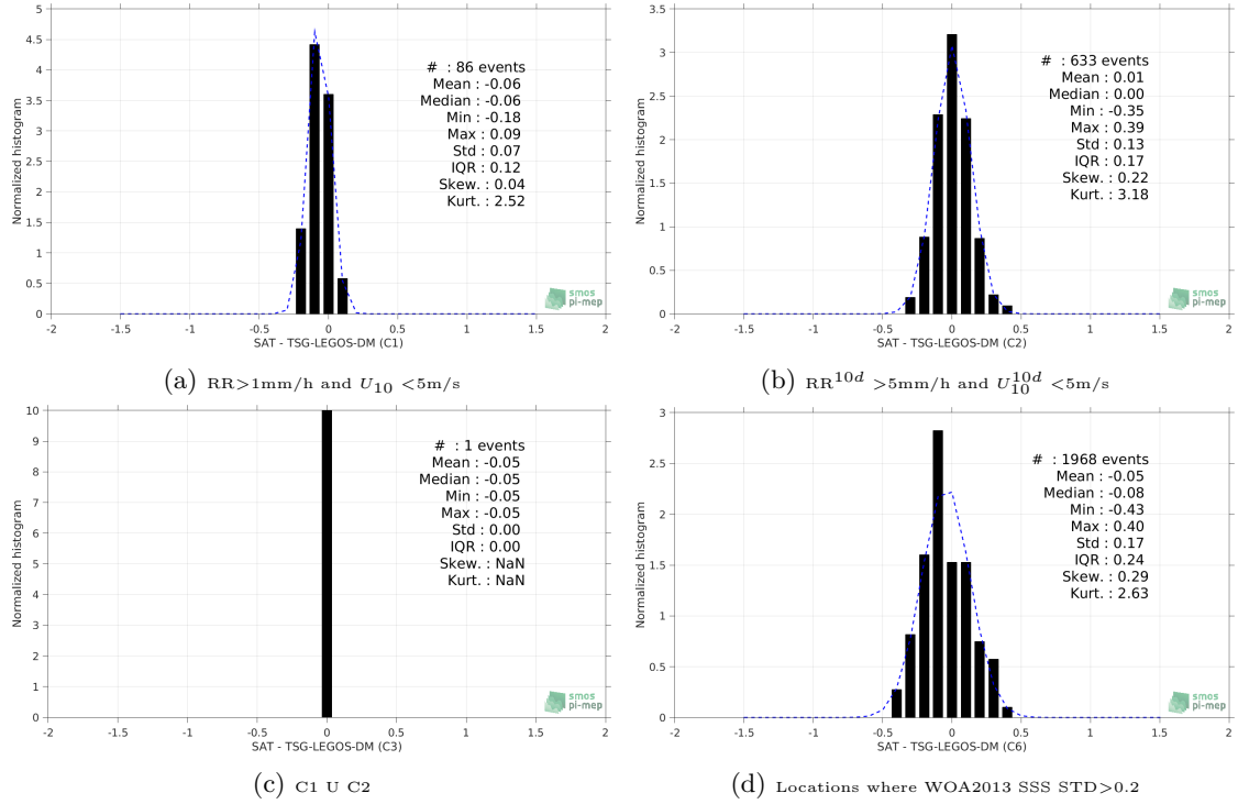
Figure 13: Normalized histogram of \Delta\text{SSS} (Aquarius-L3-JPL-V5-MONTHLY - TSG-LEGOS-DM) for 6 different subdatasets corresponding to: RR > 1mm/h and U_{10} < 5\text{m/s} (a), \text{RR}^{10d} > 5\text{mm/h} and U_{10}^{10d} < 5\text{m/s} (b), C1 U C2 (c), Locations where WOA2013 SSS STD > 0.2 (d).
