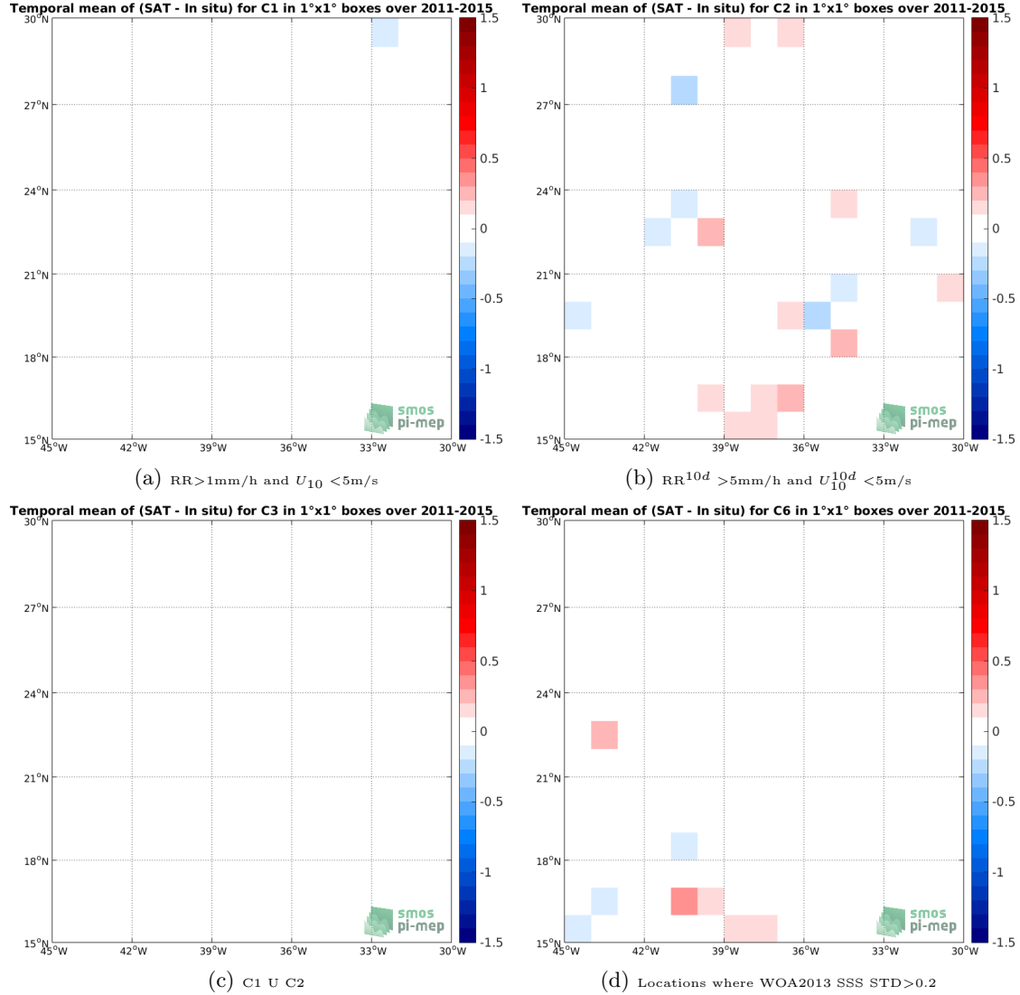
Figure 12: Temporal mean gridded over spatial boxes of size 1^\circ \times 1^\circ of \Delta SSS (Aquarius-L3-JPL-V5-MONTHLY - TSG-LEGOS-DM) for 4 different subdatasets corresponding to: RR > 1\text{mm/h} and U_{10} < 5\text{m/s} (a), RR^{10d} > 5\text{mm/h} and U_{10}^{10d} < 5\text{m/s} (b), C1 U C2 (c), Locations where WOA2013 SSS STD > 0.2 (d).
