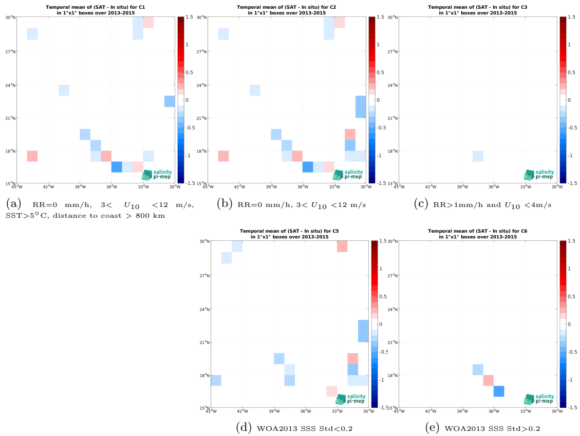
Figure 14: Temporal mean gridded over spatial boxes of size 1^\circ \times 1^\circ of \Delta\text{SSS} (Aquarius SSS L3 CAP v5 - Monthly (JPL) - TSG (GOSUD-Sailing-ship)) for 5 different subdatasets corresponding to:RR=0 mm/h, 3 < U_{10} < 12 m/s, SST>5°C, distance to coast > 800 km (a), RR=0 mm/h, 3 < U_{10} < 12 m/s (b), RR>1mm/h and U_{10} < 4 m/s (c), WOA2013 SSS Std<0.2 (d), WOA2013 SSS Std>0.2 (e).
