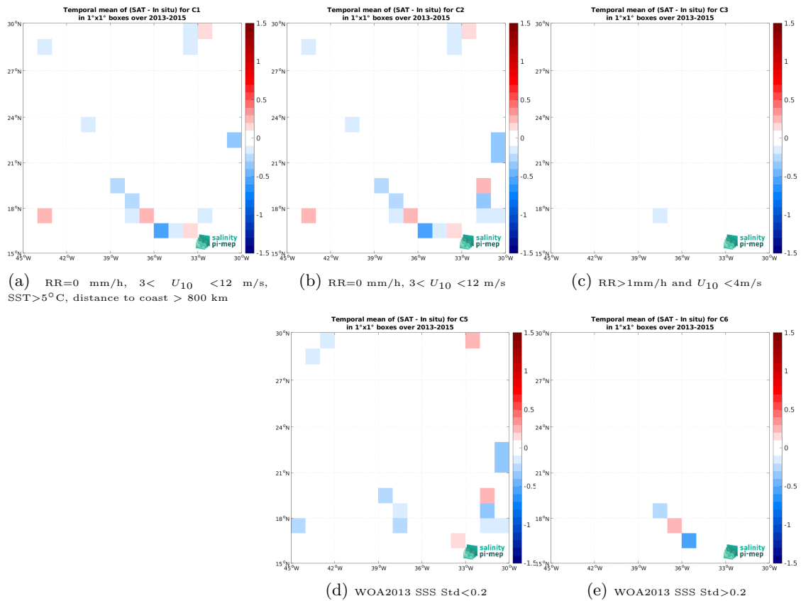
Figure 14: Temporal mean gridded over spatial boxes of size 1^\circ \times 1^\circ of \Delta SSS (Aquarius SSS L3 CAP v5 - Monthly (JPL) - TSG (GOSUD-Sailing-ship)) for 5 different subdatasets corresponding to: RR=0 mm/h, 3 < U_{10} < 12 m/s, SST > 5^\circ C , distance to coast > 800 km (a), RR=0 mm/h, 3 < U_{10} < 12 m/s (b), RR > 1 mm/h and U_{10} < 4 m/s (c), WOA2013 SSS Std < 0.2 (d), WOA2013 SSS Std > 0.2 (e).
