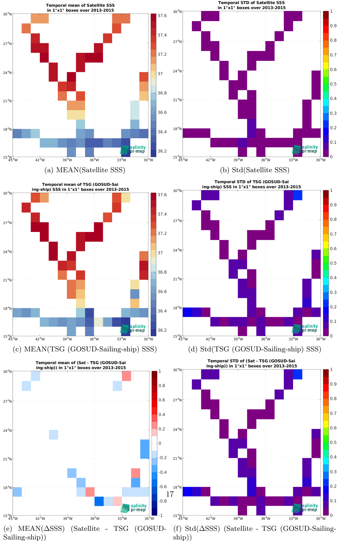
Figure 7: Temporal mean (left) and Std (right) of SSS from Aquarius SSS L3 CAP v5 - Monthly (JPL) (top), TSG (GOSUD-Sailing-ship) (middle), and of \Delta SSS (Satellite - TSG (GOSUD-Sailing-ship)). Only match-up pairs are used to generate these maps.
