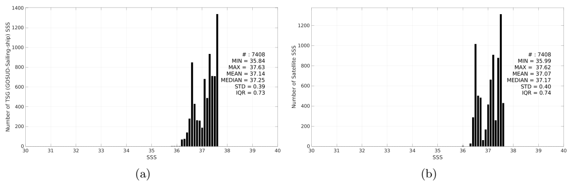
Figure 3: Histograms of SSS from TSG (GOSUD-Sailing-ship) (a) and Aquarius SSS L3 CAP v5 - Monthly (JPL) (b) considering all match-up pairs per bins of 0.1 over the SPURS 1 Pi-MEP region and for the full satellite product period.
