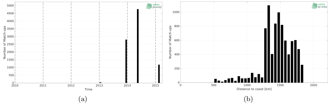
Figure 1: Number of match-ups between TSG (GOSUD-Sailing-ship) and Aquarius SSS L3 CAP v5 - Monthly (JPL) SSS as a function of time (a) and as function of the distance to coast (b) over the SPURS 1 Pi-MEP region and for the full satellite product period.
