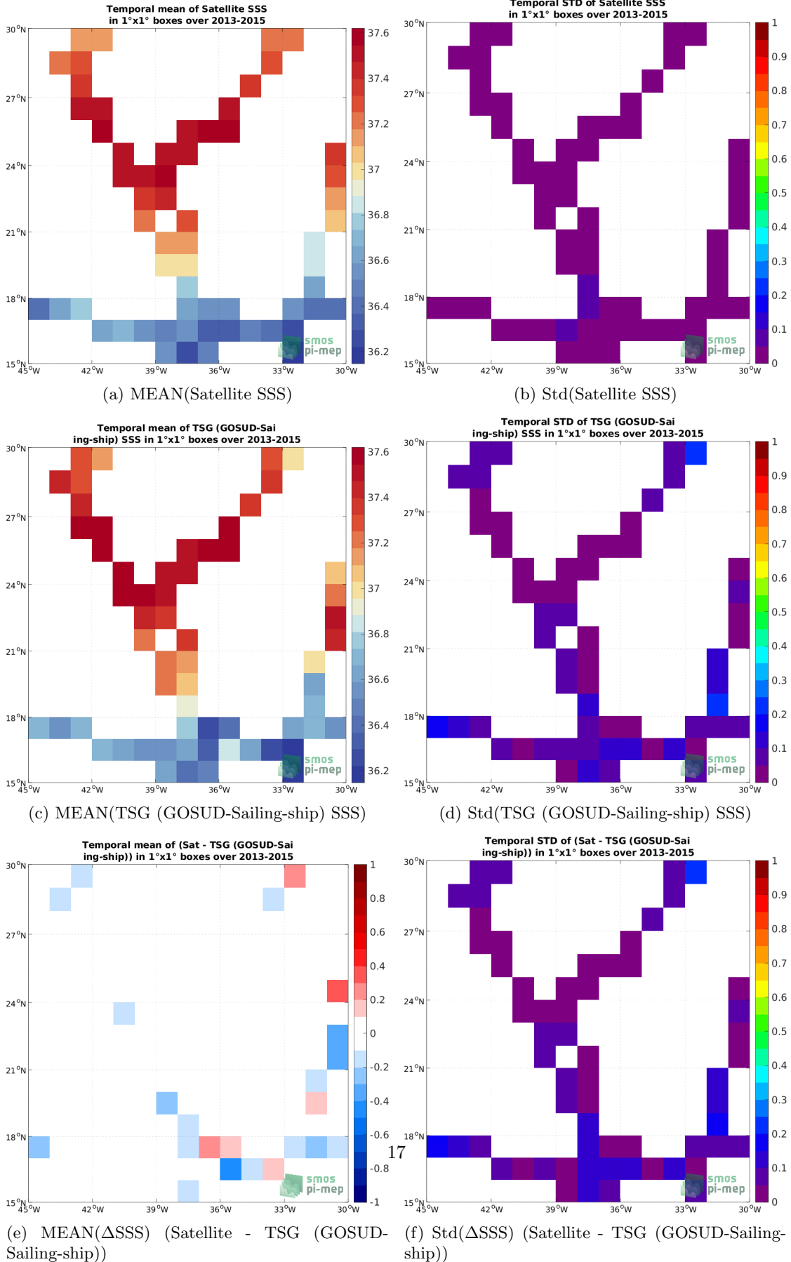
Figure 6: Temporal mean (left) and Std (right) of SSS from Aquarius SSS L3 CAP v5 - Monthly (JPL) (top), TSG (GOSUD-Sailing-ship) (middle), and of \Delta SSS (Satellite - TSG (GOSUD-Sailing-ship)). Only match-up pairs are used to generate these maps.
