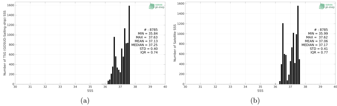
Figure 2: Histograms of SSS from TSG (GOSUD-Sailing-ship) (a) and Aquarius SSS L3 CAP v5 - Monthly (JPL) (b) considering all match-up pairs per bins of 0.1 over the SPURS 1 Pi-MEP region and for the full satellite product period.
