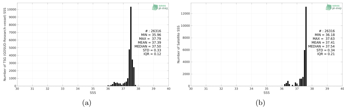
Figure 2: Histograms of SSS from TSG (GOSUD-Research-vessel) (a) and Aquarius SSS L3 CAP v5 - Monthly (JPL) (b) considering all match-up pairs per bins of 0.1 over the SPURS 1 Pi-MEP region and for the full satellite product period.
