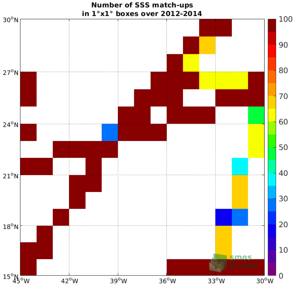
Figure 4: Number of SSS match-ups between TSG (GOSUD-Research-vessel) SSS and the Aquarius SSS L3 CAP v5 - Monthly (JPL) SSS product for the SPURS 1 Pi-MEP region over 1^\circ \times 1^\circ boxes and for the full satellite product period.
