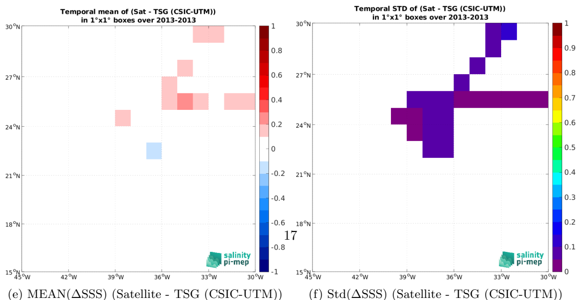
Figure 7: Temporal mean (left) and Std (right) of SSS from Aquarius SSS L3 CAP v5 - Monthly (JPL) (top), TSG (CSIC-UTM) (middle), and of \Delta SSS (Satellite - TSG (CSIC-UTM)). Only match-up pairs are used to generate these maps.
