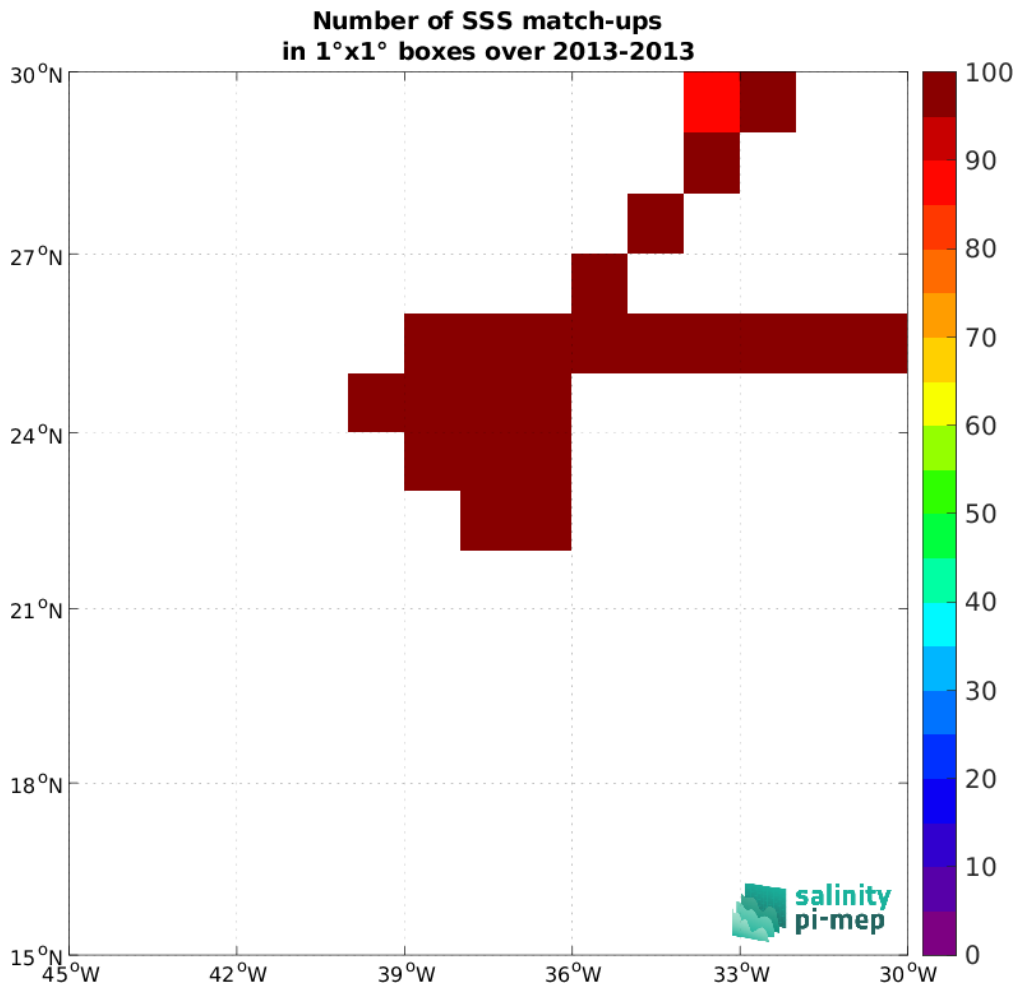
Figure 5: Number of SSS match-ups between TSG (CSIC-UTM) SSS and the Aquarius SSS L3 CAP v5 - Monthly (JPL) SSS product for the SPURS 1 Pi-MEP region over 1°×1° boxes and for the full satellite product period.
