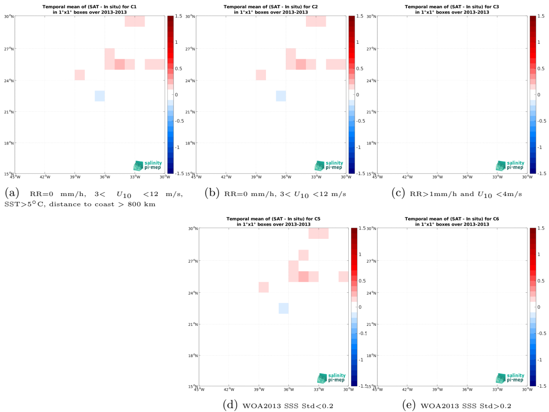
Figure 14: Temporal mean gridded over spatial boxes of size 1^\circ \times 1^\circ of \Delta SSS (Aquarius SSS L3 CAP v5 - Monthly (JPL) - TSG (CSIC-UTM)) for 5 different subdatasets corresponding to:RR=0 mm/h, 3 < U_{10} < 12 m/s, SST >5^\circ C, distance to coast > 800 km (a), RR=0 mm/h, 3 < U_{10} < 12 m/s (b), RR >1 mm/h and U_{10} < 4 m/s (c), WOA2013 SSS Std <0.2 (d), WOA2013 SSS Std >0.2 (e).
