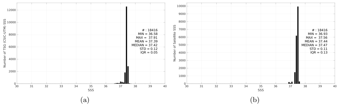
Figure 3: Histograms of SSS from TSG (CSIC-UTM) (a) and Aquarius SSS L3 CAP v5 - Monthly (JPL) (b) considering all match-up pairs per bins of 0.1 over the SPURS 1 Pi-MEP region and for the full satellite product period.
