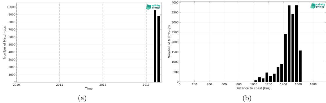
Figure 2: Number of match-ups between TSG (CSIC-UTM) and Aquarius SSS L3 CAP v5 - Monthly (JPL) SSS as a function of time (a) and as function of the distance to coast (b) over the SPURS 1 Pi-MEP region and for the full satellite product period.
