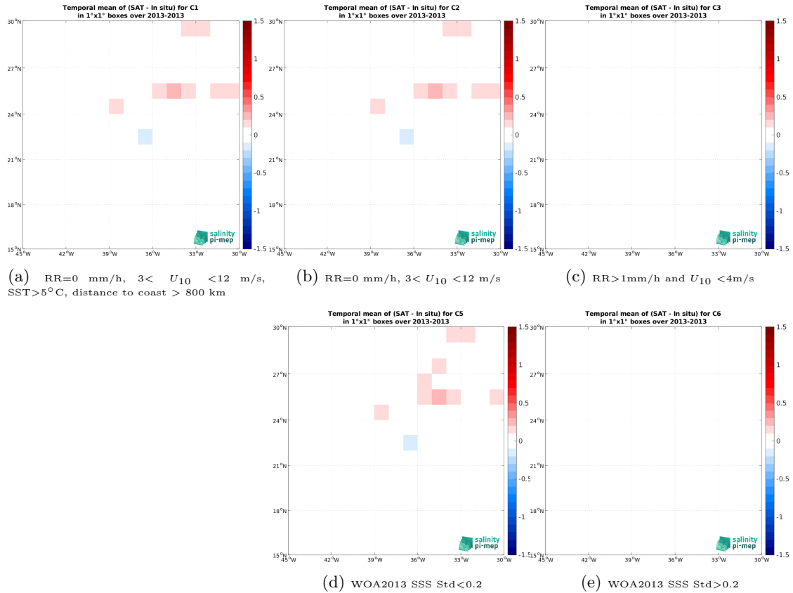
Figure 12: Temporal mean gridded over spatial boxes of size 1^{\circ}\times 1^{\circ} of \Delta\text{SSS} (Aquarius SSS L3 CAP v5 - Monthly (JPL) - TSG (CSIC-UTM)) for 5 different subdatasets corresponding to:RR=0 mm/h, 3 < U_{10} < 12 m/s, SST >5^{\circ}\text{C} , distance to coast > 800 km (a), RR=0 mm/h, 3 < U_{10} < 12 m/s (b), RR >1 mm/h and U_{10} < 4 m/s (c), WOA2013 SSS Std <0.2 (d), WOA2013 SSS Std >0.2 (e).
