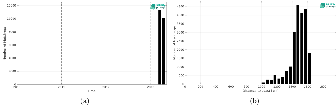
Figure 1: Number of match-ups between TSG (CSIC-UTM) and Aquarius SSS L3 CAP v5 - Monthly (JPL) SSS as a function of time (a) and as function of the distance to coast (b) over the SPURS 1 Pi-MEP region and for the full satellite product period.
