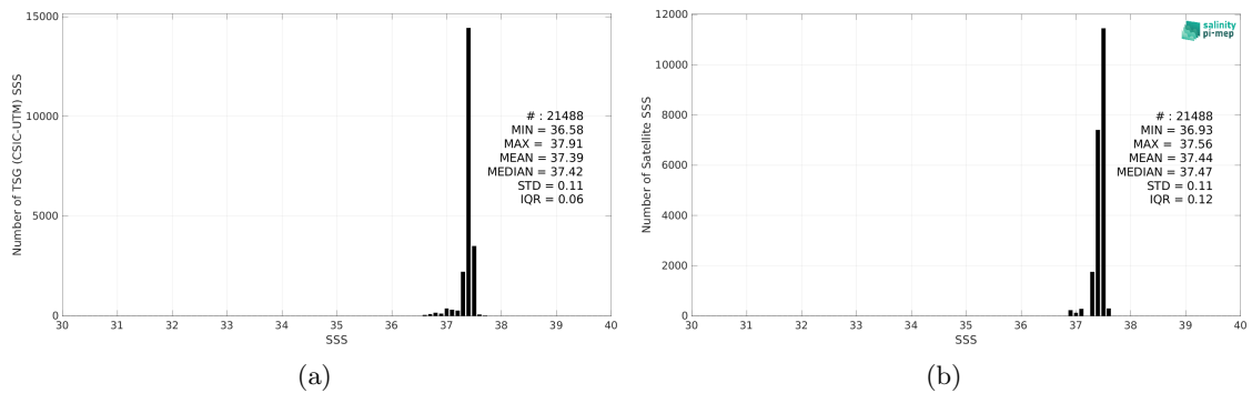
Figure 2: Histograms of SSS from TSG (CSIC-UTM) (a) and Aquarius SSS L3 CAP v5 - Monthly (JPL) (b) considering all match-up pairs per bins of 0.1 over the SPURS 1 Pi-MEP region and for the full satellite product period.
