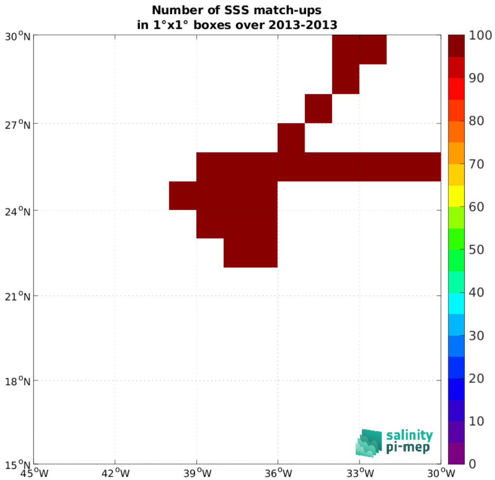
Figure 4: Number of SSS match-ups between TSG (CSIC-UTM) SSS and the Aquarius SSS L3 CAP v5 - Monthly (JPL) SSS product for the SPURS 1 Pi-MEP region over 1°x1° boxes and for the full satellite product period.
