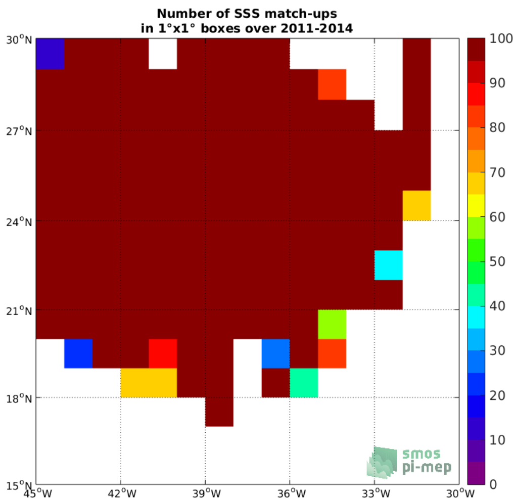
Figure 3: Number of SSS match-ups between Surface drifters SSS and the Aquarius-L3-JPL-V5-MONTHLY SSS product for the SPURS 1 Pi-MEP region over 1°x1° boxes and for the full satellite product period.
