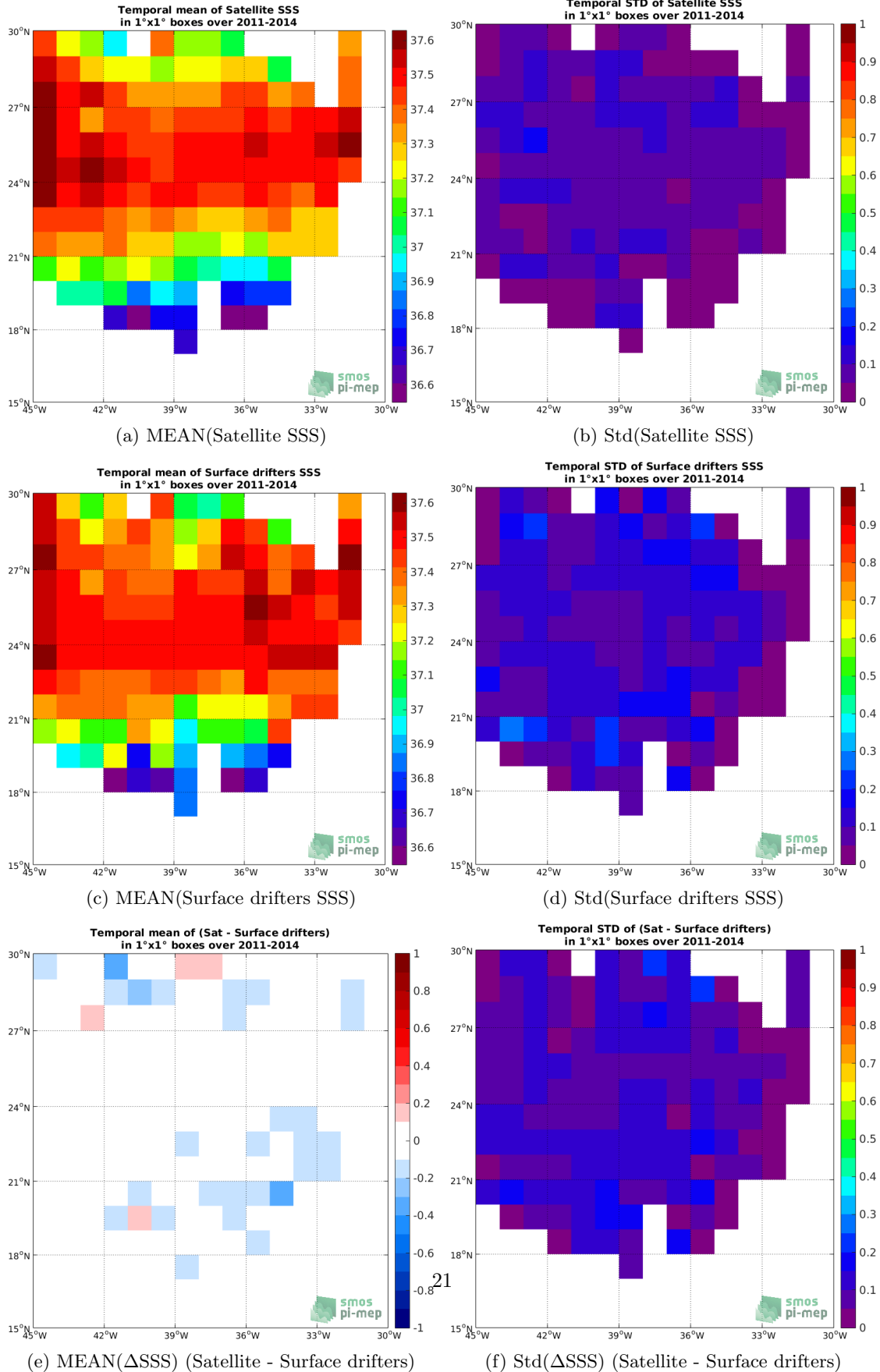
Figure 5: Temporal mean (left) and Std (right) of SSS from Aquarius-L3-JPL-V5-MONTHLY (top), Surface drifters (middle), and of \Delta SSS (Satellite - Surface drifters). Only match-up pairs are used to generate these maps.
