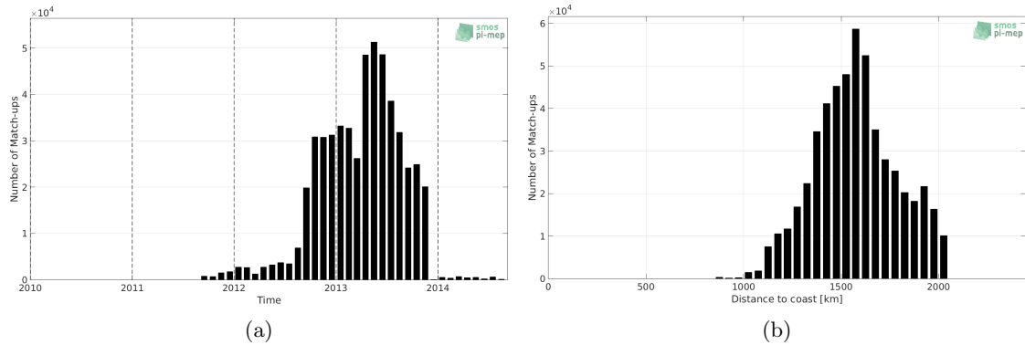
Figure 1: Number of match-ups between Surface drifters and Aquarius-L3-JPL-V5-MONTHLY SSS as a function of time (a) and as function of the distance to coast (b) over the SPURS 1 Pi-MEP region and for the full satellite product period.
