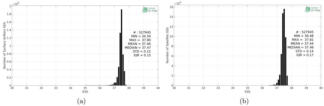
Figure 2: Histograms of SSS from Surface drifters (a) and Aquarius-L3-JPL-V5-MONTHLY (b) considering all match-up pairs per bins of 0.1 over the SPURS 1 Pi-MEP region and for the full satellite product period.
