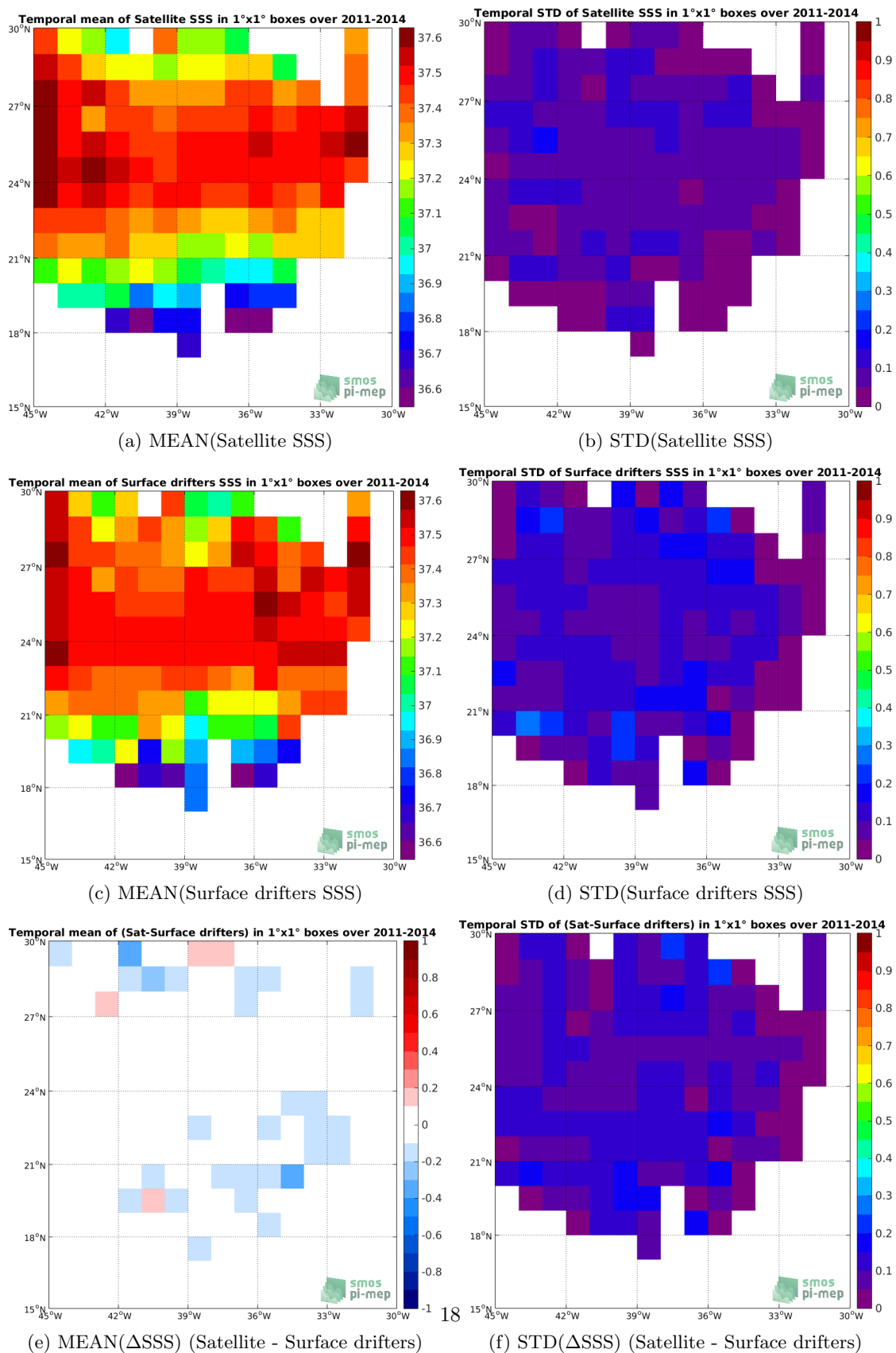
Figure 5: Temporal mean (left) and STD (right) of SSS from Aquarius-L3-JPL-V5-MONTHLY (top), Surface drifters (middle), and of \Delta SSS (Satellite - Surface drifters). Only match-up pairs are used to generate these maps.
