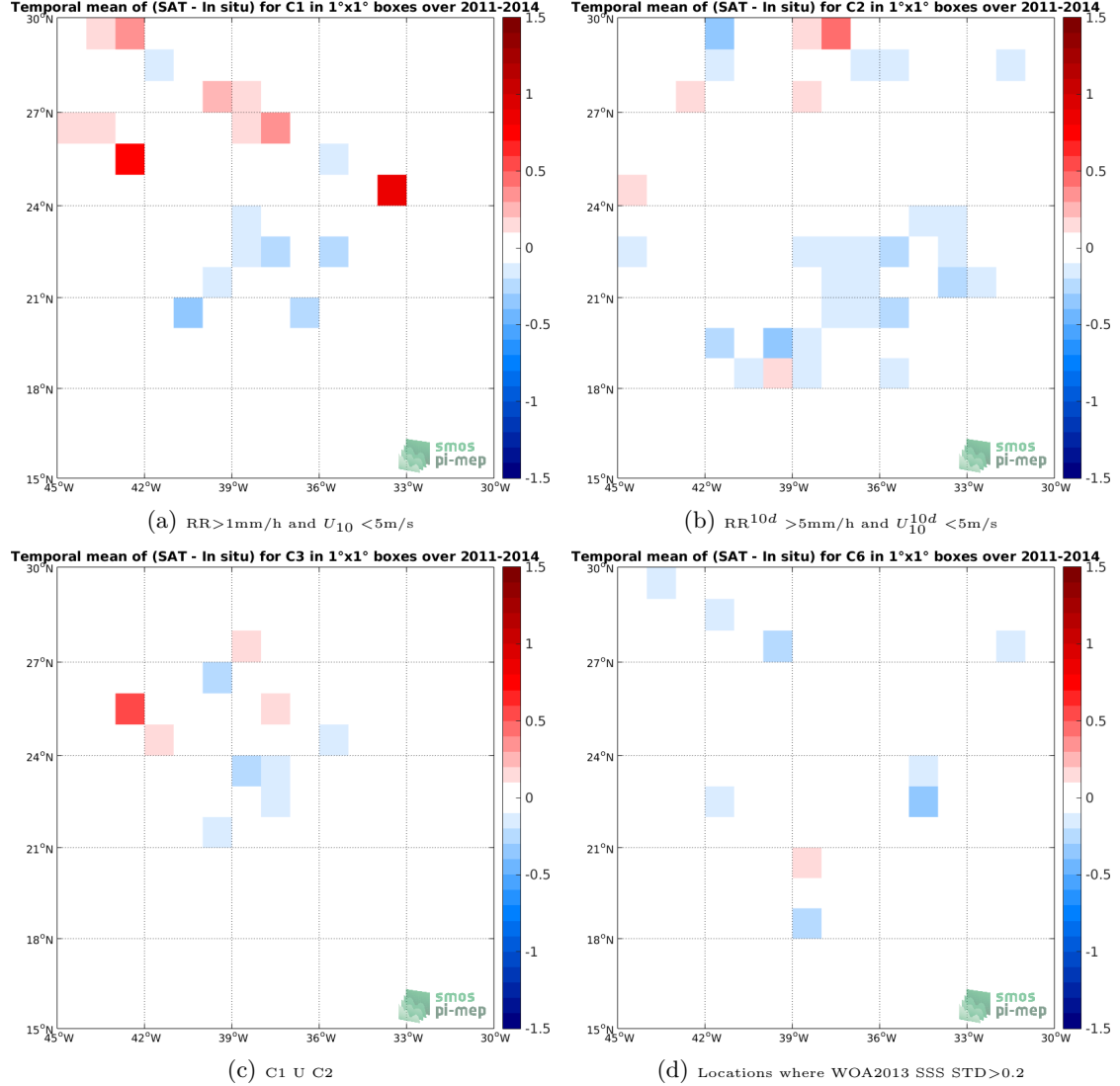
Figure 11: Temporal mean gridded over spatial boxes of size 1^\circ \times 1^\circ of \Delta SSS (Aquarius-L3-JPL-V5-MONTHLY - Surface drifters) for 4 different subdatasets corresponding to: RR > 1 \text{ mm/h} and U_{10} < 5 \text{ m/s} (a), RR^{10d} > 5 \text{ mm/h} and U_{10}^{10d} < 5 \text{ m/s} (b), C1 U C2 (c), Locations where WOA2013 SSS STD > 0.2 (d).
