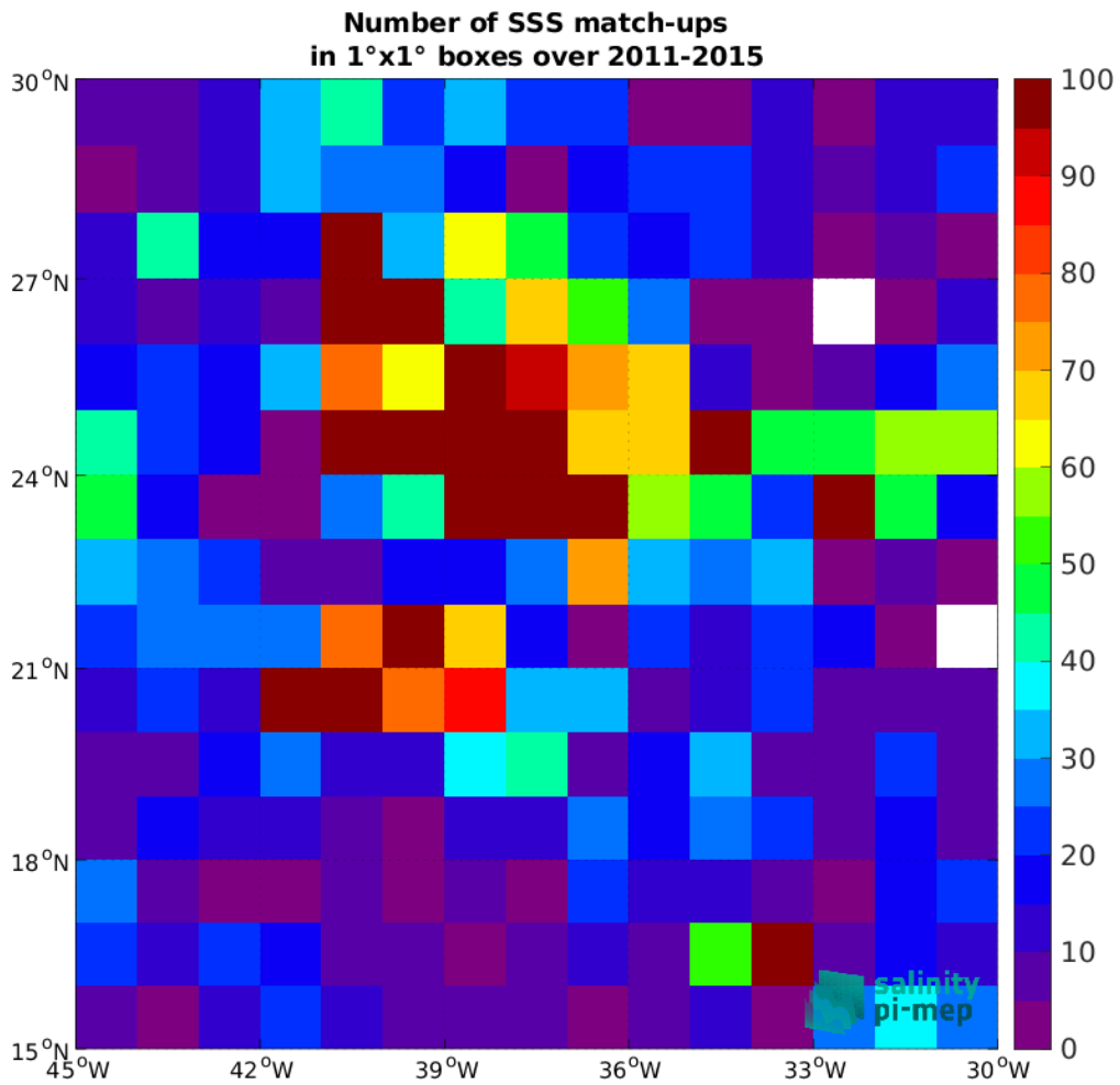
Figure 4: Number of SSS match-ups between Argo SSS and the Aquarius SSS L3 CAP v5 - Monthly (JPL) SSS product for the SPURS 1 Pi-MEP region over 1°×1° boxes and for the full satellite product period.
