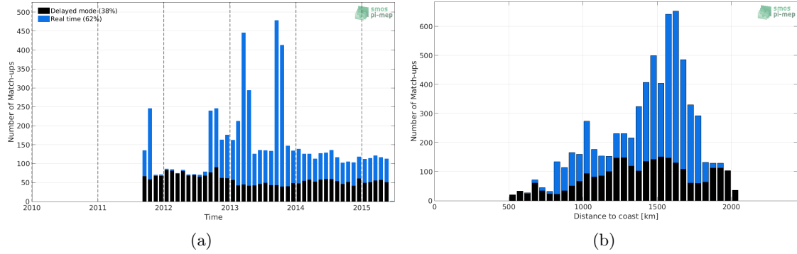
Figure 1: Number of match-ups between Argo and Aquarius-L3-JPL-V5-MONTHLY SSS as a function of time (a) and as function of the distance to coast (b) over the SPURS 1 Pi-MEP region and for the full satellite product period.
