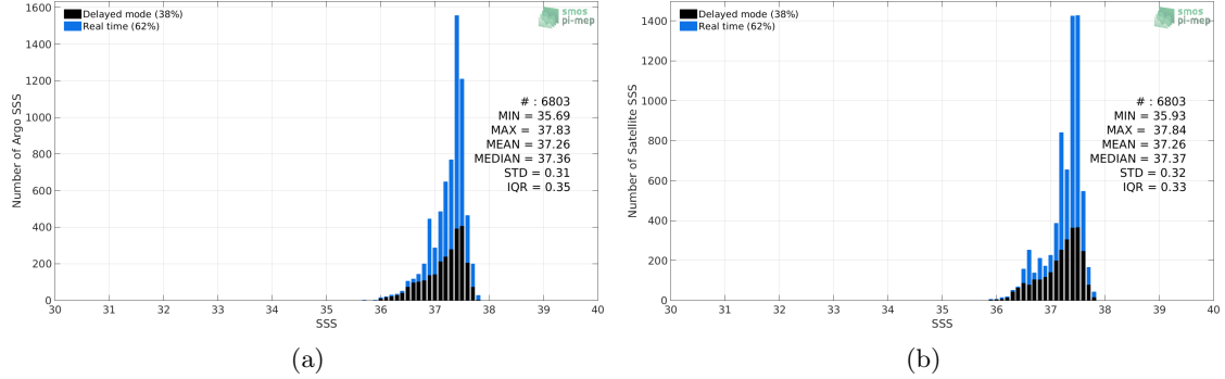
Figure 2: Histograms of SSS from Argo (a) and Aquarius-L3-JPL-V5-MONTHLY (b) considering all match-up pairs per bins of 0.1 over the SPURS 1 Pi-MEP region and for the full satellite product period.
