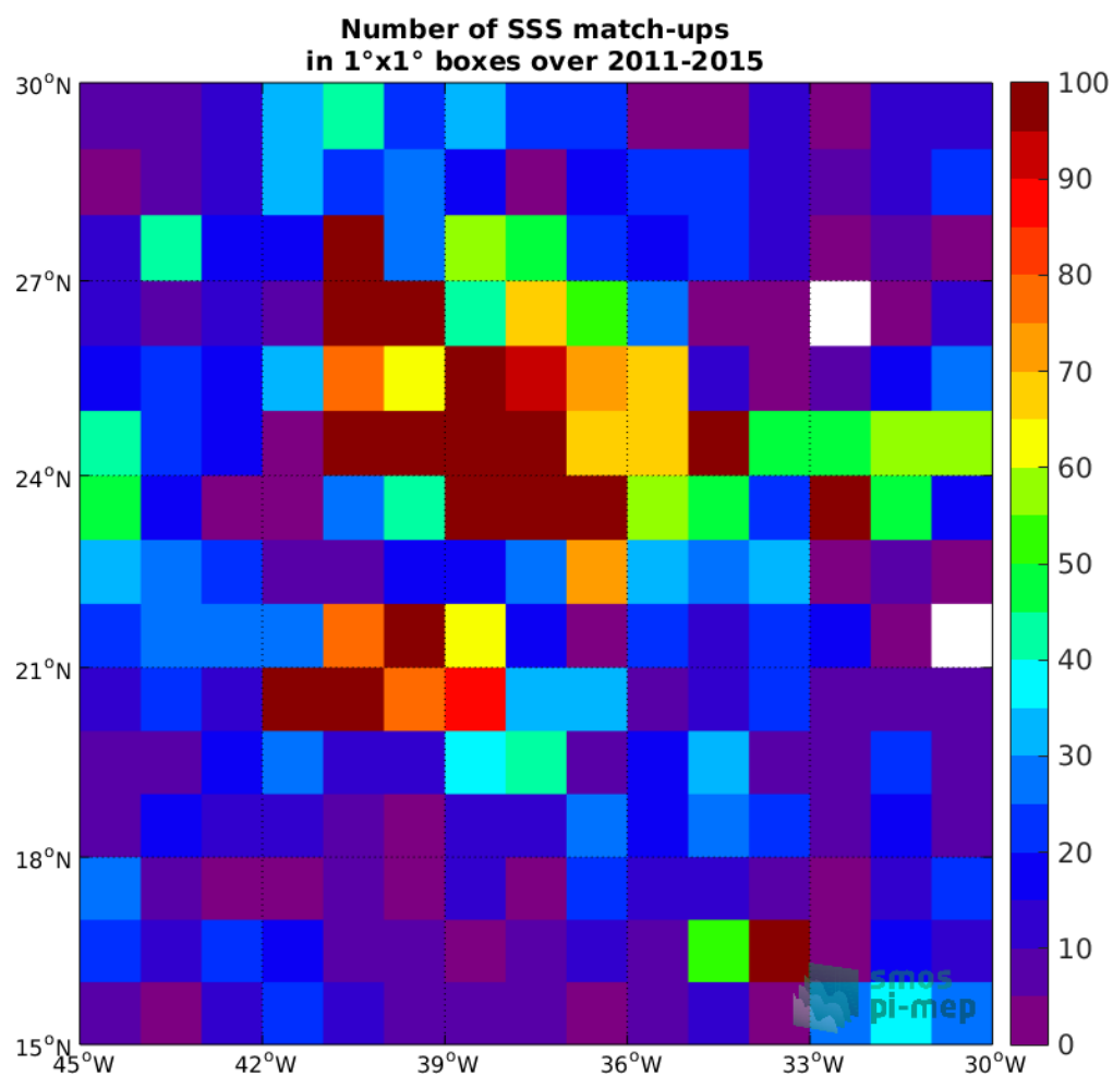
Figure 4: Number of SSS match-ups between Argo SSS and the Aquarius-L3-JPL-V5-MONTHLY SSS product for the SPURS 1 Pi-MEP region over 1°x1° boxes and for the full satellite product period.
