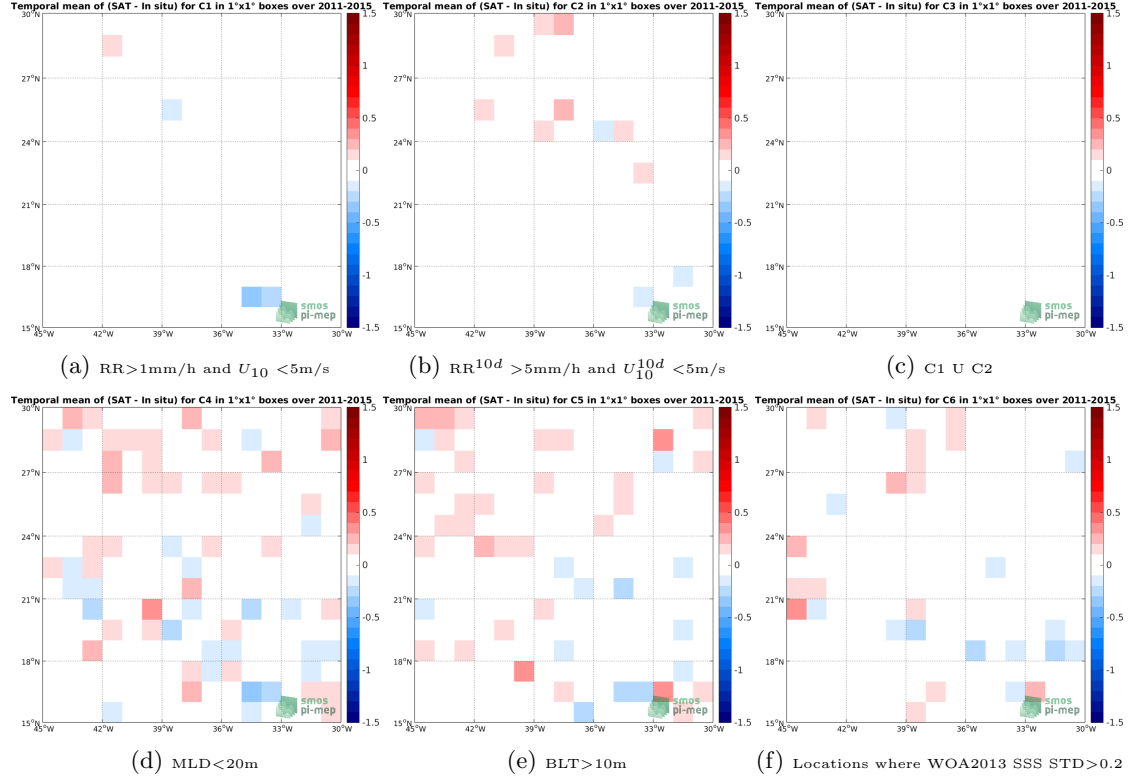
Figure 12: Temporal mean gridded over spatial boxes of size 1^\circ \times 1^\circ of \Delta\text{SSS} (Aquarius-L3-JPL-V5-MONTHLY - Argo) for 6 different subdatasets corresponding to: \text{RR} > 1\text{mm/h} and U_{10} < 5\text{m/s} (a), \text{RR}^{10d} > 5\text{mm/h} and U_{10}^{10d} < 5\text{m/s} (b), C1 U C2 (c), \text{MLD} < 20\text{m} (d), \text{BLT} > 10\text{m} (e), Locations where WOA2013 SSS STD > 0.2 (f).
