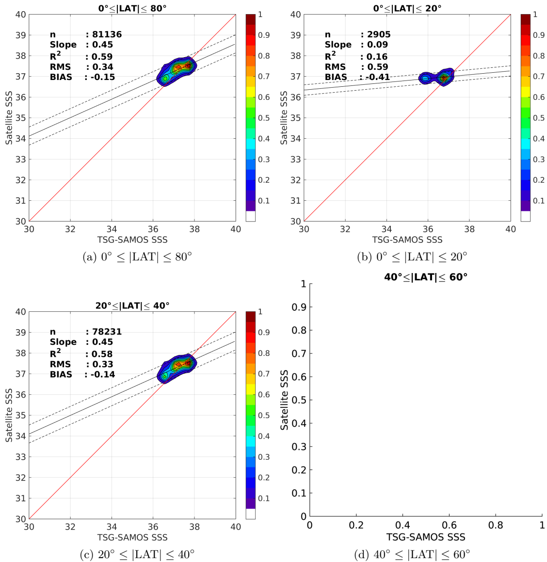
Figure 9: Contour maps of the concentration of Aquarius-L3-JPL-V4-7DAY-RUNNING SSS (y-axis) versus TSG-SAMOS SSS (x-axis) at match-up pairs for different latitude bands. For each plot, the red line shows x=y . The black thin and dashed lines indicate a linear fit through the data cloud and the \pm 95\% confidence levels, respectively. The number match-up pairs n , the slope and R^2 coefficient of the linear fit, the root mean square (RMS) and the mean bias between satellite and in situ data are indicated for each latitude band in each plots.
