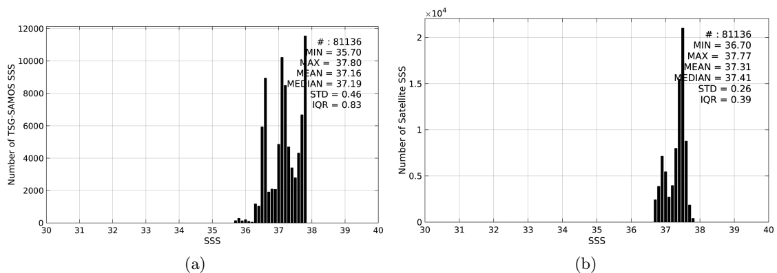
Figure 2: Histograms of SSS from TSG-SAMOS (a) and Aquarius-L3-JPL-V4-7DAY-RUNNING (b) considering all match-up pairs per bins of 0.1 over the SPURS 1 Pi-MEP region and for the full satellite product period.
