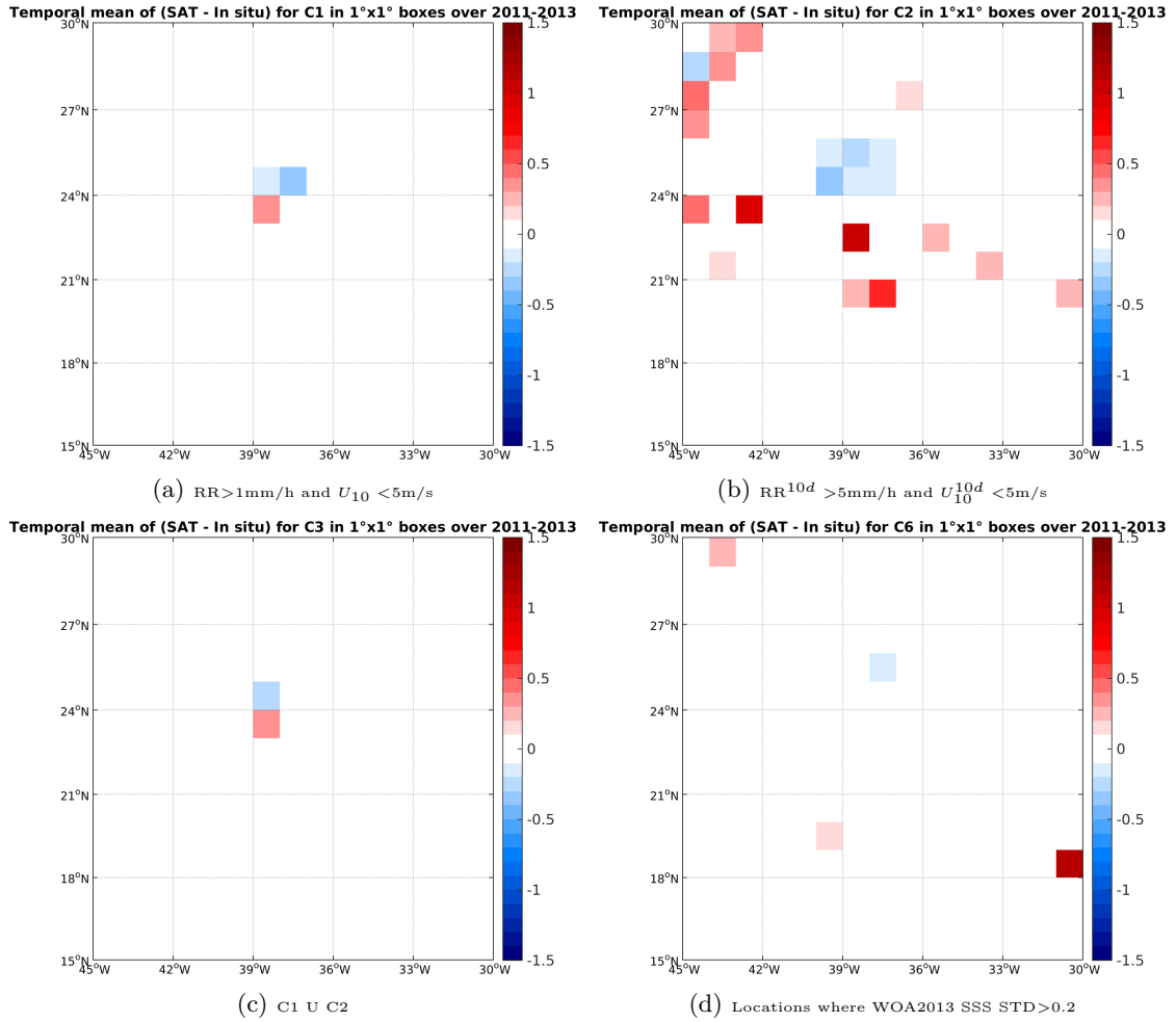
Figure 12: Temporal mean gridded over spatial boxes of size 1°x1° of \Delta SSS (Aquarius-L3-JPL-V4-7DAY-RUNNING - TSG-SAMOS) for 4 different subdatasets corresponding to:RR>1mm/h and U_{10} < 5m/s (a), RR^{10d} > 5mm/h and U_{10}^{10d} < 5m/s (b), C1 U C2 (c),Locations where WOA2013 SSS STD>0.2 (d).
