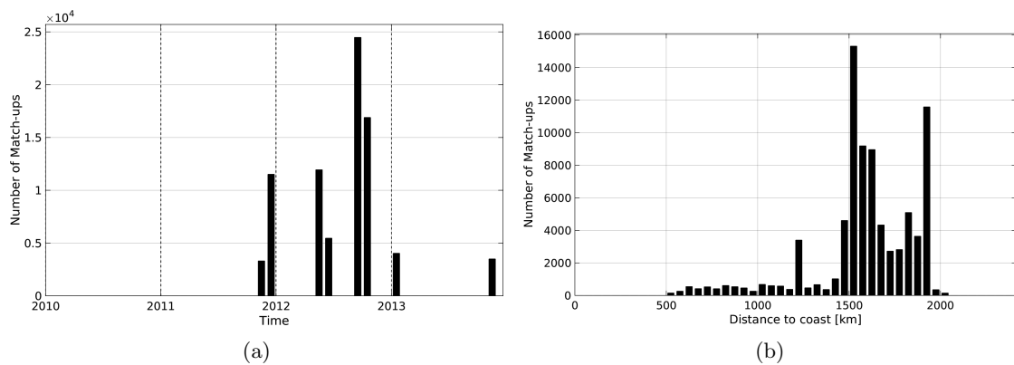
Figure 1: Number of match-ups between TSG-SAMOS and Aquarius-L3-JPL-V4-7DAY-RUNNING SSS as a function of time (a) and as function of the distance to coast (b) over the SPURS 1 Pi-MEP region and for the full satellite product period.
