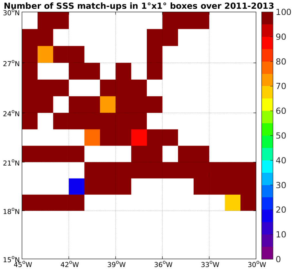
Figure 4: Number of SSS match-ups between TSG-SAMOS SSS and the Aquarius-L3-JPL-V4-7DAY-RUNNING SSS product for the SPURS 1 Pi-MEP region over 1°x1° boxes and for the full satellite product period.
