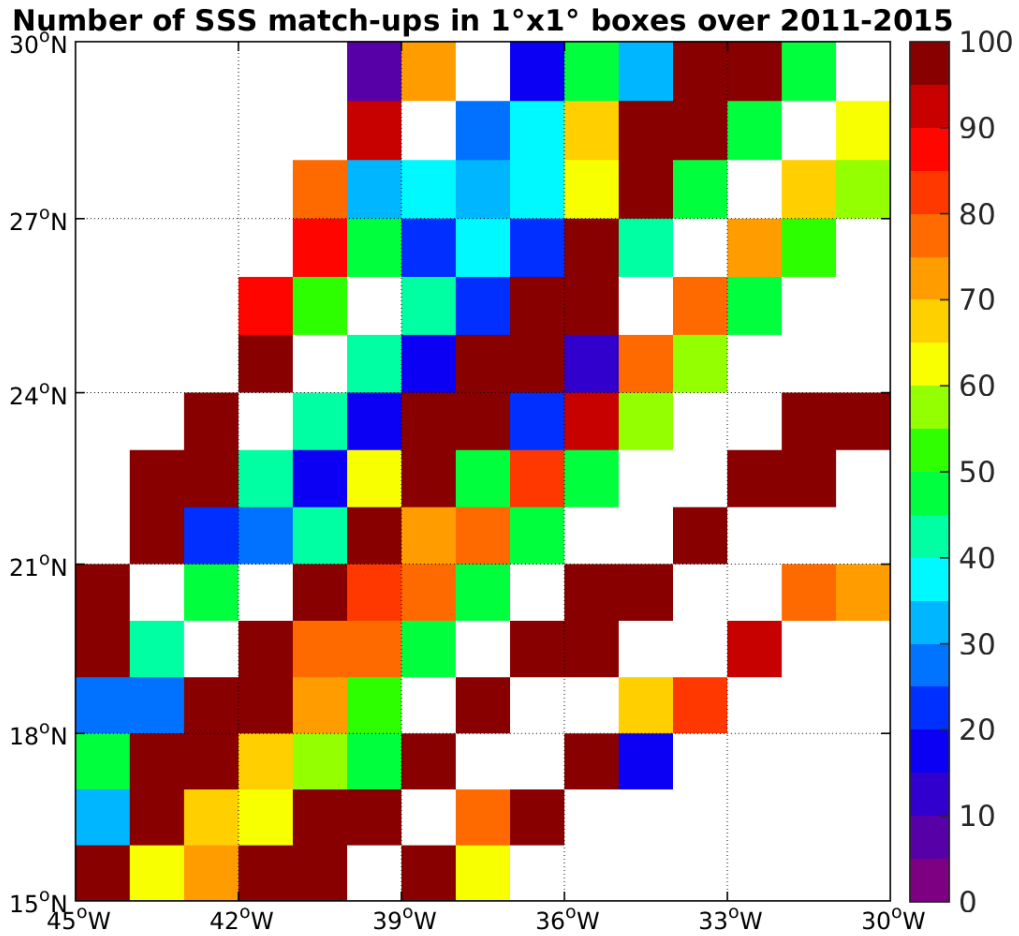
Figure 4: Number of SSS match-ups between TSG-LEGOS-DM SSS and the Aquarius-L3-JPL-V4-7DAY-RUNNING SSS product for the SPURS 1 Pi-MEP region over 1°x1° boxes and for the full satellite product period.
