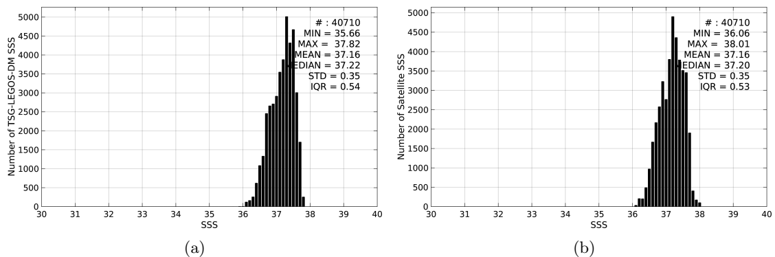
Figure 2: Histograms of SSS from TSG-LEGOS-DM (a) and Aquarius-L3-JPL-V4-7DAY-RUNNING (b) considering all match-up pairs per bins of 0.1 over the SPURS 1 Pi-MEP region and for the full satellite product period.
