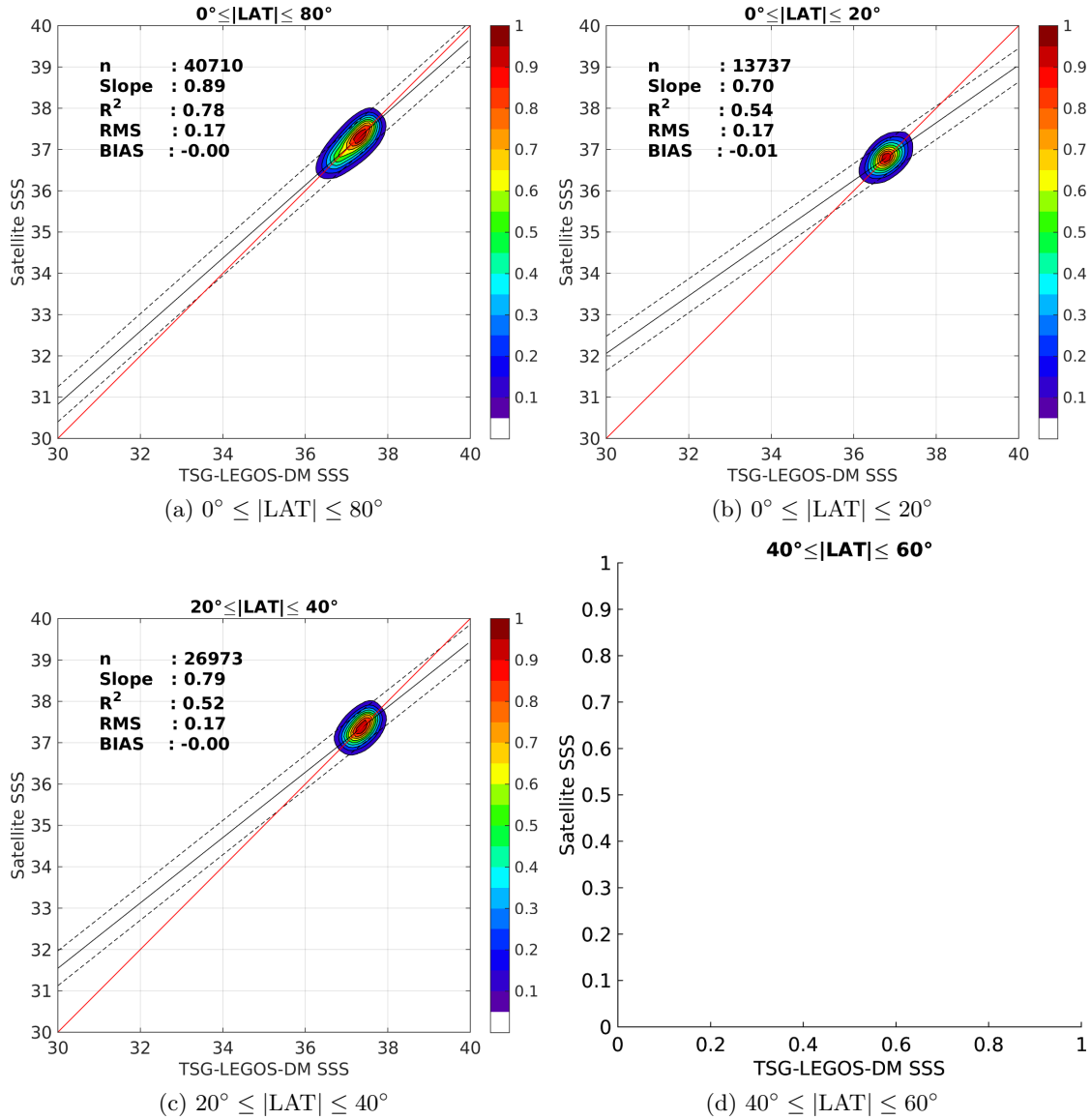
Figure 9: Contour maps of the concentration of Aquarius-L3-JPL-V4-7DAY-RUNNING SSS (y-axis) versus TSG-LEGOS-DM SSS (x-axis) at match-up pairs for different latitude bands. For each plot, the red line shows x=y . The black thin and dashed lines indicate a linear fit through the data cloud and the \pm 95\% confidence levels, respectively. The number match-up pairs n , the slope and R^2 coefficient of the linear fit, the root mean square (RMS) and the mean bias between satellite and in situ data are indicated for each latitude band in each plots.
