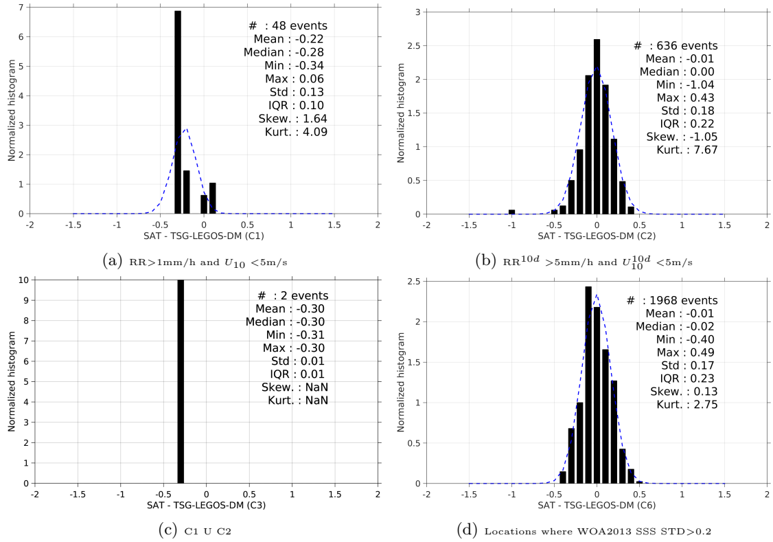
Figure 13: Normalized histogram of \Delta\text{SSS} (Aquarius-L3-JPL-V4-7DAY-RUNNING - TSG-LEGOS-DM) for 6 different subdatasets corresponding to: RR > 1mm/h and U_{10} < 5\text{m/s} (a), RR^{10d} > 5\text{mm/h} and U_{10}^{10d} < 5\text{m/s} (b), C1 U C2 (c), Locations where WOA2013 SSS STD > 0.2 (d).
