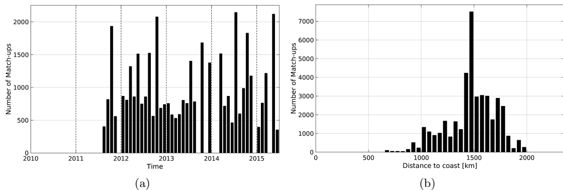
Figure 1: Number of match-ups between TSG-LEGOS-DM and Aquarius-L3-JPL-V4-7DAY-RUNNING SSS as a function of time (a) and as function of the distance to coast (b) over the SPURS 1 Pi-MEP region and for the full satellite product period.
