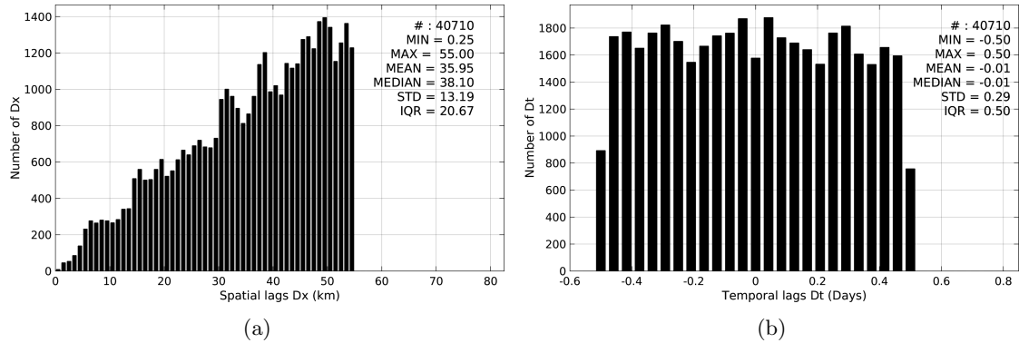
Figure 5: Histograms of the spatial (a) and temporal (b) lags between the time of the TSG-LEGOS-DM measurements and the date of the corresponding Aquarius-L3-JPL-V4-7DAY-RUNNING SSS product.
