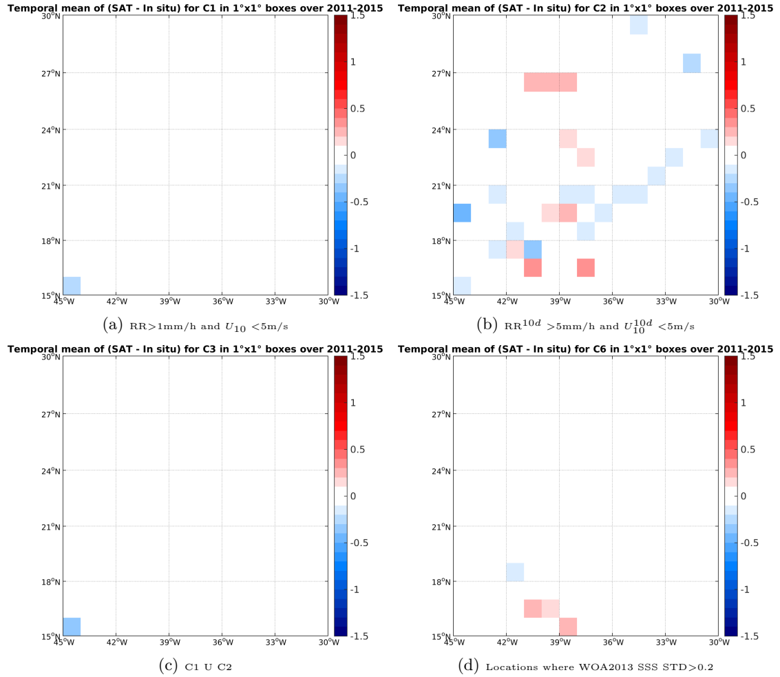
Figure 12: Temporal mean gridded over spatial boxes of size 1^\circ \times 1^\circ of \Delta SSS (Aquarius-L3-JPL-V4-7DAY-RUNNING - TSG-LEGOS-DM) for 4 different subdatasets corresponding to: RR > 1 mm/h and U_{10} < 5 m/s (a), RR^{10d} > 5 mm/h and U_{10}^{10d} < 5 m/s (b), C1 U C2 (c), Locations where WOA2013 SSS STD > 0.2 (d).
