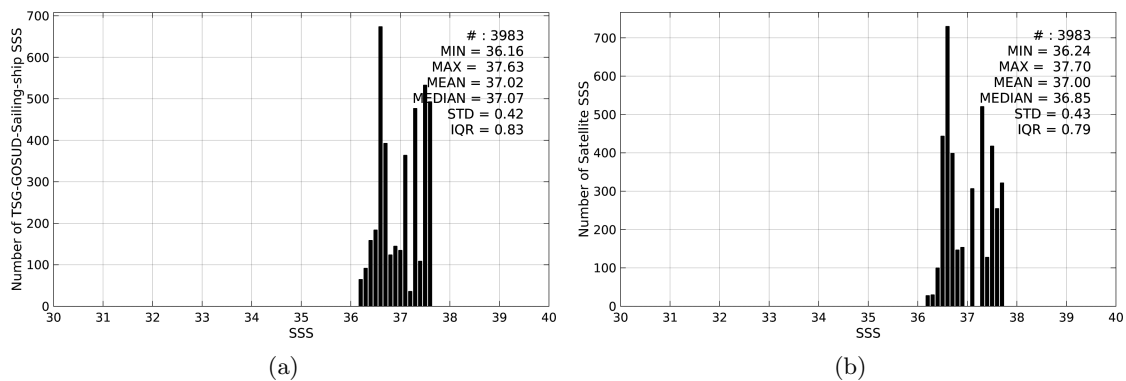
Figure 2: Histograms of SSS from TSG-GOSUD-Sailing-ship (a) and Aquarius-L3-JPL-V4-7DAY-RUNNING (b) considering all match-up pairs per bins of 0.1 over the SPURS 1 Pi-MEP region and for the full satellite product period.
