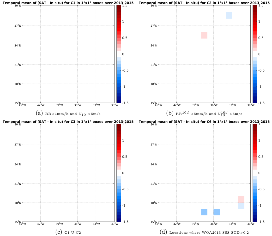
Figure 12: Temporal mean gridded over spatial boxes of size 1^\circ \times 1^\circ of \Delta SSS (Aquarius-L3-JPL-V4-7DAY-RUNNING - TSG-GOSUD-Sailing-ship) for 4 different subdatasets corresponding to: RR > 1\text{mm/h} and U_{10} < 5\text{m/s} (a), RR^{10d} > 5\text{mm/h} and U_{10}^{10d} < 5\text{m/s} (b), C1 U C2 (c), Locations where WOA2013 SSS STD > 0.2 (d).
