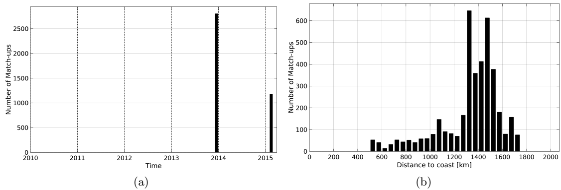
Figure 1: Number of match-ups between TSG-GOSUD-Sailing-ship and Aquarius-L3-JPL-V4-7DAY-RUNNING SSS as a function of time (a) and as function of the distance to coast (b) over the SPURS 1 Pi-MEP region and for the full satellite product period.
