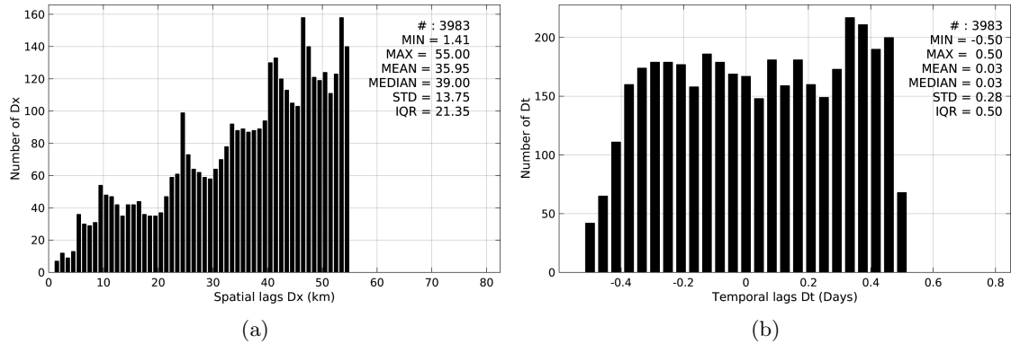
Figure 5: Histograms of the spatial (a) and temporal (b) lags between the time of the TSG-GOSUD-Sailing-ship measurements and the date of the corresponding Aquarius-L3-JPL-V4-7DAY-RUNNING SSS product.
