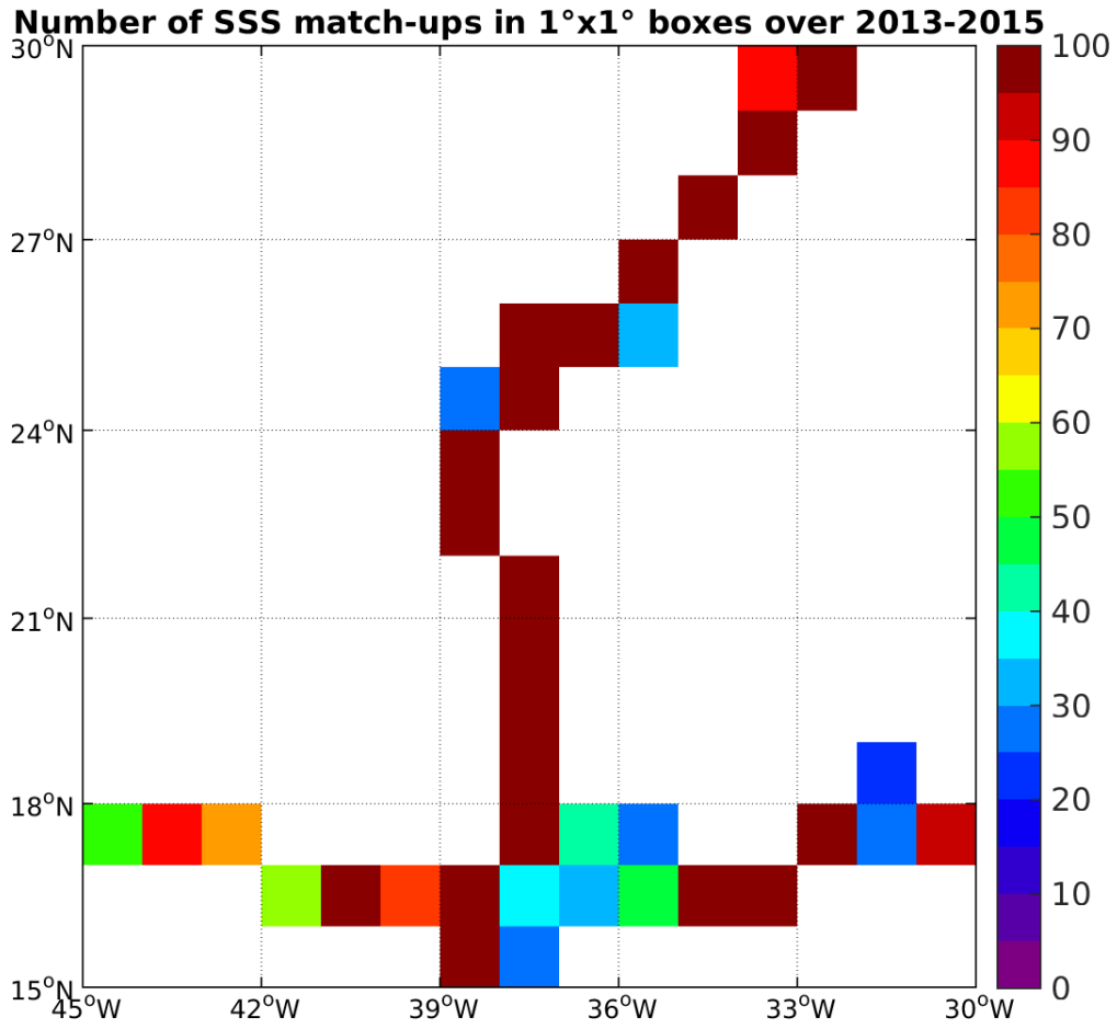
Figure 4: Number of SSS match-ups between TSG-GOSUD-Sailing-ship SSS and the Aquarius-L3-JPL-V4-7DAY-RUNNING SSS product for the SPURS 1 Pi-MEP region over 1°x1° boxes and for the full satellite product period.
