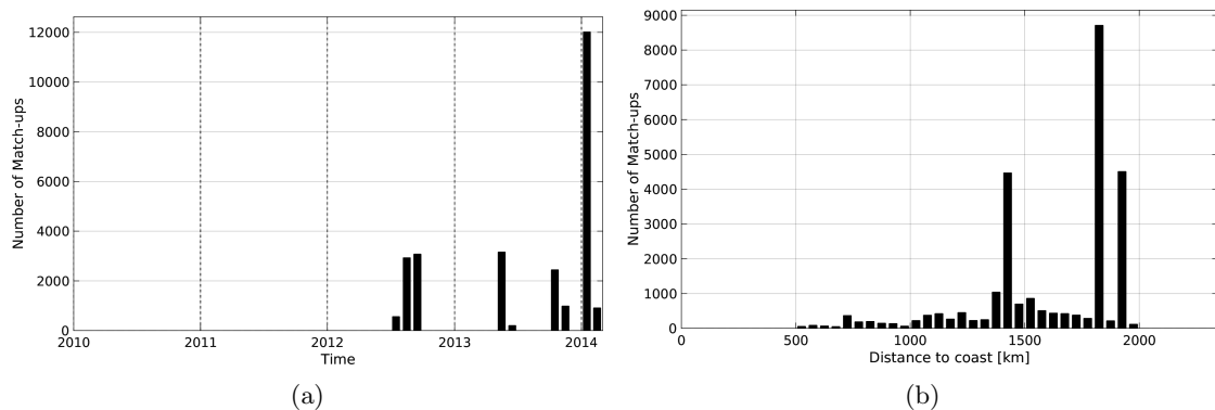
Figure 1: Number of match-ups between TSG-GOSUD-Research-vessel and Aquarius-L3-JPL-V4-7DAY-RUNNING SSS as a function of time (a) and as function of the distance to coast (b) over the SPURS 1 Pi-MEP region and for the full satellite product period.
