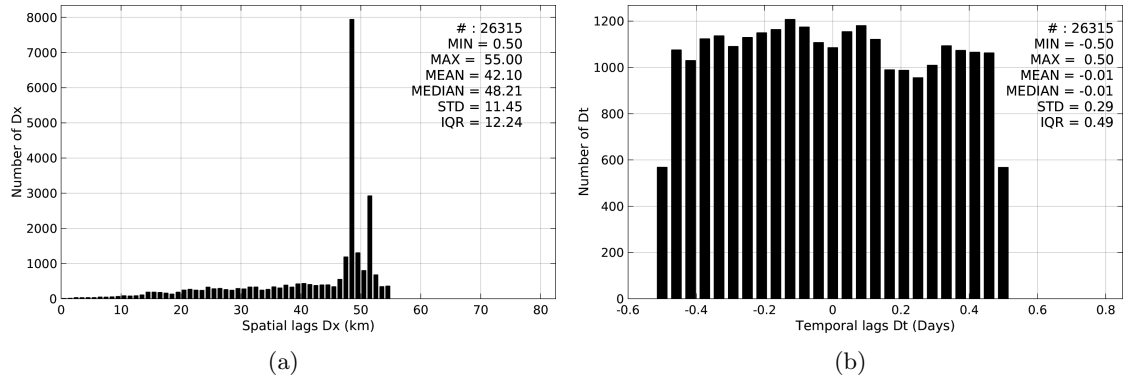
Figure 5: Histograms of the spatial (a) and temporal (b) lags between the time of the TSG-GOSUD-Research-vessel measurements and the date of the corresponding Aquarius-L3-JPL-V4-7DAY-RUNNING SSS product.
