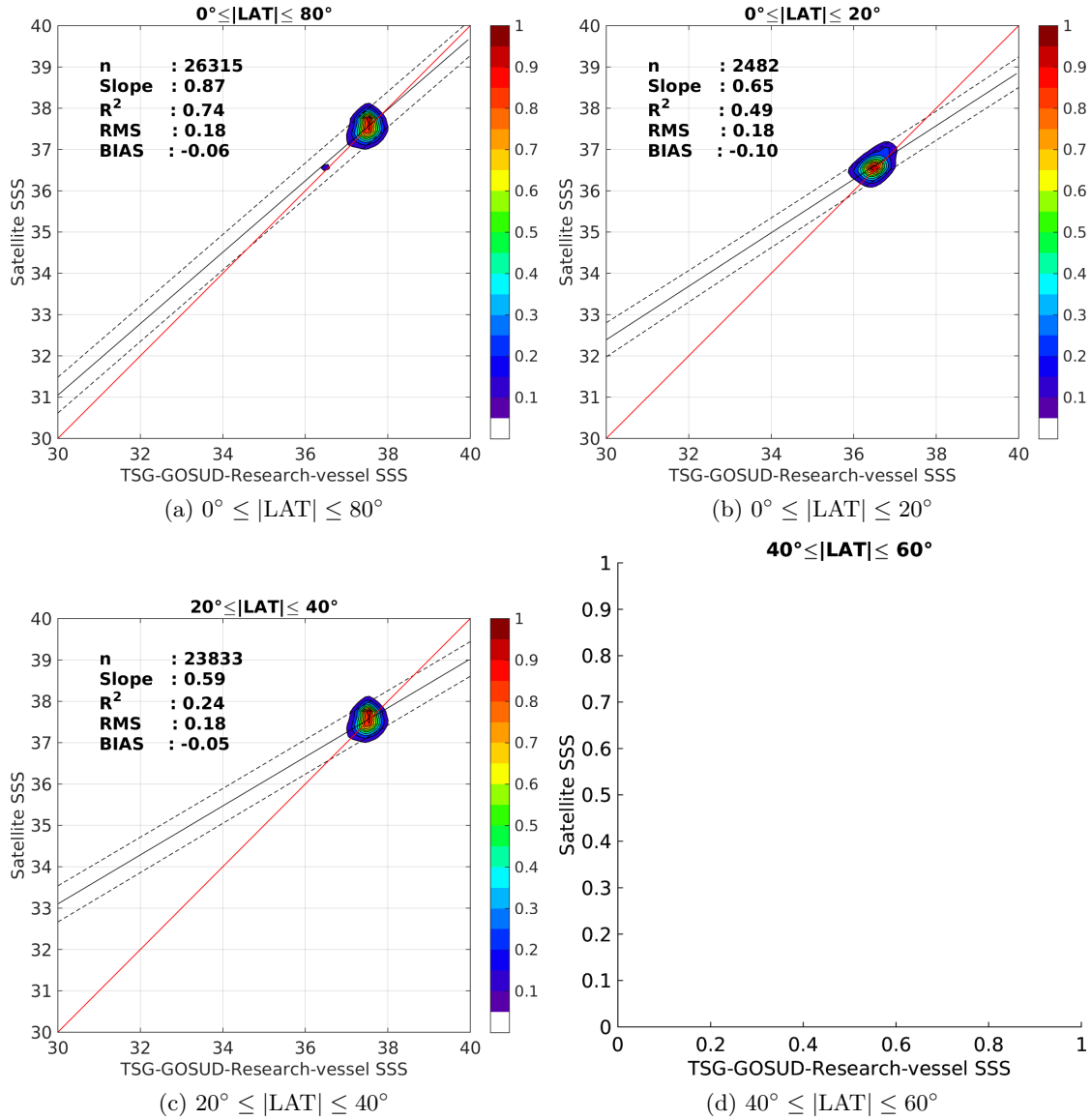
Figure 9: Contour maps of the concentration of Aquarius-L3-JPL-V4-7DAY-RUNNING SSS (y-axis) versus TSG-GOSUD-Research-vessel SSS (x-axis) at match-up pairs for different latitude bands. For each plot, the red line shows x=y . The black thin and dashed lines indicate a linear fit through the data cloud and the \pm 95\% confidence levels, respectively. The number match-up pairs n , the slope and R^2 coefficient of the linear fit, the root mean square (RMS) and the mean bias between satellite and in situ data are indicated for each latitude band in each plots.
