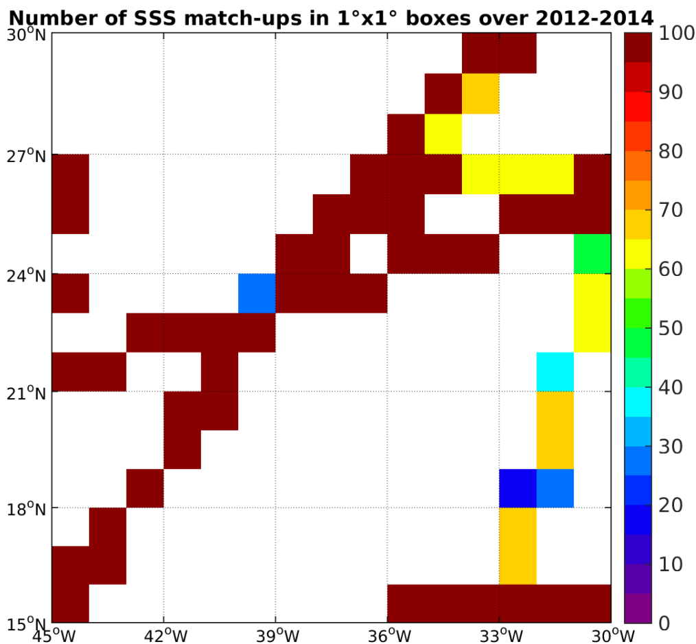
Figure 4: Number of SSS match-ups between TSG-GOSUD-Research-vessel SSS and the Aquarius-L3-JPL-V4-7DAY-RUNNING SSS product for the SPURS 1 Pi-MEP region over 1°x1° boxes and for the full satellite product period.
