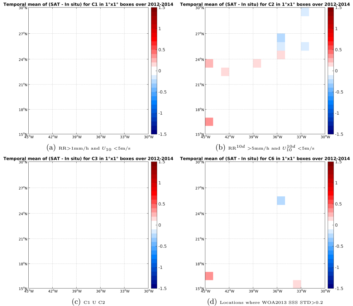
Figure 12: Temporal mean gridded over spatial boxes of size 1^\circ \times 1^\circ of \Delta SSS (Aquarius-L3-JPL-V4-7DAY-RUNNING - TSG-GOSUD-Research-vessel) for 4 different subdatasets corresponding to: RR > 1 mm/h and U_{10} < 5 m/s (a), RR 10d > 5 mm/h and U_{10}^{10d} < 5 m/s (b), C1 U C2 (c), Locations where WOA2013 SSS STD > 0.2 (d).
