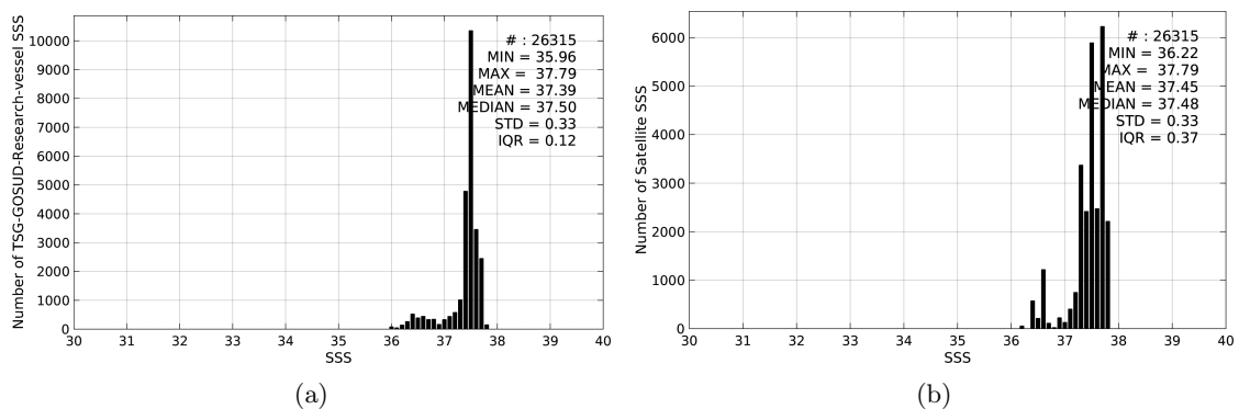
Figure 2: Histograms of SSS from TSG-GOSUD-Research-vessel (a) and Aquarius-L3-JPL-V4-7DAY-RUNNING (b) considering all match-up pairs per bins of 0.1 over the SPURS 1 Pi-MEP region and for the full satellite product period.
