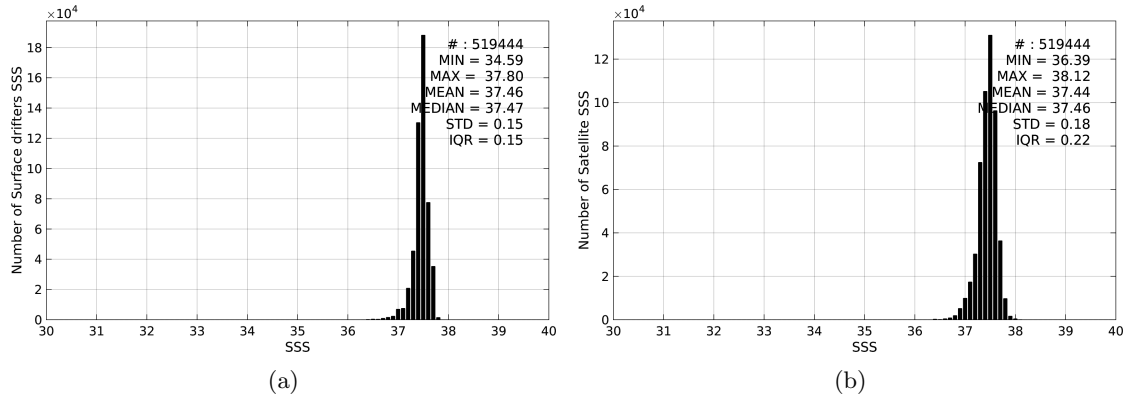
Figure 2: Histograms of SSS from Surface drifters (a) and Aquarius-L3-JPL-V4-7DAY-RUNNING (b) considering all match-up pairs per bins of 0.1 over the SPURS 1 Pi-MEP region and for the full satellite product period.
