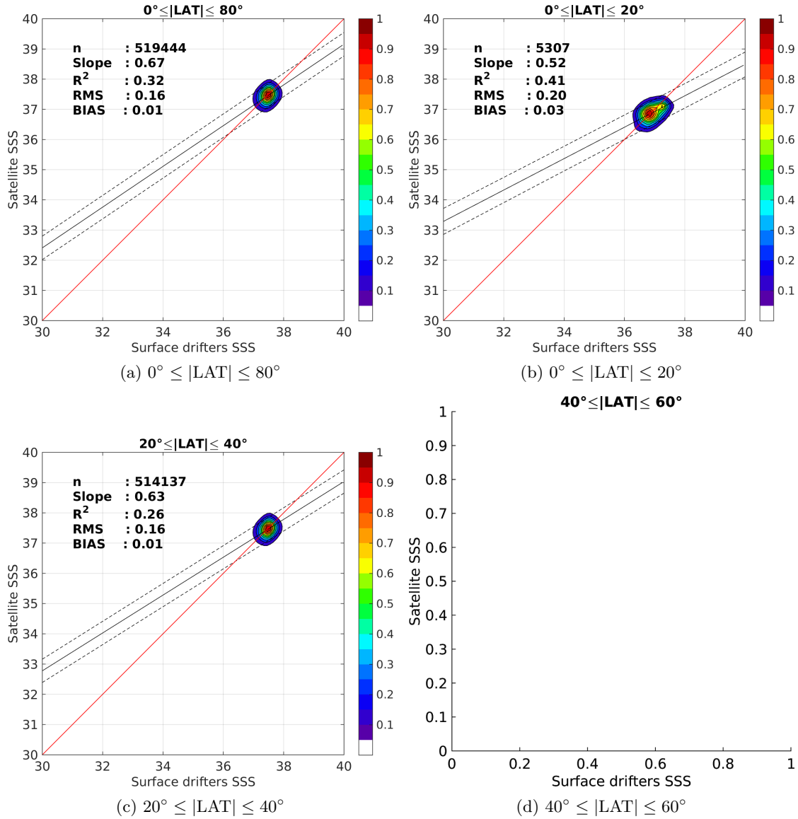
Figure 8: Contour maps of the concentration of Aquarius-L3-JPL-V4-7DAY-RUNNING SSS (y-axis) versus Surface drifters SSS (x-axis) at match-up pairs for different latitude bands. For each plot, the red line shows x=y . The black thin and dashed lines indicate a linear fit through the data cloud and the \pm 95\% confidence levels, respectively. The number match-up pairs n , the slope and R^2 coefficient of the linear fit, the root mean square (RMS) and the mean bias between satellite and in situ data are indicated for each latitude band in each plots.
