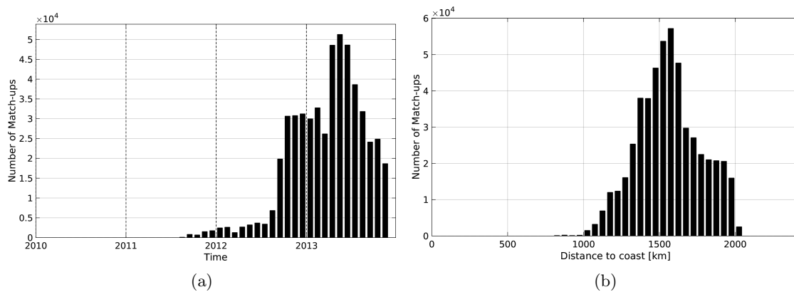
Figure 1: Number of match-ups between Surface drifters and Aquarius-L3-JPL-V4-7DAY-RUNNING SSS as a function of time (a) and as function of the distance to coast (b) over the SPURS 1 Pi-MEP region and for the full satellite product period.
