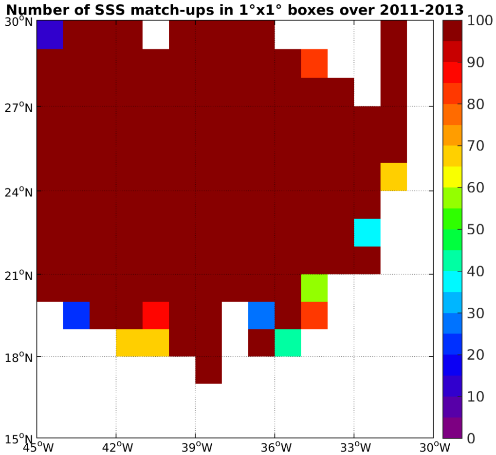
Figure 3: Number of SSS match-ups between Surface drifters SSS and the Aquarius-L3-JPL-V4-7DAY-RUNNING SSS product for the SPURS 1 Pi-MEP region over 1°x1° boxes and for the full satellite product period.
