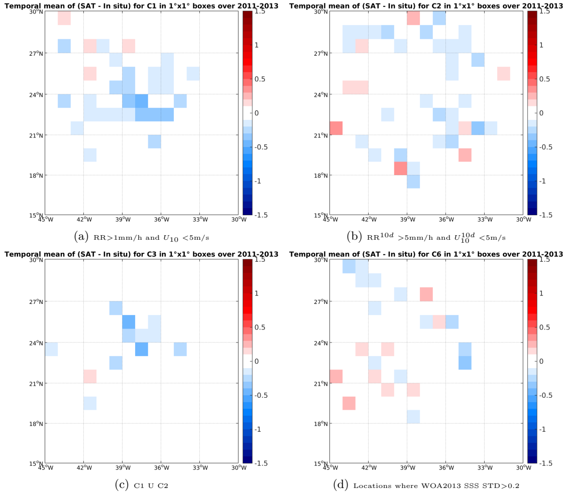
Figure 11: Temporal mean gridded over spatial boxes of size 1°x1° of \Delta SSS (Aquarius-L3-JPL-V4-7DAY-RUNNING - Surface drifters) for 4 different subdatasets corresponding to: RR > 1\text{mm/h} and U_{10} < 5\text{m/s} (a), RR^{10d} > 5\text{mm/h} and U_{10}^{10d} < 5\text{m/s} (b), C1 U C2 (c), Locations where WOA2013 SSS STD > 0.2 (d).
