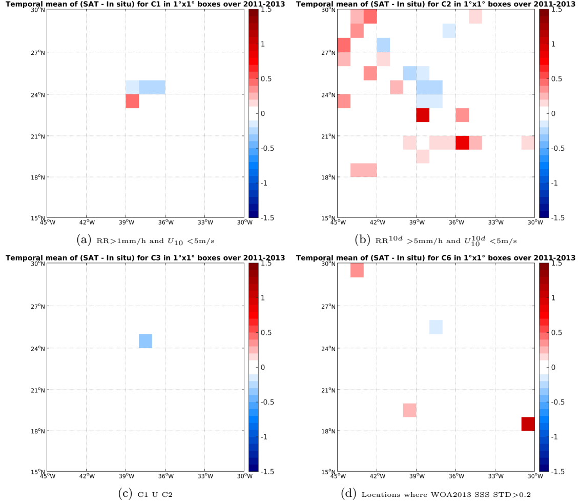
Figure 12: Temporal mean gridded over spatial boxes of size 1^\circ \times 1^\circ of \Delta SSS (Aquarius-L3-JPL-V4-MONTHLY - TSG-SAMOS) for 4 different subdatasets corresponding to: RR > 1mm/h and U_{10} < 5 m/s (a), RR 10d > 5mm/h and U_{10}^{10d} < 5 m/s (b), C1 U C2 (c), Locations where WOA2013 SSS STD > 0.2 (d).
