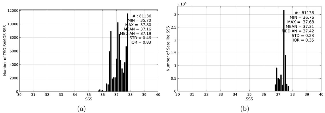
Figure 2: Histograms of SSS from TSG-SAMOS (a) and Aquarius-L3-JPL-V4-MONTHLY (b) considering all match-up pairs per bins of 0.1 over the SPURS 1 Pi-MEP region and for the full satellite product period.
