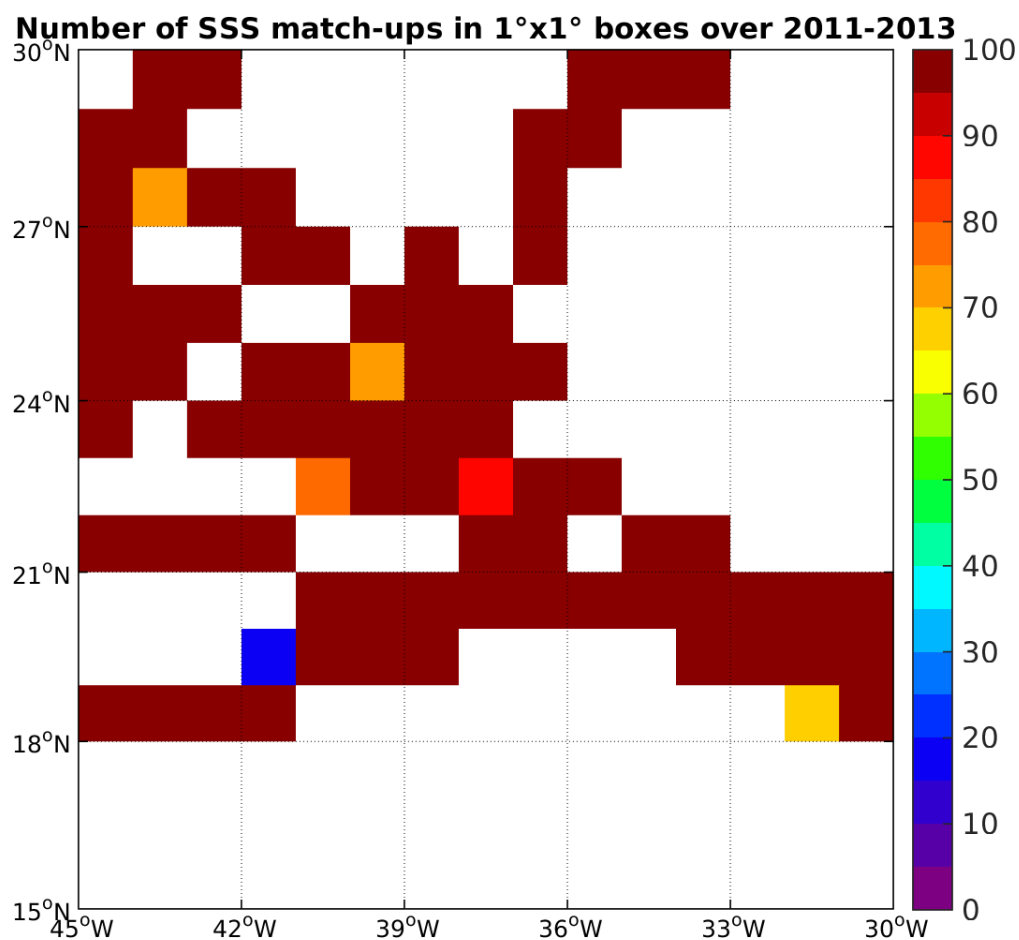
Figure 4: Number of SSS match-ups between TSG-SAMOS SSS and the Aquarius-L3-JPL-V4-MONTHLY SSS product for the SPURS 1 Pi-MEP region over 1°x1° boxes and for the full satellite product period.
