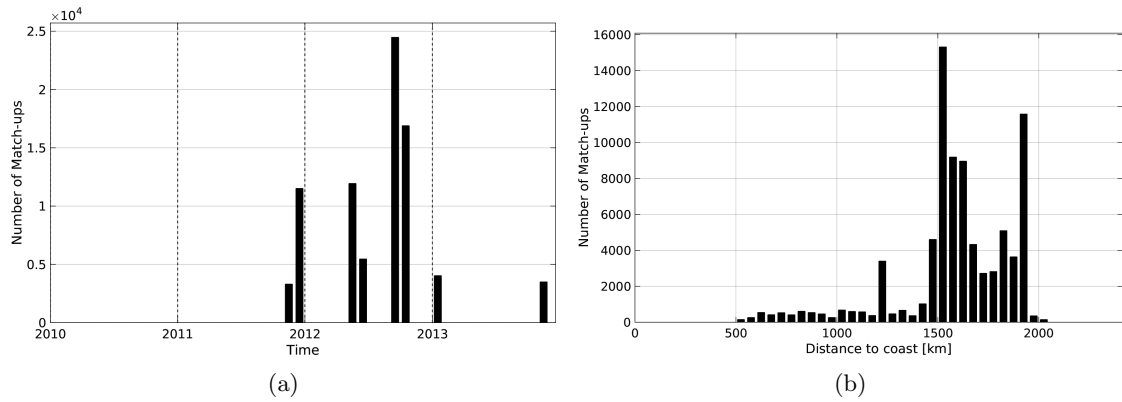
Figure 1: Number of match-ups between TSG-SAMOS and Aquarius-L3-JPL-V4-MONTHLY SSS as a function of time (a) and as function of the distance to coast (b) over the SPURS 1 Pi-MEP region and for the full satellite product period.
