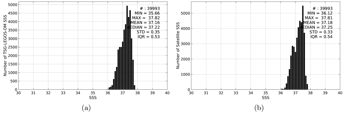
Figure 2: Histograms of SSS from TSG-LEGOS-DM (a) and Aquarius-L3-JPL-V4-MONTHLY (b) considering all match-up pairs per bins of 0.1 over the SPURS 1 Pi-MEP region and for the full satellite product period.
