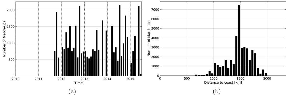
Figure 1: Number of match-ups between TSG-LEGOS-DM and Aquarius-L3-JPL-V4-MONTHLY SSS as a function of time (a) and as function of the distance to coast (b) over the SPURS 1 Pi-MEP region and for the full satellite product period.
