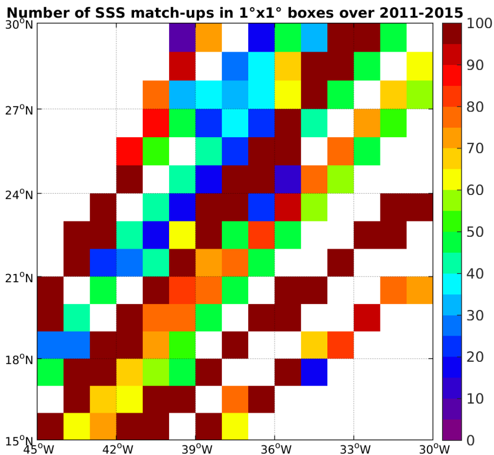
Figure 4: Number of SSS match-ups between TSG-LEGOS-DM SSS and the Aquarius-L3-JPL-V4-MONTHLY SSS product for the SPURS 1 Pi-MEP region over 1°x1° boxes and for the full satellite product period.
