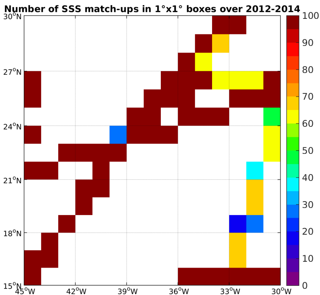
Figure 4: Number of SSS match-ups between TSG-GOSUD-Research-vessel SSS and the Aquarius-L3-JPL-V4-MONTHLY SSS product for the SPURS 1 Pi-MEP region over 1°x1° boxes and for the full satellite product period.
