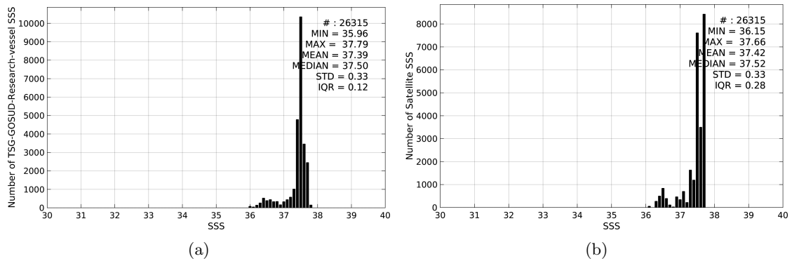
Figure 2: Histograms of SSS from TSG-GOSUD-Research-vessel (a) and Aquarius-L3-JPL-V4-MONTHLY (b) considering all match-up pairs per bins of 0.1 over the SPURS 1 Pi-MEP region and for the full satellite product period.
