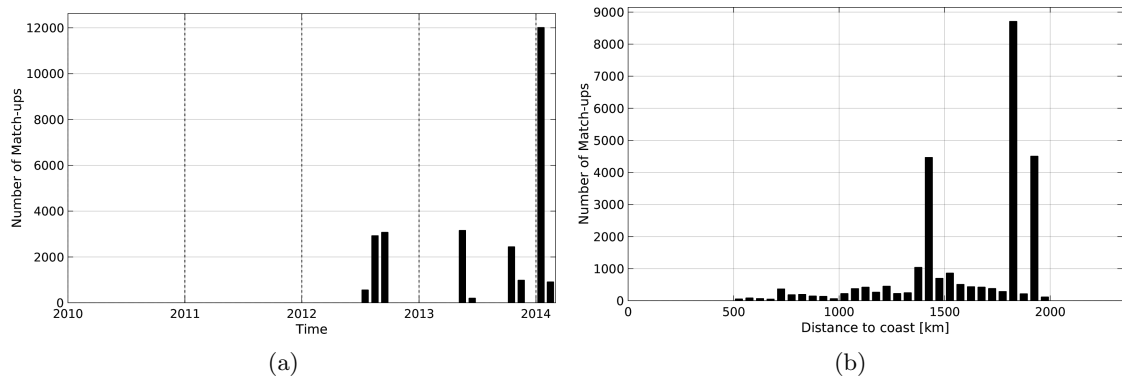
Figure 1: Number of match-ups between TSG-GOSUD-Research-vessel and Aquarius-L3-JPL-V4-MONTHLY SSS as a function of time (a) and as function of the distance to coast (b) over the SPURS 1 Pi-MEP region and for the full satellite product period.
