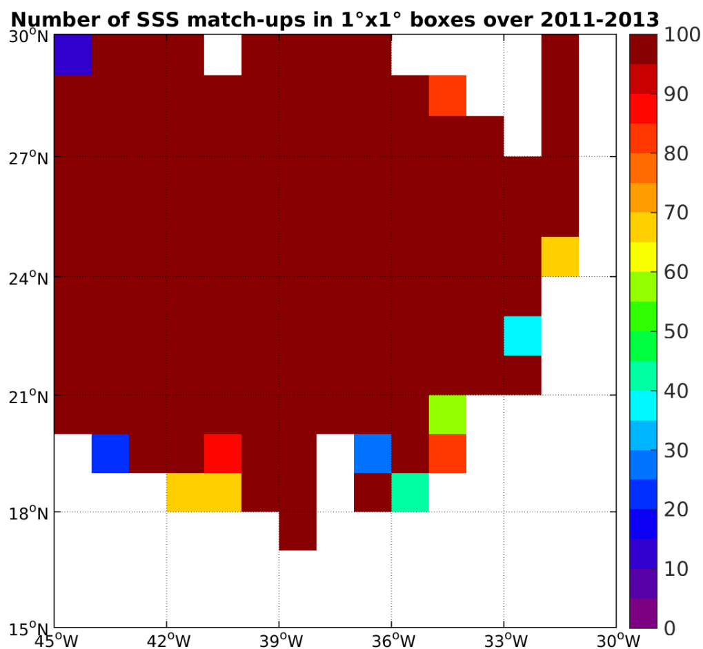
Figure 3: Number of SSS match-ups between Surface drifters SSS and the Aquarius-L3-JPL-V4-MONTHLY SSS product for the SPURS 1 Pi-MEP region over 1°x1° boxes and for the full satellite product period.
