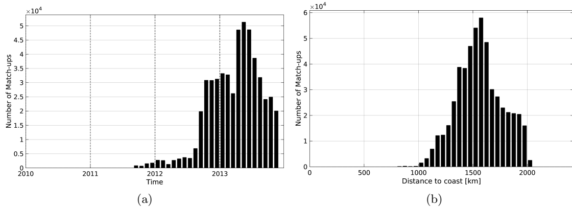
Figure 1: Number of match-ups between Surface drifters and Aquarius-L3-JPL-V4-MONTHLY SSS as a function of time (a) and as function of the distance to coast (b) over the SPURS 1 Pi-MEP region and for the full satellite product period.
