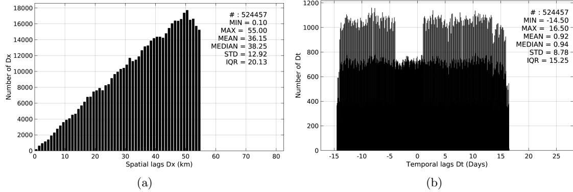
Figure 4: Histograms of the spatial (a) and temporal (b) lags between the time of the Surface drifters measurements and the date of the corresponding Aquarius-L3-JPL-V4-MONTHLY SSS product.
