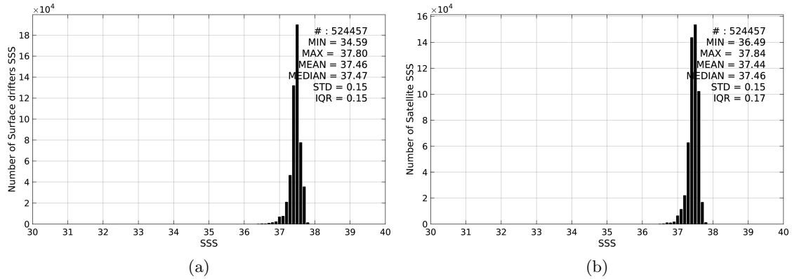
Figure 2: Histograms of SSS from Surface drifters (a) and Aquarius-L3-JPL-V4-MONTHLY (b) considering all match-up pairs per bins of 0.1 over the SPURS 1 Pi-MEP region and for the full satellite product period.
