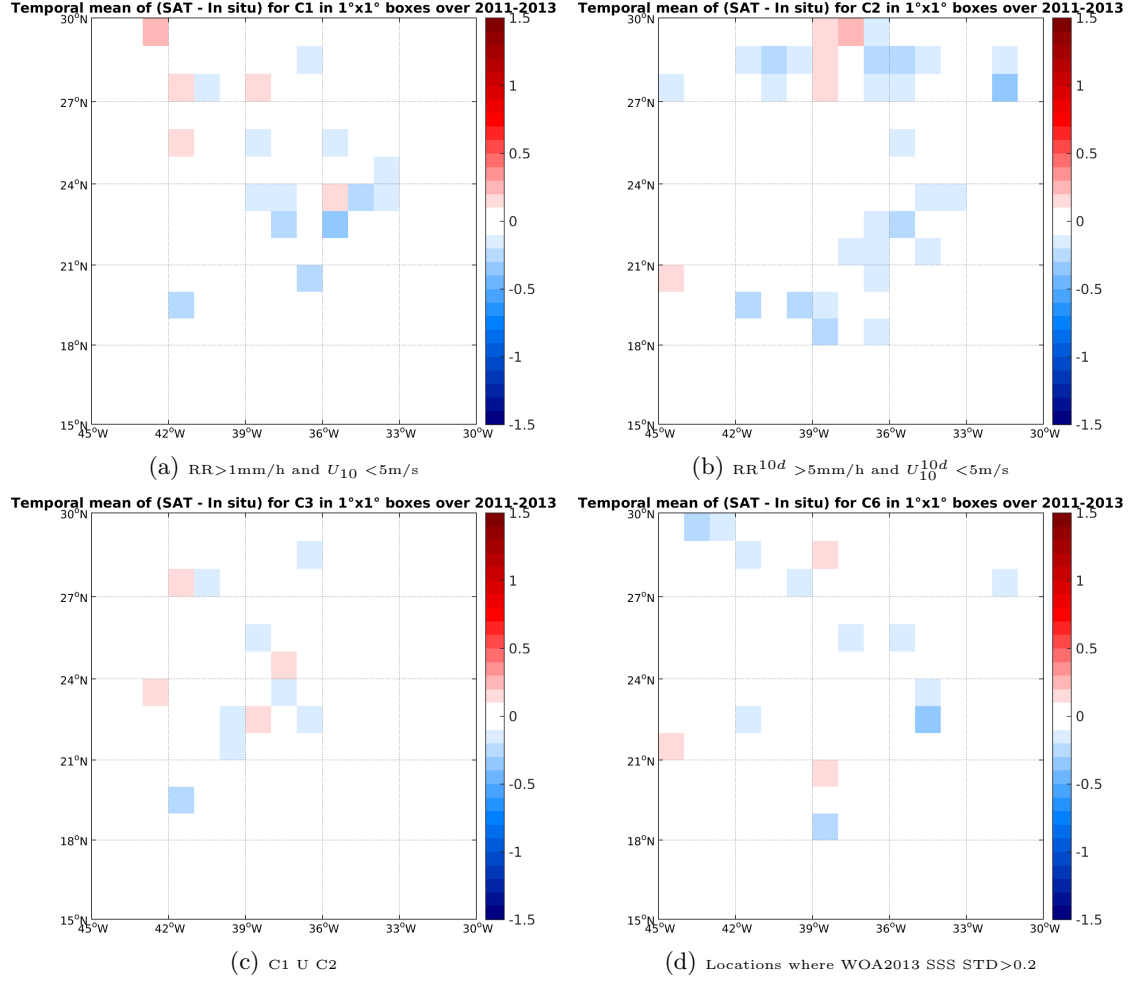
Figure 11: Temporal mean gridded over spatial boxes of size 1^\circ \times 1^\circ of \Delta SSS (Aquarius-L3-JPL-V4-MONTHLY - Surface drifters) for 4 different subdatasets corresponding to: RR > 1 mm/h and U_{10} < 5 m/s (a), RR 10d > 5 mm/h and U_{10}^{10d} < 5 m/s (b), C1 U C2 (c), Locations where WOA2013 SSS STD > 0.2 (d).
