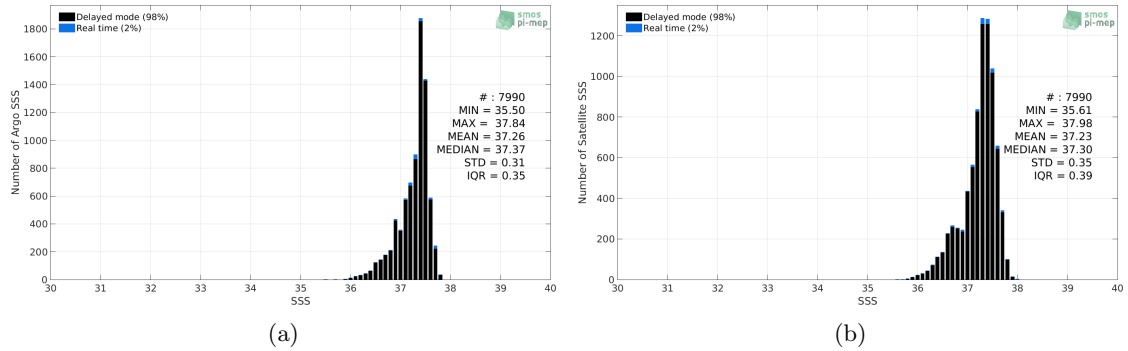
Figure 2: Histograms of SSS from Argo (a) and Aquarius SSS L2-AVERAGED OR v5 (NASA-GSFC) (b) considering all match-up pairs per bins of 0.1 over the SPURS 1 Pi-MEP region and for the full satellite product period.
