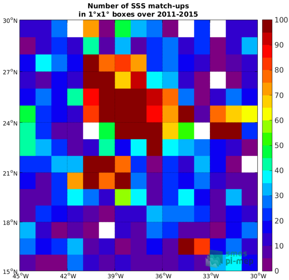
Figure 4: Number of SSS match-ups between Argo SSS and the Aquarius SSS L2-AVERAGED OR v5 (NASA-GSFC) SSS product for the SPURS 1 Pi-MEP region over 1°x1° boxes and for the full satellite product period.
