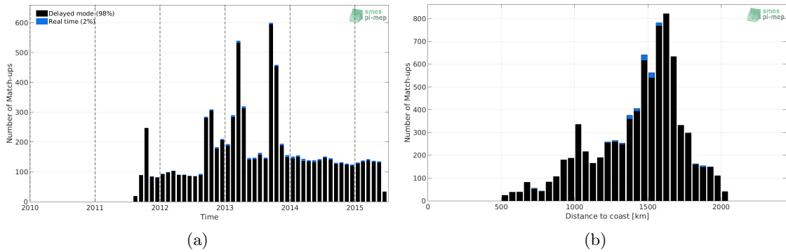
Figure 1: Number of match-ups between Argo and Aquarius SSS L2-AVERAGED OR v5 (NASA-GSFC) SSS as a function of time (a) and as function of the distance to coast (b) over the SPURS 1 Pi-MEP region and for the full satellite product period.
