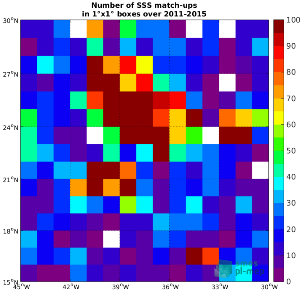
Figure 4: Number of SSS match-ups between Argo SSS and the Aquarius SSS L2-AVERAGED CAP v5 (JPL) SSS product for the SPURS 1 Pi-MEP region over 1°x1° boxes and for the full satellite product period.
