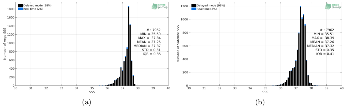
Figure 2: Histograms of SSS from Argo (a) and Aquarius SSS L2-AVERAGED CAP v5 (JPL) (b) considering all match-up pairs per bins of 0.1 over the SPURS 1 Pi-MEP region and for the full satellite product period.
