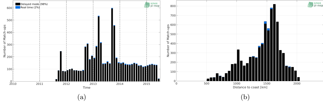
Figure 1: Number of match-ups between Argo and Aquarius SSS L2-AVERAGED CAP v5 (JPL) SSS as a function of time (a) and as function of the distance to coast (b) over the SPURS 1 Pi-MEP region and for the full satellite product period.
