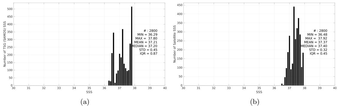
Figure 3: Histograms of SSS from TSG (SAMOS) (a) and Aquarius SSS L2 OR v5 (NASA-GSFC) (b) considering all match-up pairs per bins of 0.1 over the SPURS 1 Pi-MEP region and for the full satellite product period.
