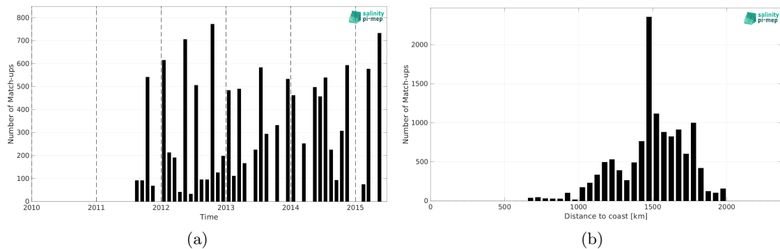
Figure 2: Number of match-ups between TSG (LEGOS-DM) and Aquarius SSS L2 OR v5 (NASA-GSFC) SSS as a function of time (a) and as function of the distance to coast (b) over the SPURS 1 Pi-MEP region and for the full satellite product period.
