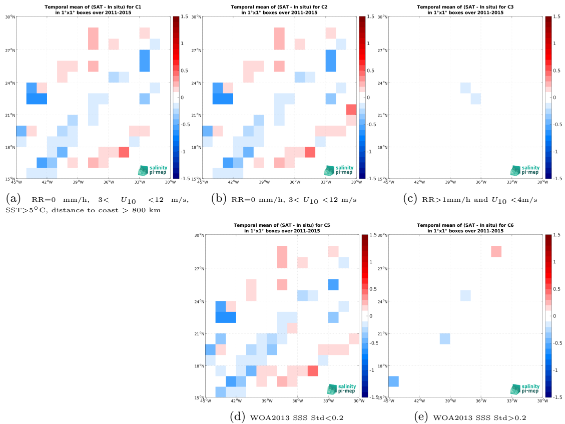
Figure 14: Temporal mean gridded over spatial boxes of size 1^\circ \times 1^\circ of \Delta SSS (Aquarius SSS L2 OR v5 (NASA-GSFC) - TSG (LEGOS-DM)) for 5 different subdatasets corresponding to: RR=0 mm/h, 3 < U_{10} < 12 m/s, SST > 5^\circ C , distance to coast > 800 km (a), RR=0 mm/h, 3 < U_{10} < 12 m/s (b), RR > 1 mm/h and U_{10} < 4 m/s (c), WOA2013 SSS Std < 0.2 (d), WOA2013 SSS Std > 0.2 (e).
