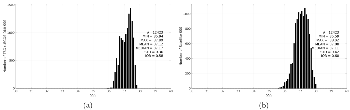
Figure 3: Histograms of SSS from TSG (LEGOS-DM) (a) and Aquarius SSS L2 OR v5 (NASA-GSFC) (b) considering all match-up pairs per bins of 0.1 over the SPURS 1 Pi-MEP region and for the full satellite product period.
