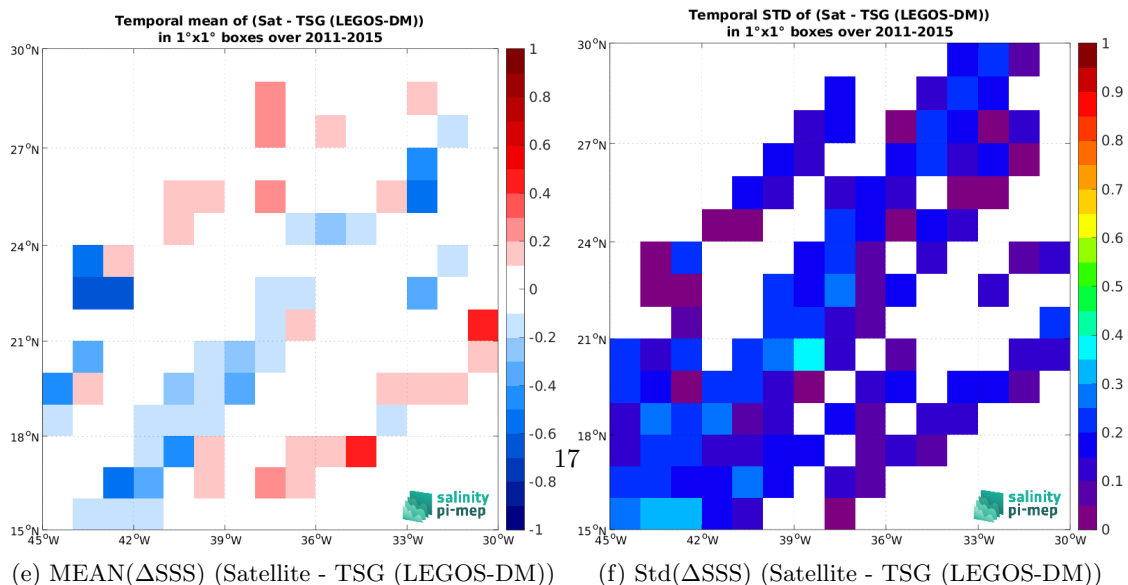
Figure 7: Temporal mean (left) and Std (right) of SSS from Aquarius SSS L2 OR v5 (NASA-GSFC) (top), TSG (LEGOS-DM) (middle), and of \Delta SSS (Satellite - TSG (LEGOS-DM)). Only match-up pairs are used to generate these maps.
