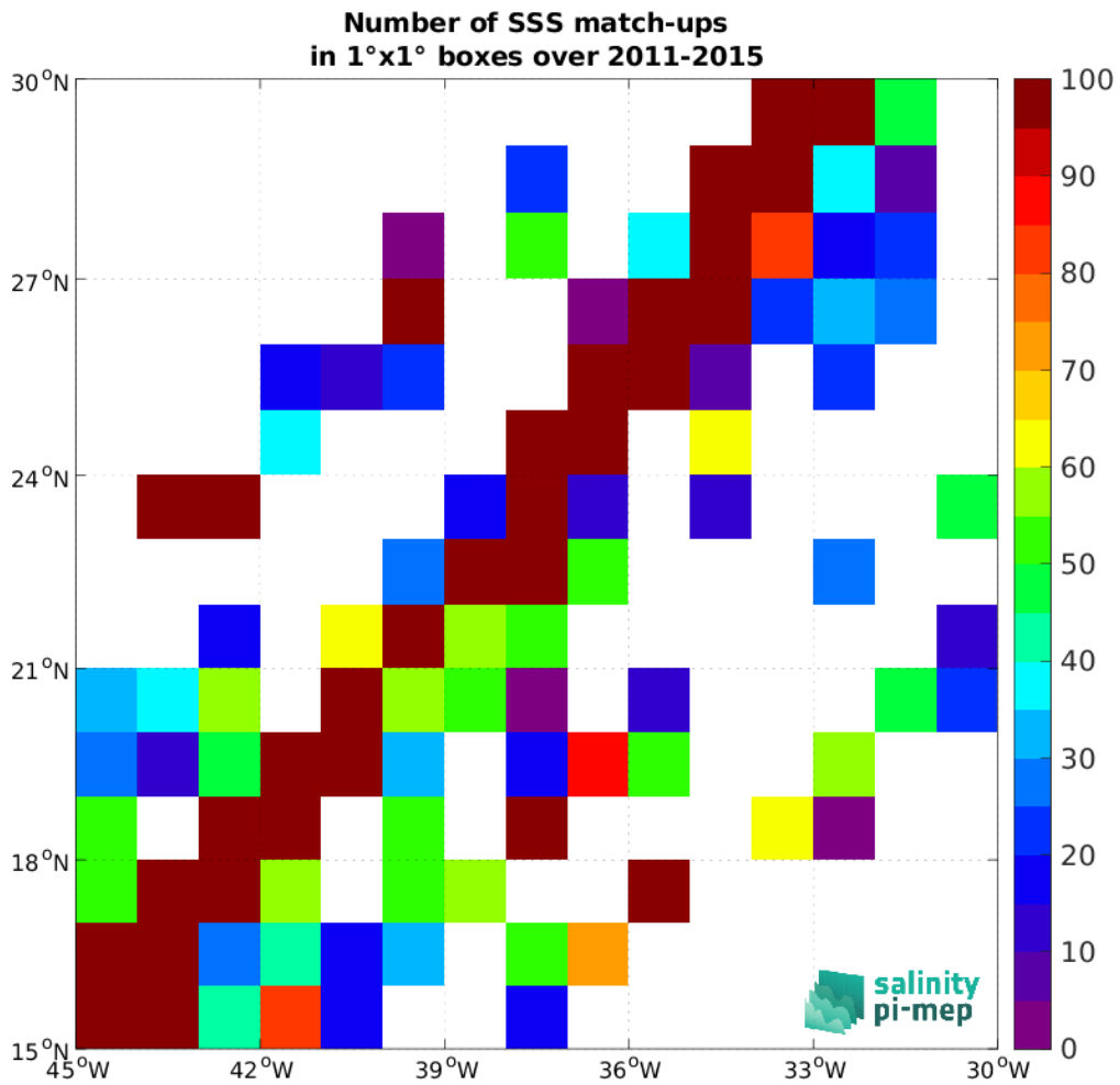
Figure 5: Number of SSS match-ups between TSG (LEGOS-DM) SSS and the Aquarius SSS L2 OR v5 (NASA-GSFC) SSS product for the SPURS 1 Pi-MEP region over 1^\circ \times 1^\circ boxes and for the full satellite product period.
